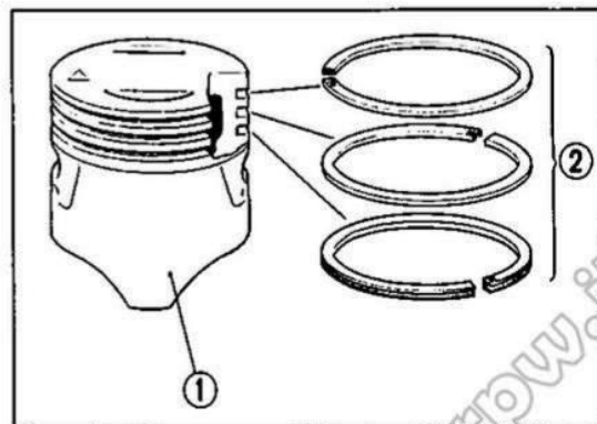
Fig. 3-63 ① Pistone.
