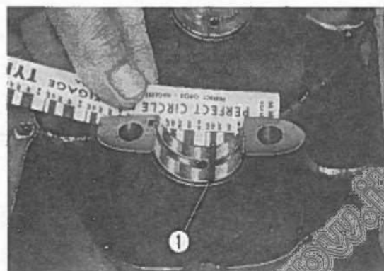
Fig. 3-92 ① Plastigage.
