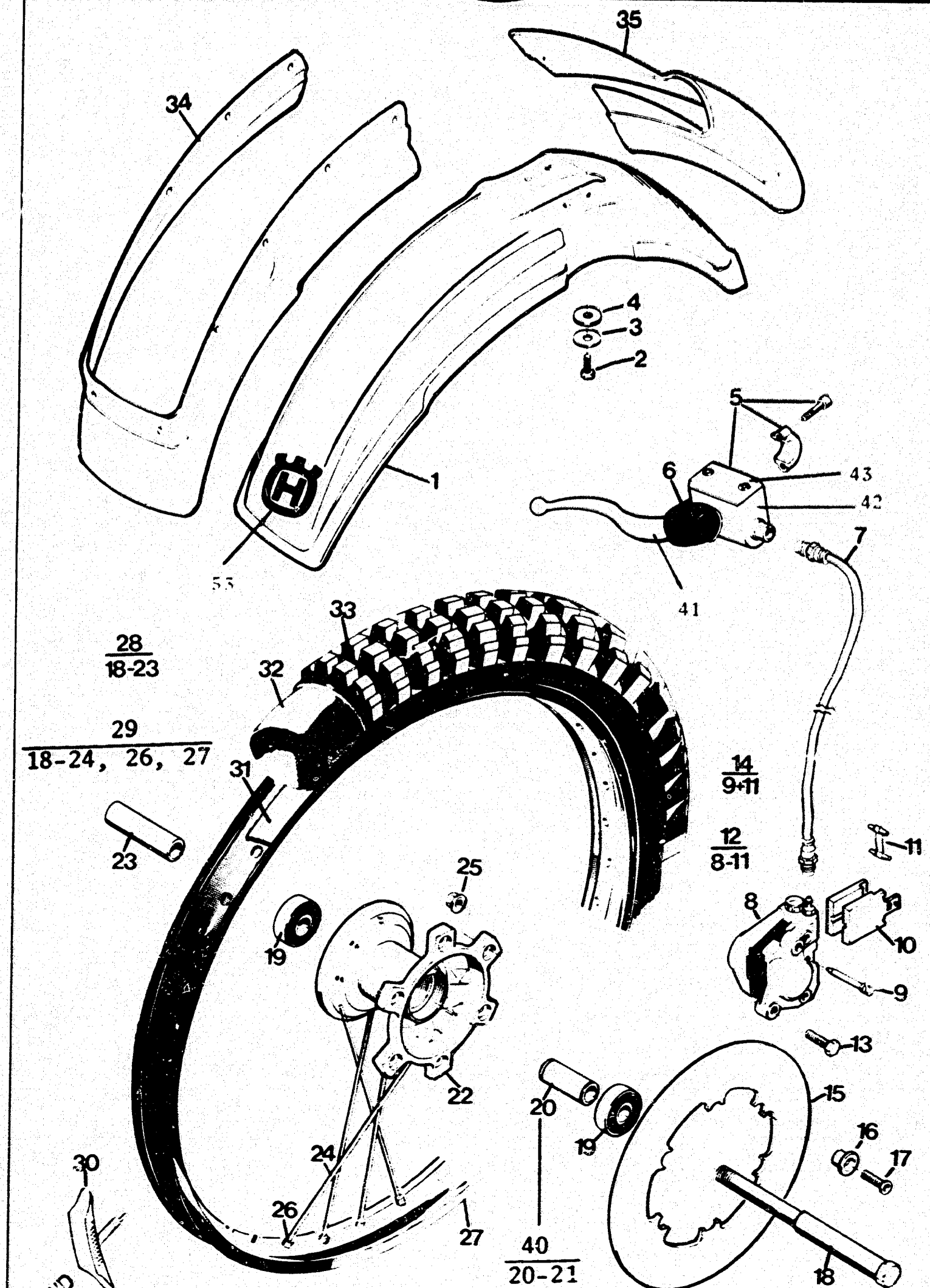
SPOKE KIT FIG. 36 NIPPLE KIT FIG. 37
