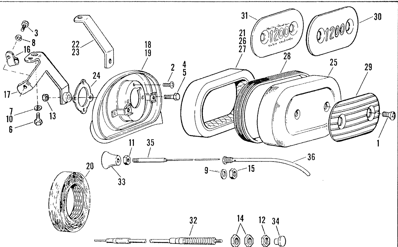
AIR CLEANER AND CHOKE 1971 TO EARLY 1978
