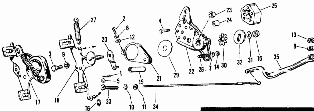
CLUTCH FOOT CONTROL 1978 & EARLIER
