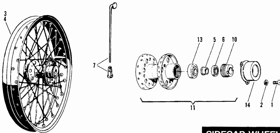
SIDECAR WHEEL — LE —
