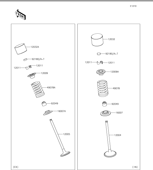
6 Valve(s)
