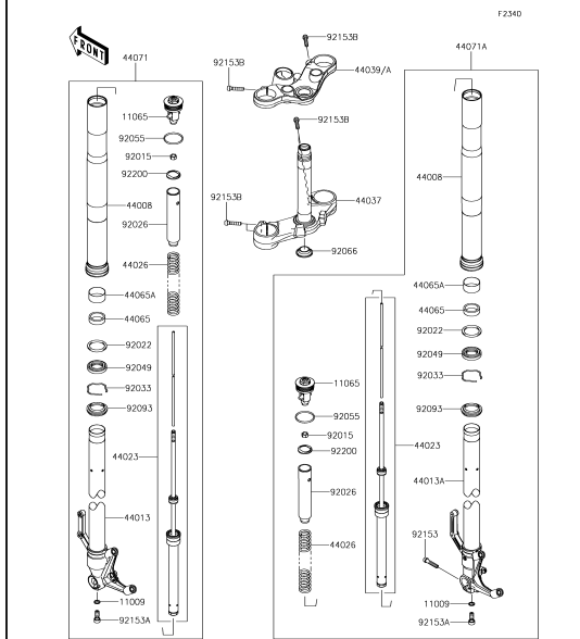
47 Front Fork
