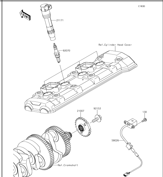
24 Ignition System
