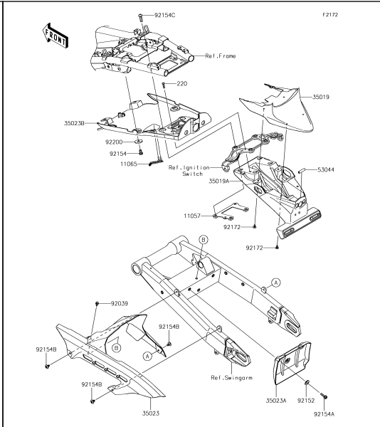
35 Rear Fender(s)
