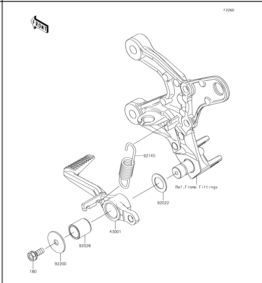
40 Brake Pedal
