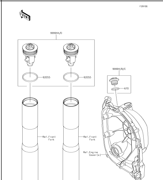
70 Accessory(Cap)
