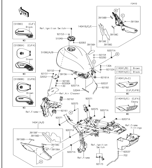
48 Fuel Tank
