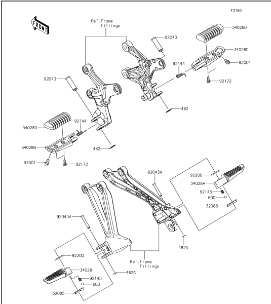
33 Footrests
