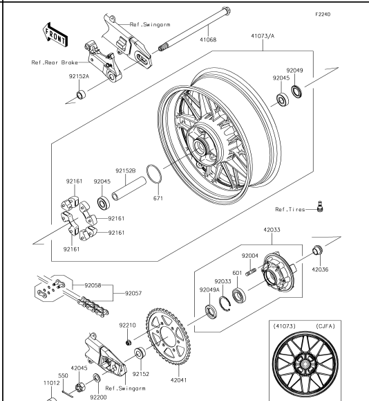
39 Rear Hub
