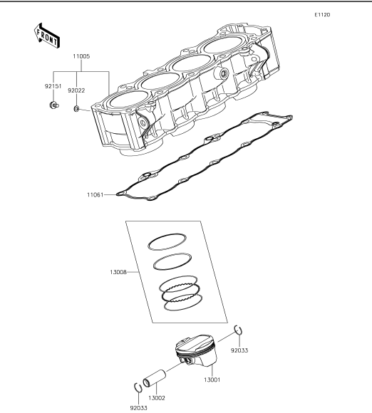
3 Cylinder/Piston(s)
