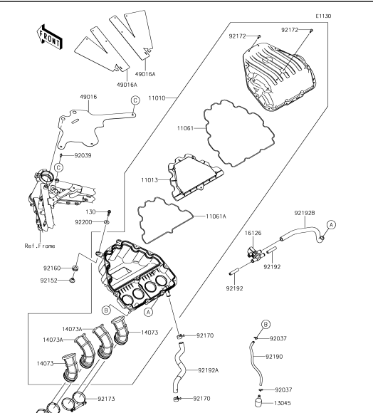
4 Air Cleaner
