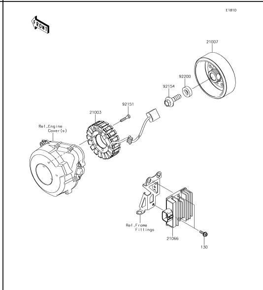
23 Generator
