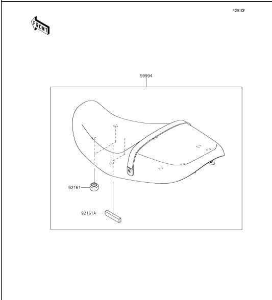
69 Accessory(Seat)
