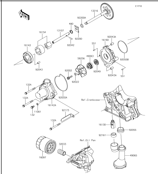
22 Oil Pump
