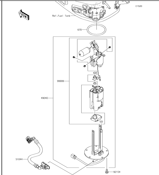
19 Fuel Pump
