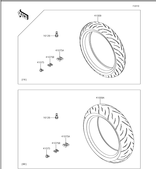
37 Tires
