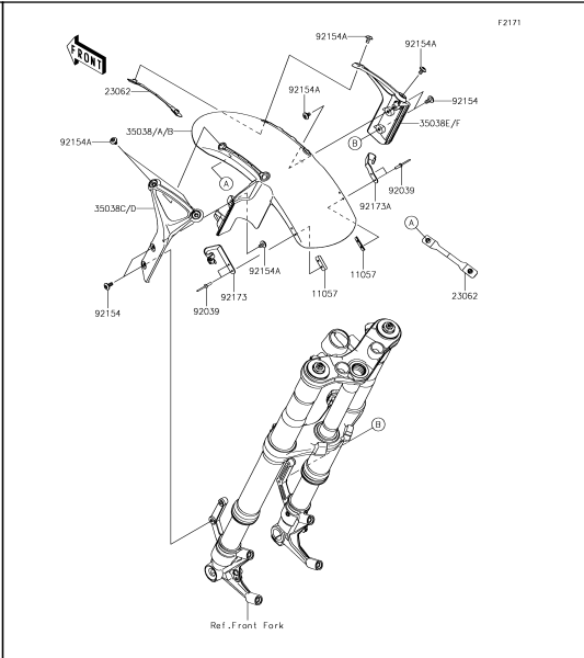
34 Front Fender(s)
