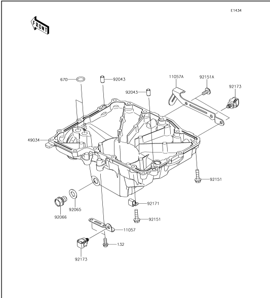
17 Oil Pan
