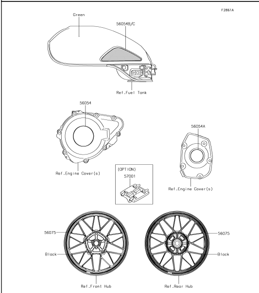
61 Decals(Green)(CJFA)
