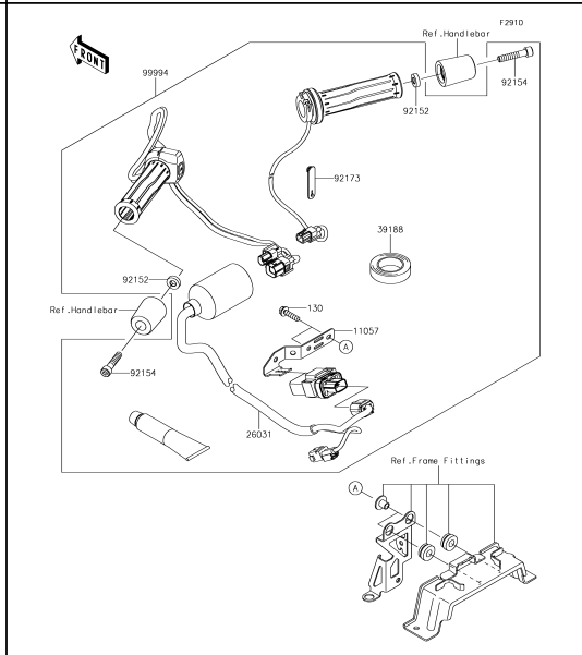
63 Accessory(Grip Heater)
