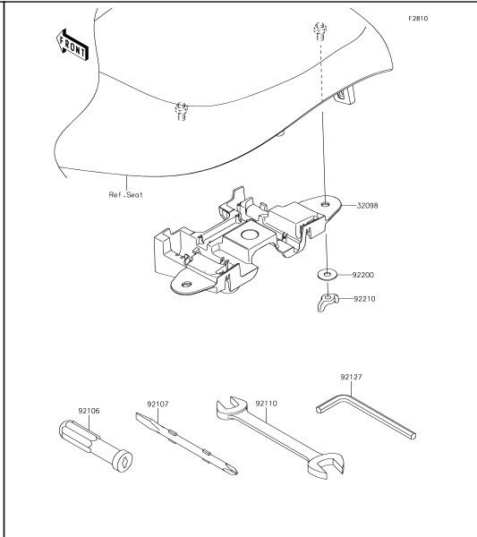
58 Owner's Tools
