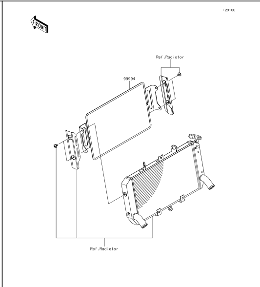
66 Accessory(Radiator Guard)
