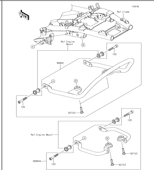
68 Accessory(Grip)
