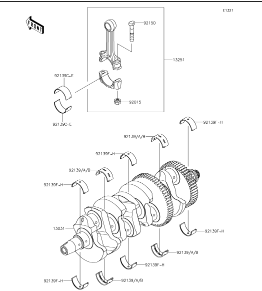
8 Crankshaft
