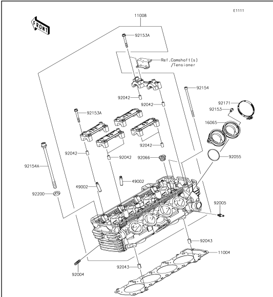
1 Cylinder Head
