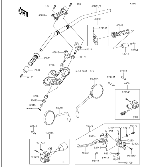
46 Handlebar
