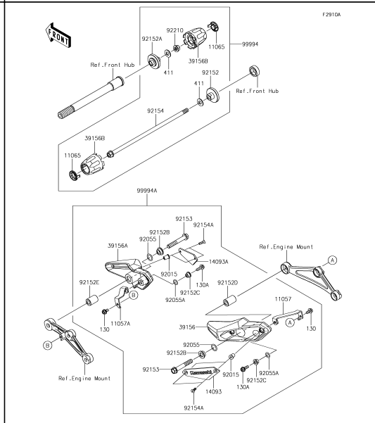
64 Accessory(Slider)
