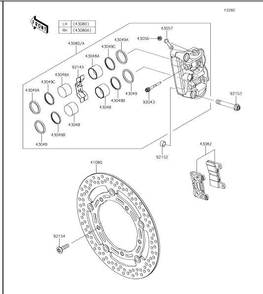
43 Front Brake
