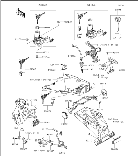
57 Ignition Switch
