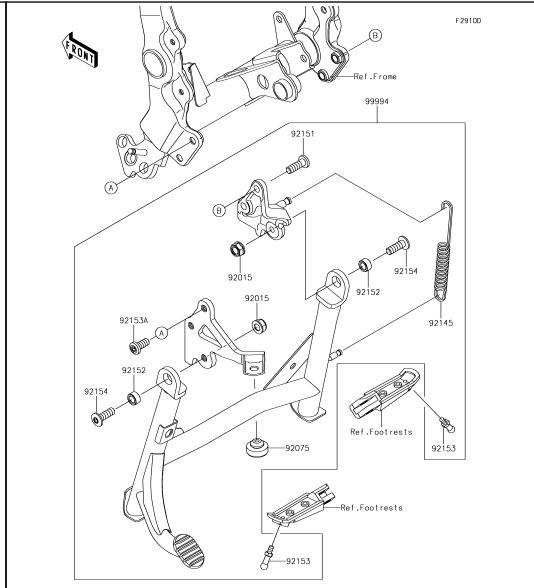
67 Accessory(Center Stand)
