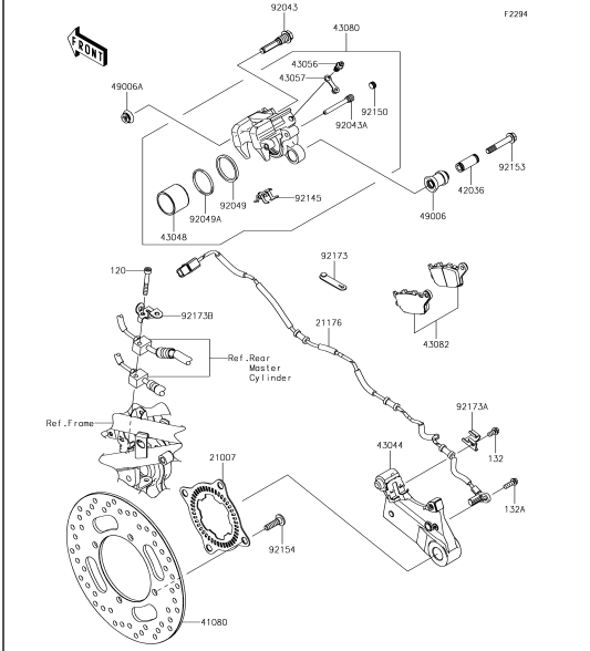
45 Rear Brake
