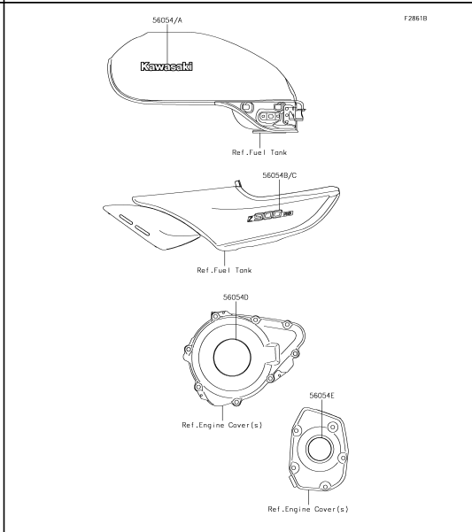
62 Decals(Brown)(CJFB)
