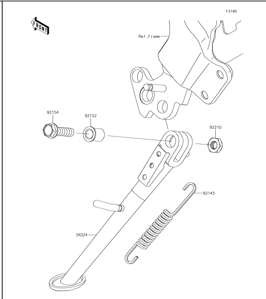
36 Stand(s)
