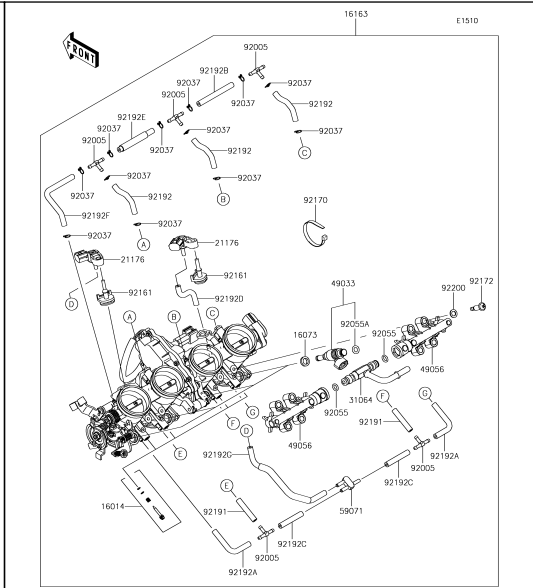
18 Throttle
