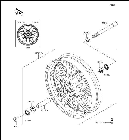
38 Front Hub
