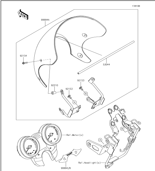
65 Accessory(Cover)
