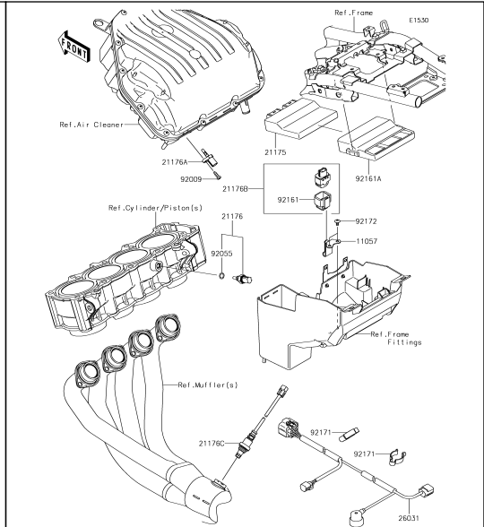
20 Fuel Injection
