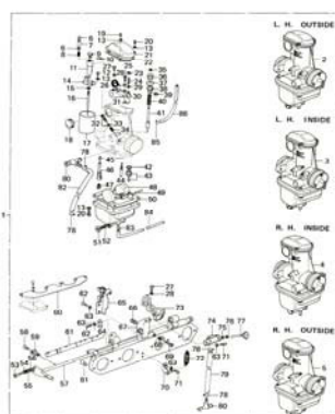
12. Carburetors 2/3
