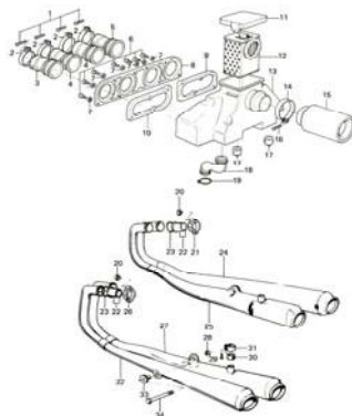
14. Mufflers, Air Cleaner
