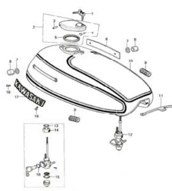
28. Fuel Tank
