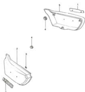
29. Side Covers
