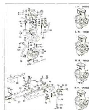
12. Carburetors 3/3
