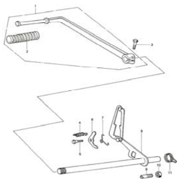
9. Gear Change Mechanism
