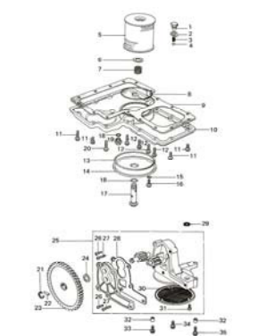
13. Oil Pump, Oil Filter
