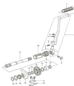
10. Kickstarter
