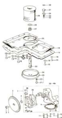
13. Oil Pump, Oil Filter
