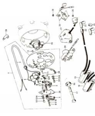
15. Contact Breaker
