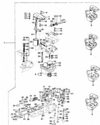
12. Carburetors 3/3
