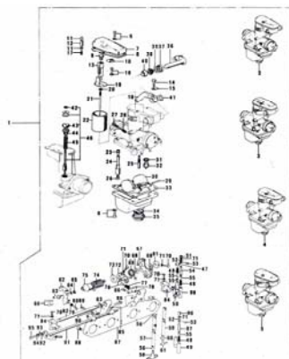
12. Carburetors 1/3
