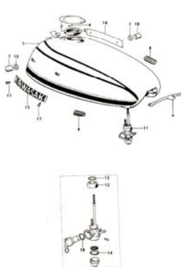
28. Fuel Tank
