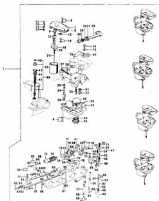
12. Carburetors 2/3
