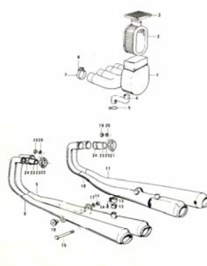
14. Mufflers, Air Cleaner
