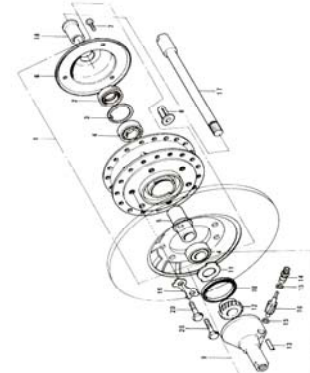
23. Front Hub
