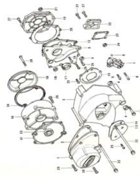
11. Engine Covers
