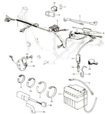
34. Electrical Equipments C
