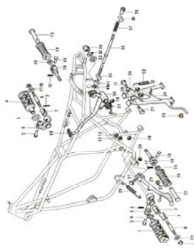
19. Footrests, Stands, Brake Pedal
