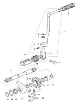
10. Kickstarter
