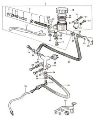
25. Disc Brake Equipments A
