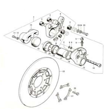
26. Disc Brake Equipments B
