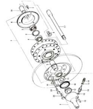
23. Front Hub
