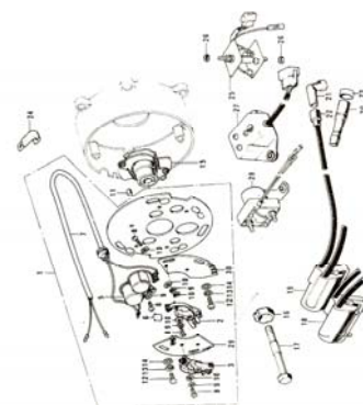
15. Contact Breaker
