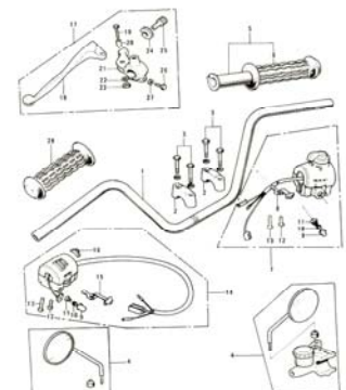
20. Handlebar, Grips
