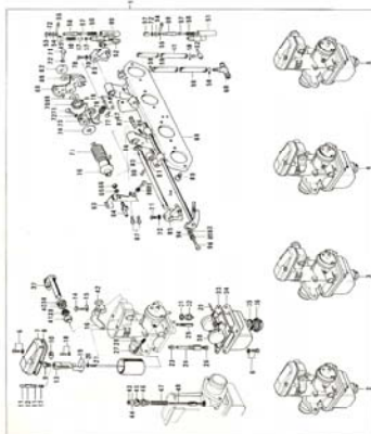
12. Carburetors 2/3
