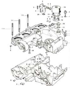
5. Crank Case
