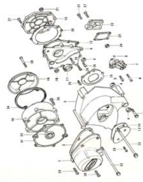
11. Engine Covers
