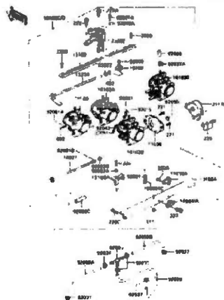
C-10 Throttle (ZX750-E2)(1/2)
