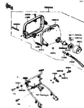
G-5 Head Lamp
