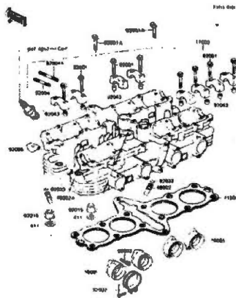
B-3 Cylinder Head
