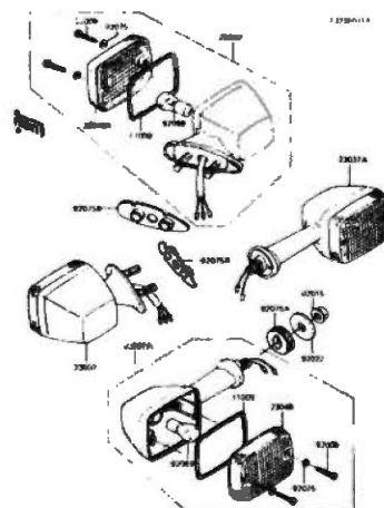
G-7 Turn Signal
