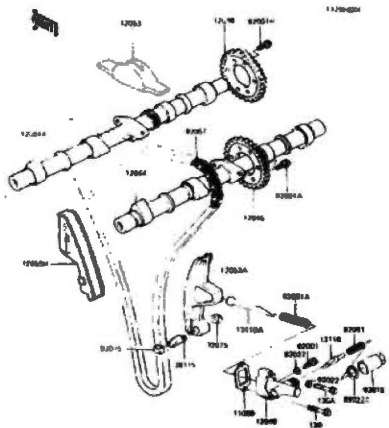
B-9 Camshaft/Tensioner
