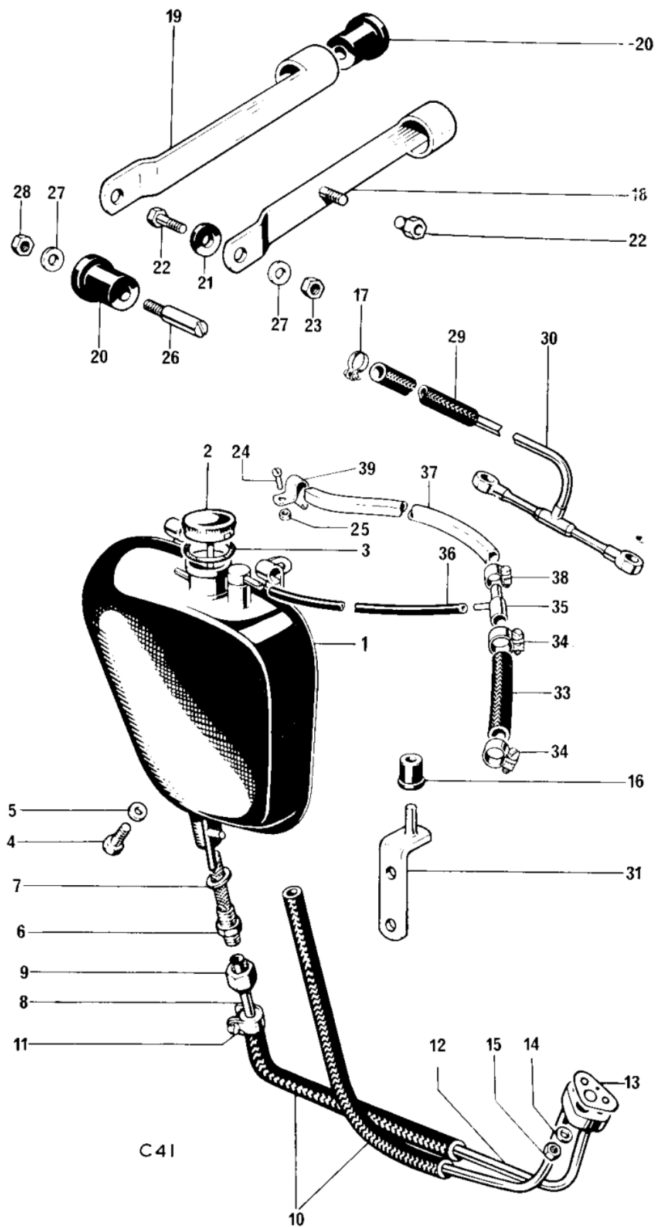
Fig. 28. OIL TANK
