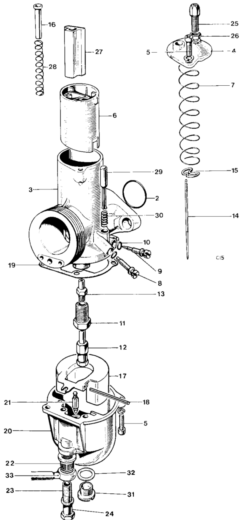
Fig. 5. CARBURETOR T100C
