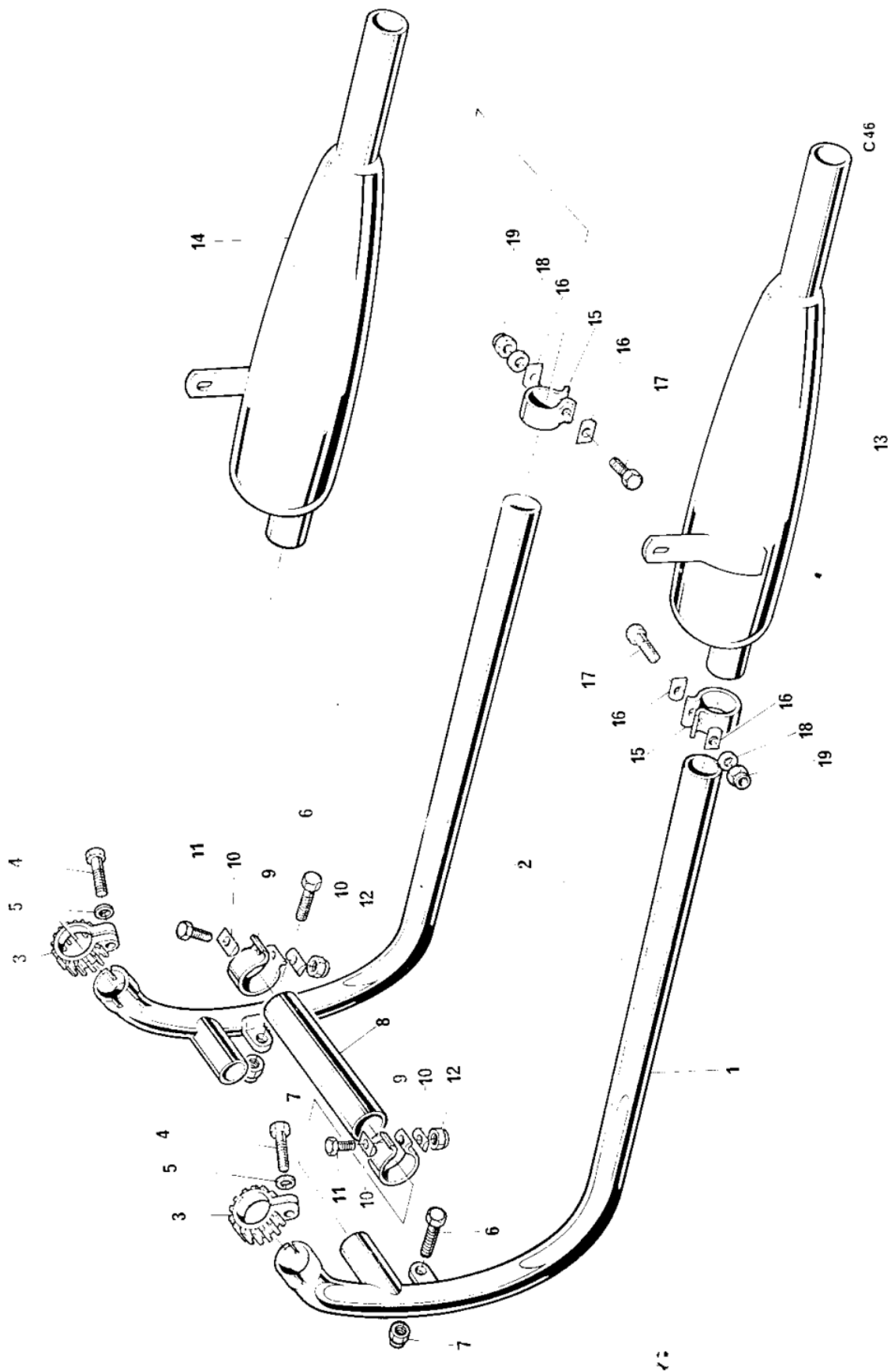
Fig. 15. EXHAUST SYSTEM
