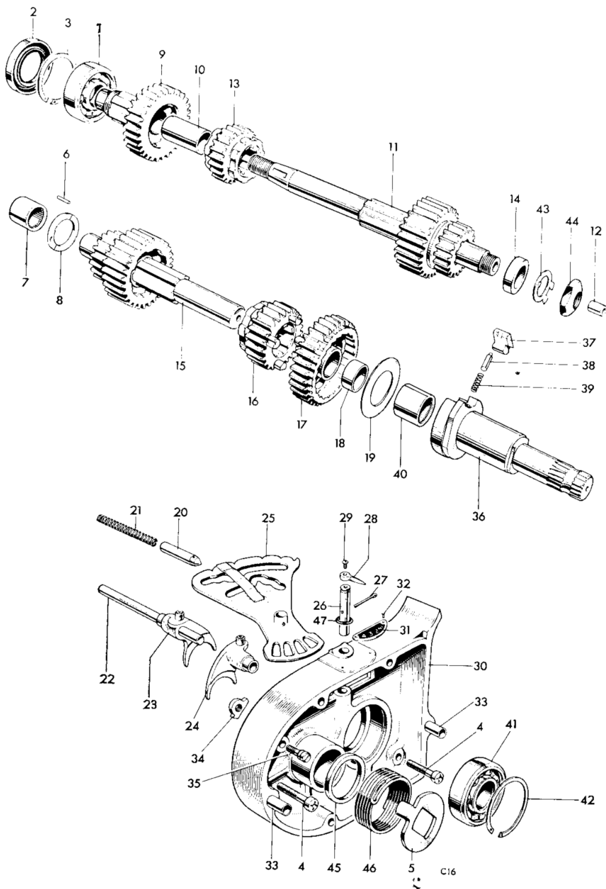
Fig. 9. GEARBOX SHAFTS, BEARINGS AND INNER COVER
