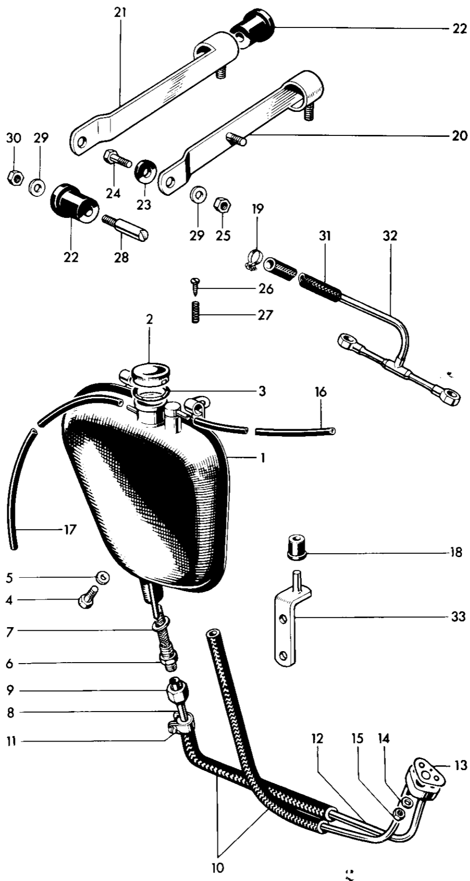
Fig. 25. OIL TANK
