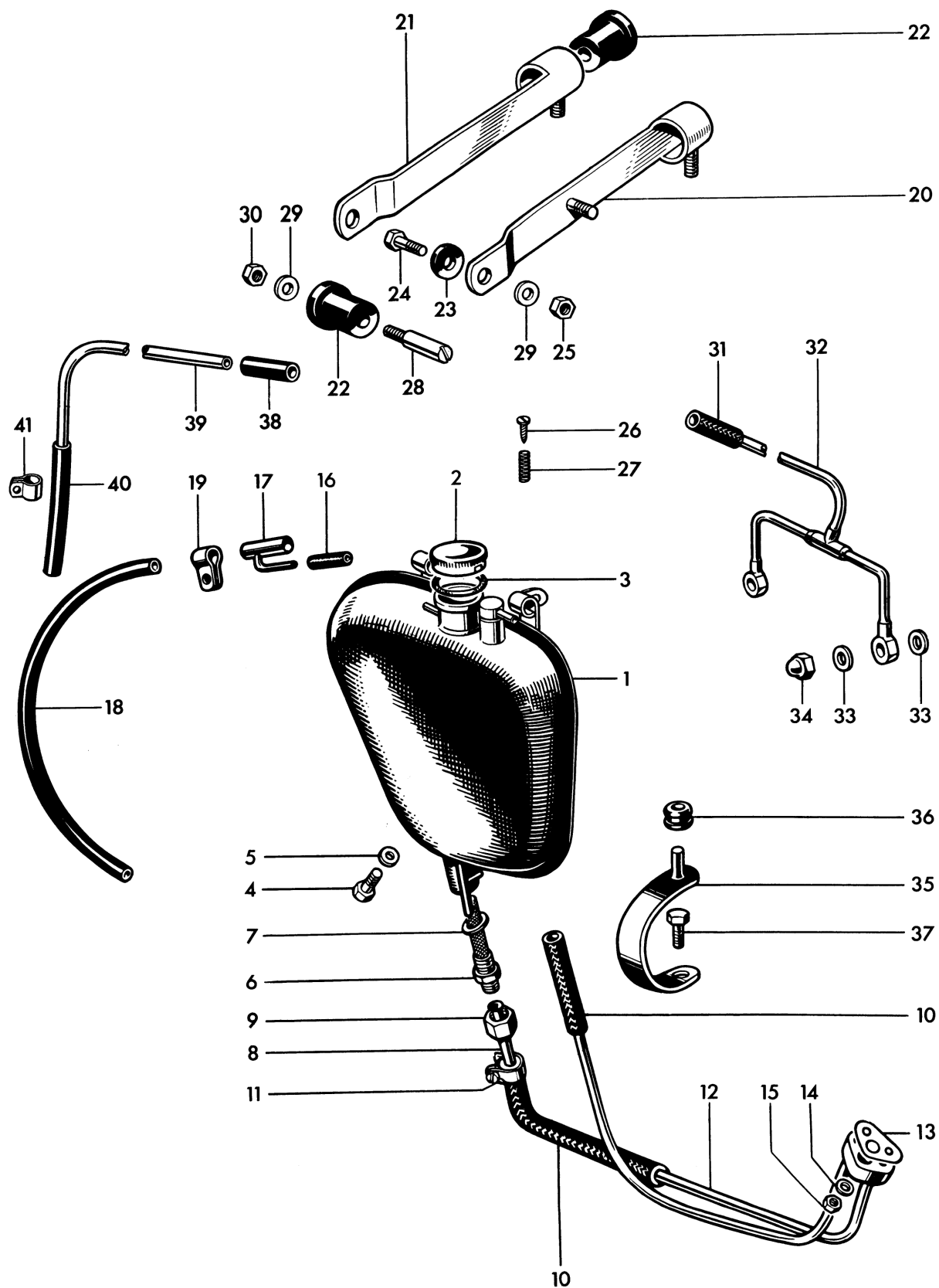
Fig. 26. OIL TANK
