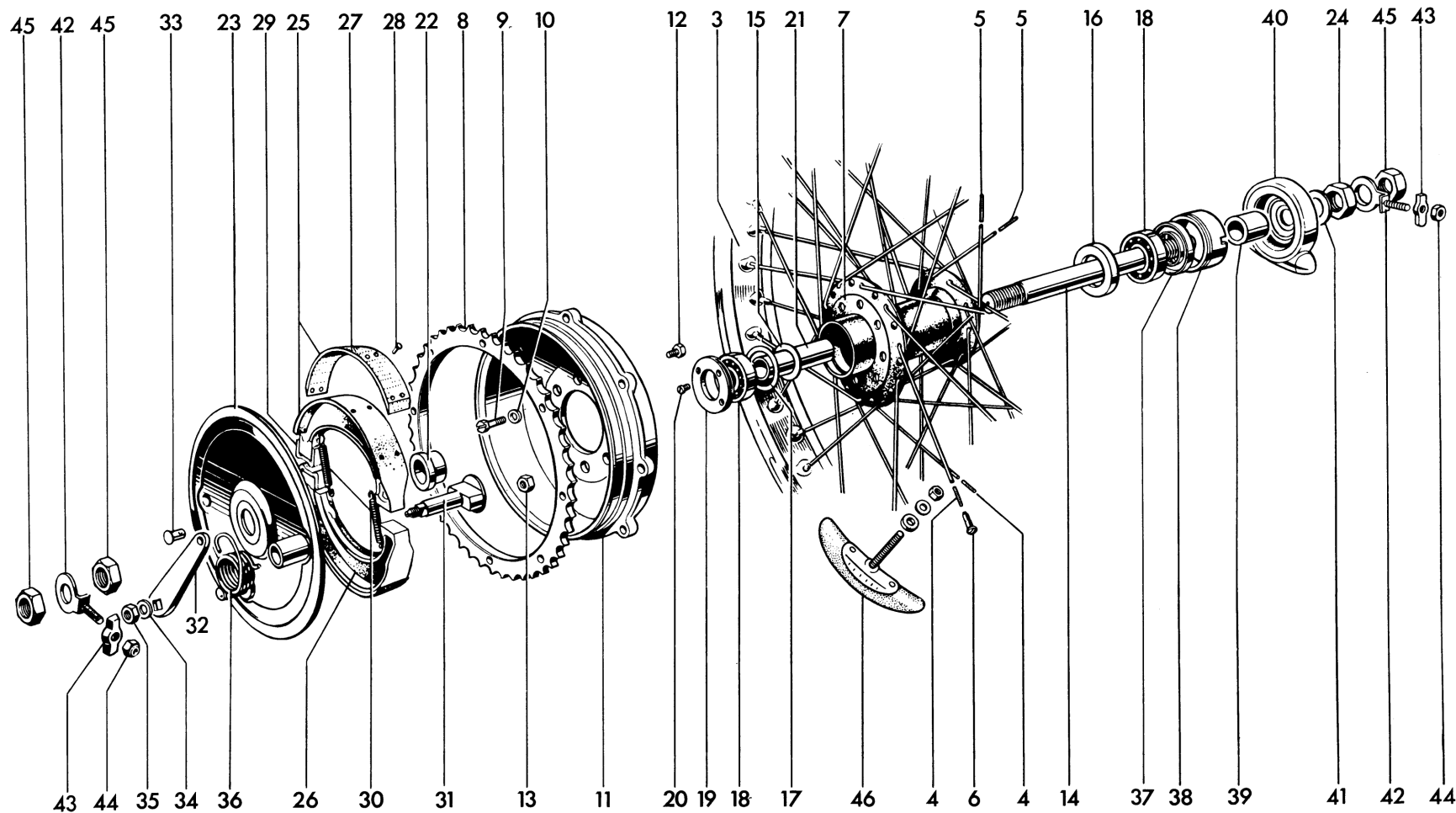
Fig. 23. REAR WHEEL
