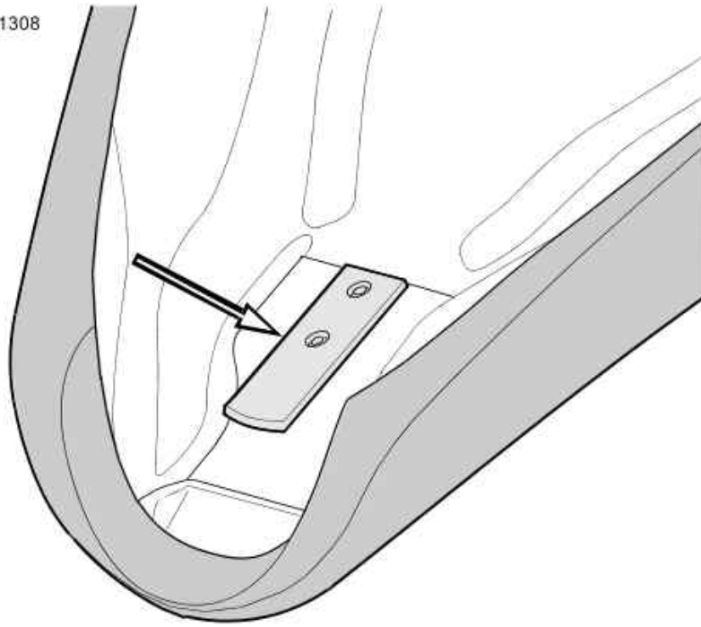
Seat Tongue (typical)
