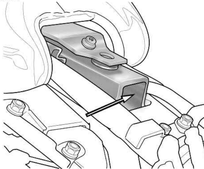
Frame Back
