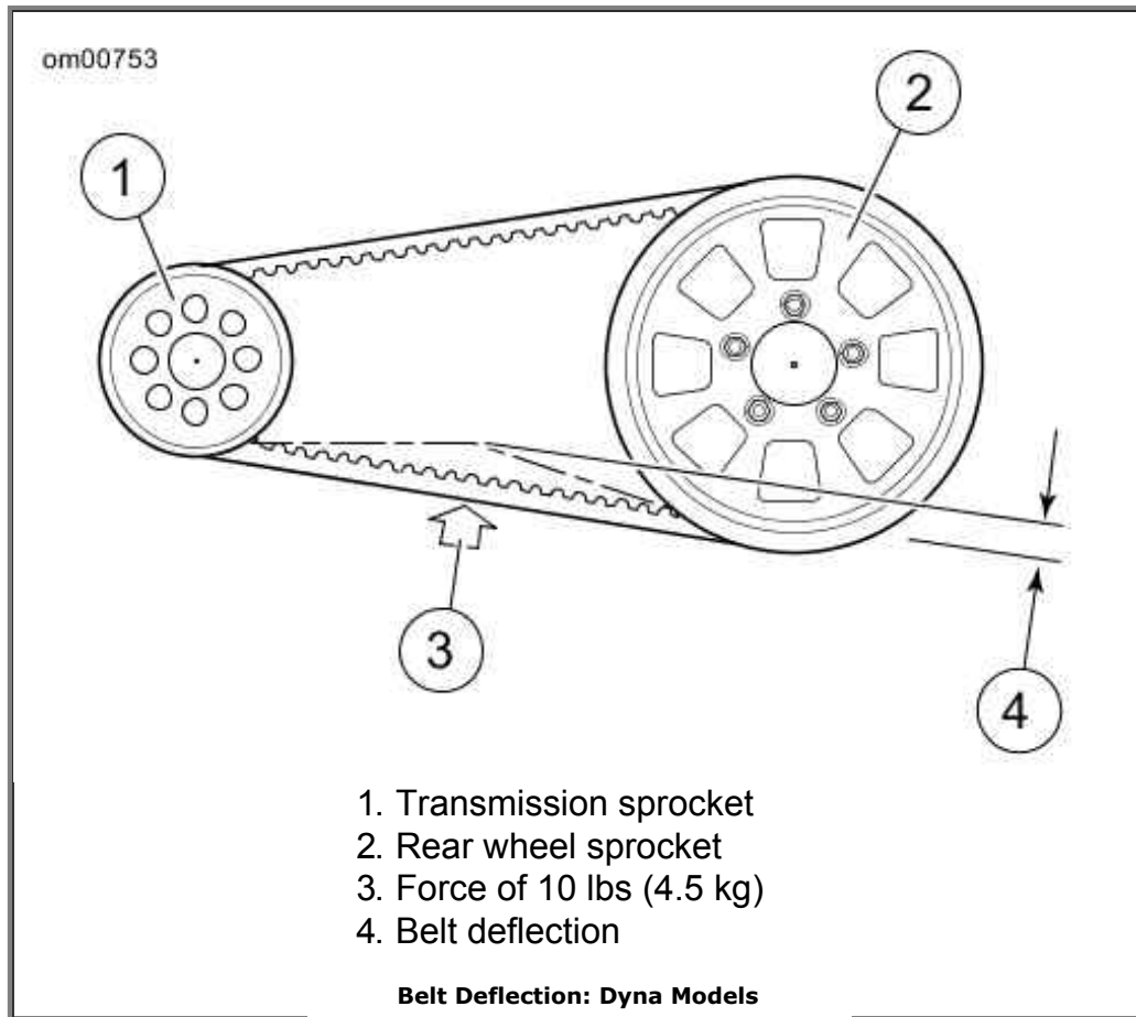
Belt Deflection: 2008 Dyna Models
