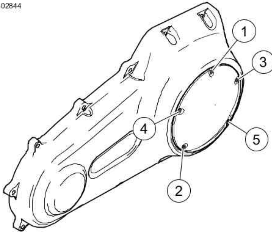
Clutch Cover Torque Sequence
