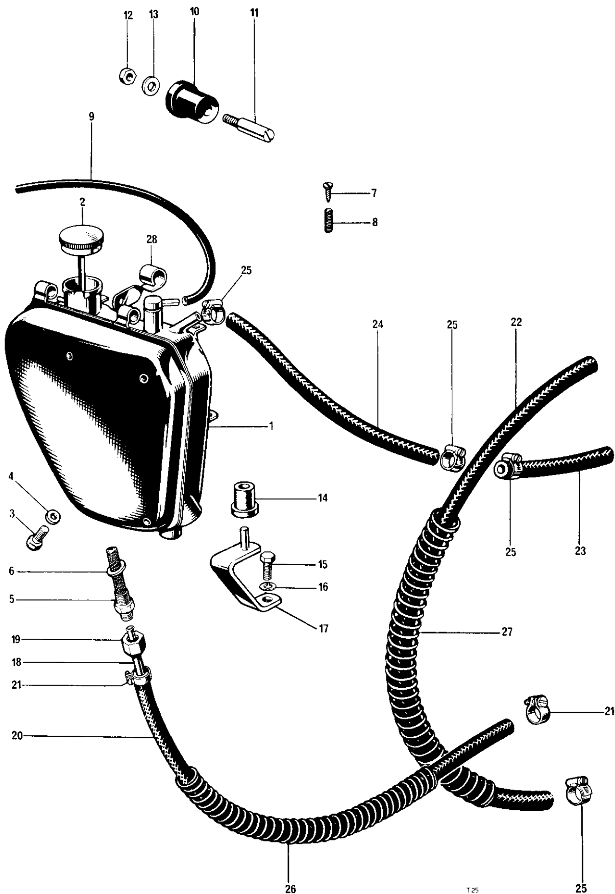
Fig. 25. OIL TANK
