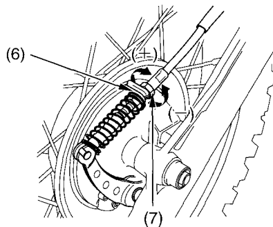
(6) lower lock nut
