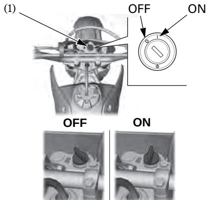
(1) Ignition switch
