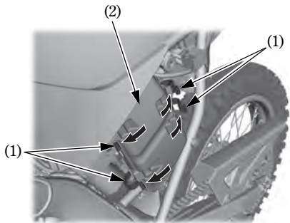
(1) Retainer clips (2) Air cleaner housing cover
