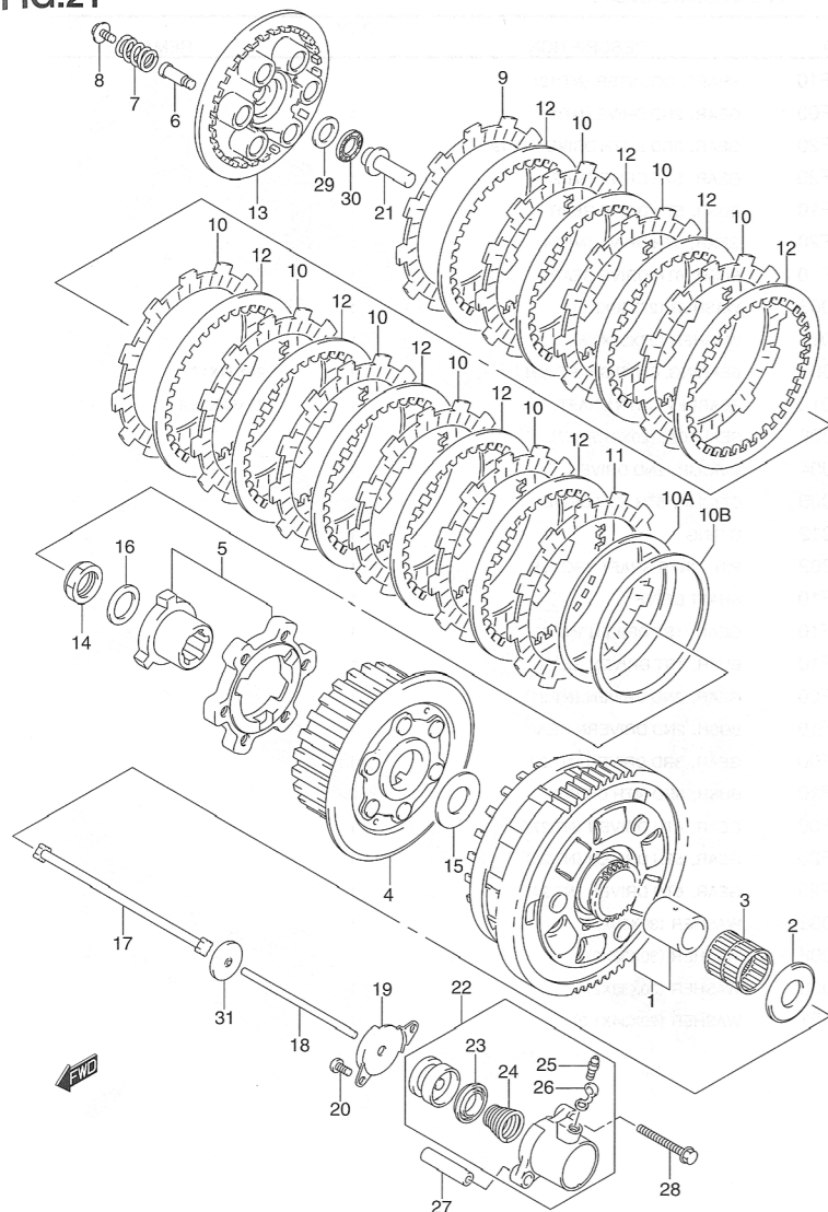
GSX1400K2 E02_021 CLUTCH
