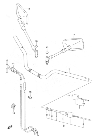
FIG.43 HANDLEBAR (G-10)
