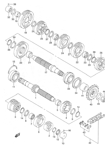
FIG.22 TRANSMISSION (D-9)
