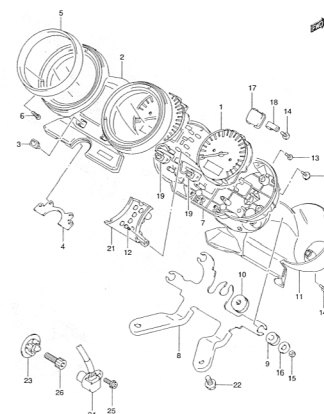
FIG.29 SPEEDOMETER (F-2)
