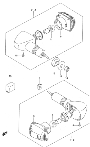
FIG.33A TURN SIGNAL LAMP (E24,F.NO.100197~) (F-7)
