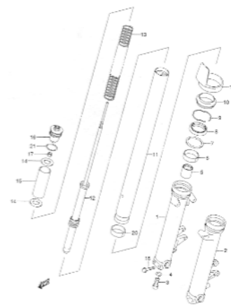
FIG.50 FRONT FORK DAMPER (H-9)
