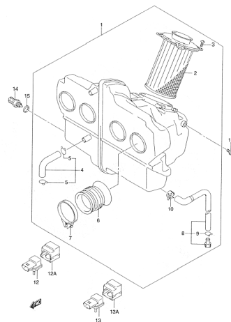
FIG.20 SECOND AIR (D-7)
