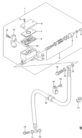
FIG.56 CLUTCH MASTER CYLINDER (I-6)
