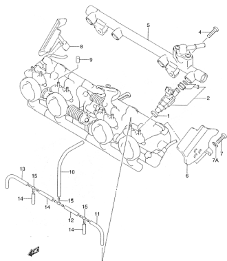
FIG.15A THROTTLE BODY HOSE/JOINT (MODEL K3) (C-12)
