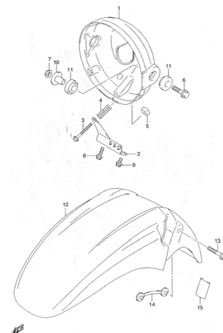
FIG.42 HEADLAMP HOUSING (G-9)
