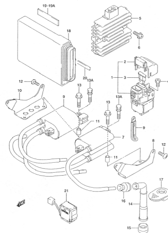
FIG.27 ELECTRICAL (E-5)
