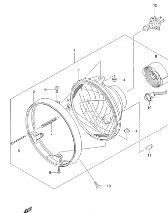
FIG.30 HEADLAMP ASSY (E2,E19) (F-3)
