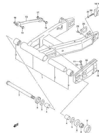
FIG.57A REAR SWINGARM (MODEL K3) (J-3)
