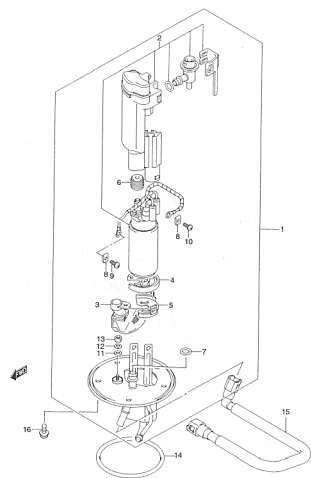
FIG.19 FUEL PUMP (D-6)
