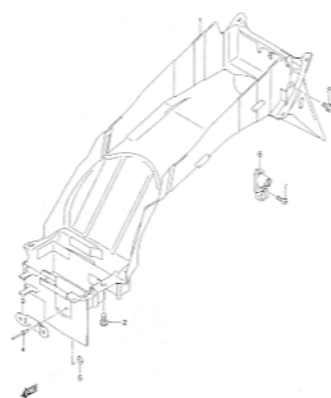
FIG.49 SEAT TAIL COVER (MODEL K2) (H-7)
