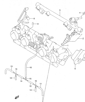
FIG.15 THROTTLE BODY HOSE/JOINT (MODEL K2) (C-11)
