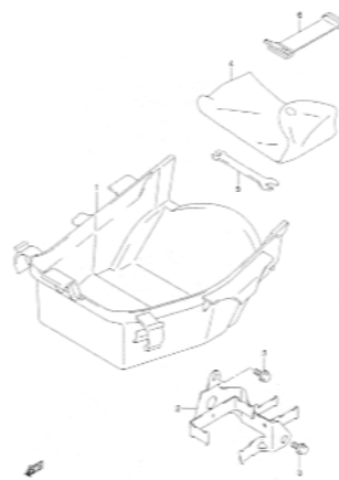
FIG.49A SEAT TAIL COVER (MODEL K3) (H-8)
