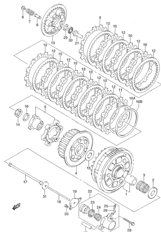
FIG.21 CLUTCH (D-8)
