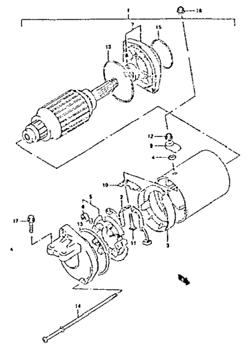
FIG.19 STARTING MOTOR (D-7)
