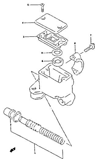
FIG.49 FRONT MASTER CYLINDER (I-7)
