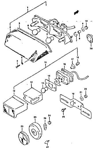
FIG.26 REAR COMBINATION LAMP (E-8)
