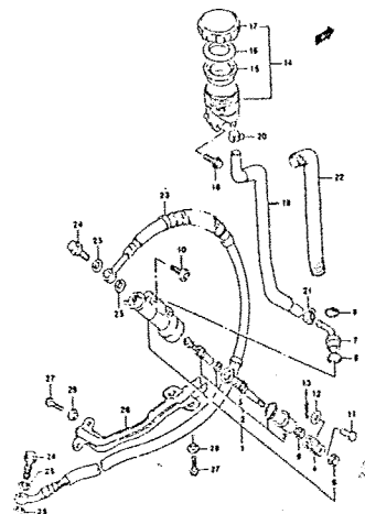
FIG.54 REAR MASTER CYLINDER (I-6)
