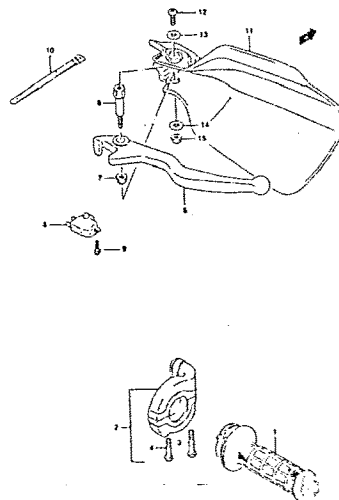
FIG.38 RIGHT HANDLE LEVER (G-3)
