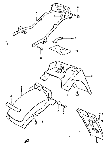
FIG.40 REAR FENDER (G-5)
