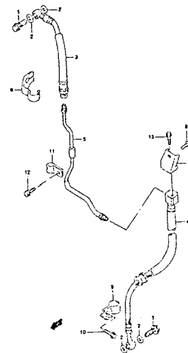
FIG.48 FRONT BRAKE HOSE (H-6)
