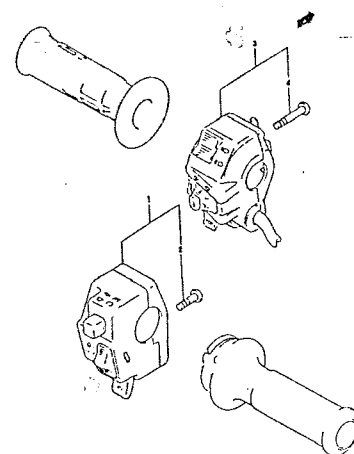
FIG.28 HANDLE SWITCH (E-10)
