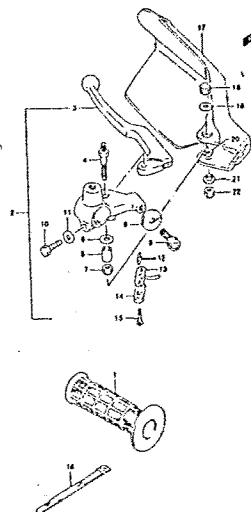
FIG.39 LEFT HANDLE LEVER (G-4)
