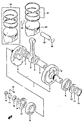
FIG.5 CRANKSHAFT (B-8)
