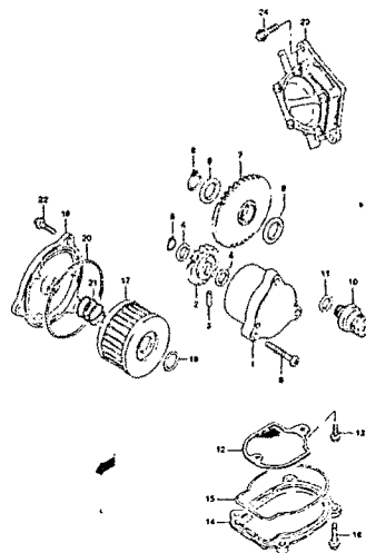
FIG.14 OIL PUMP - FUEL PUMP (C-7)
