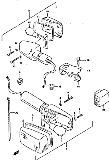
FIG.25 TURN SIGNAL LAMP (E-7)
