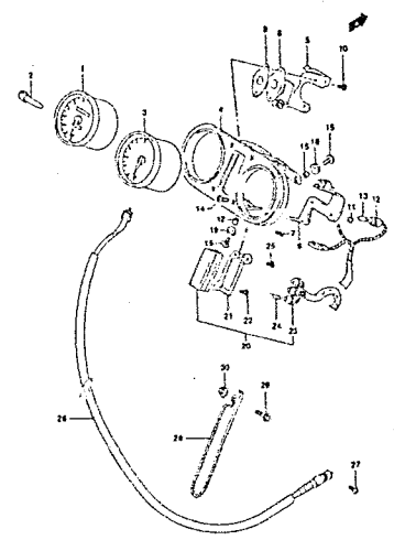
FIG.23 SPEEDOMETER (E-5)
