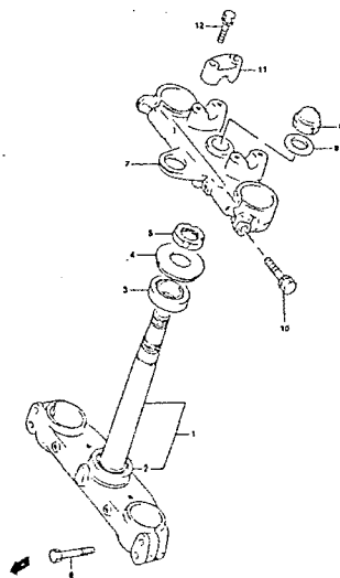
FIG.45 STEERING STEM (H-3)
