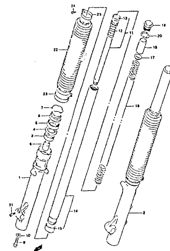
FIG.44 FRONT FORK (H-2)
