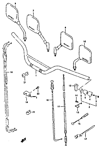
FIG.37 HANDLEBAR (G-2)
