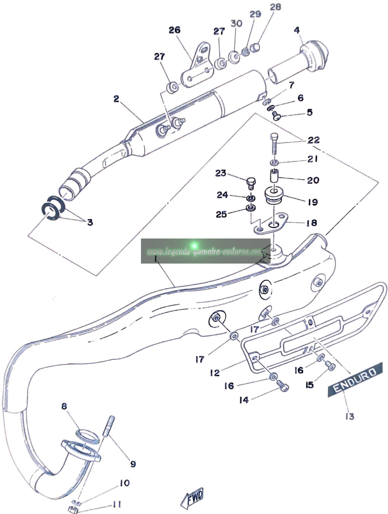
Fig. 11 EXHAUST
