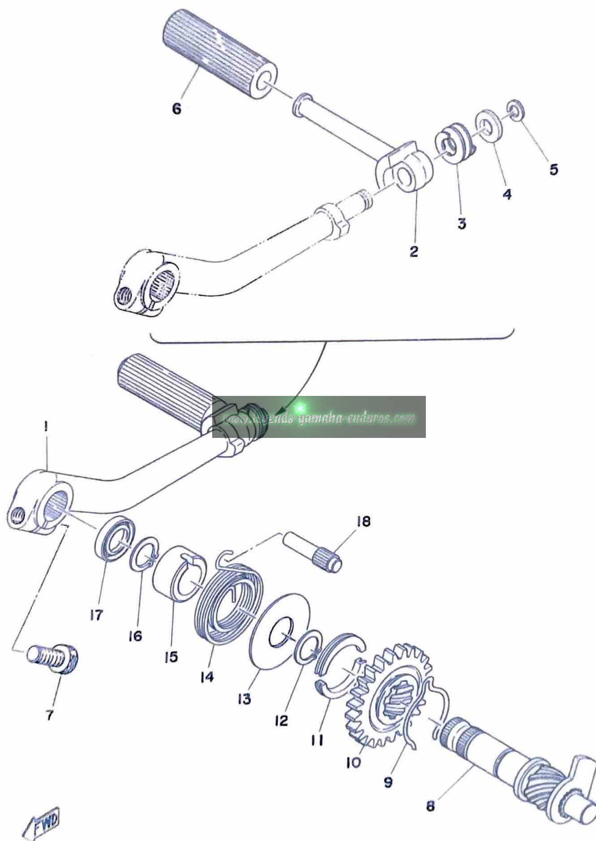
Fig. 8 KICK STARTER
