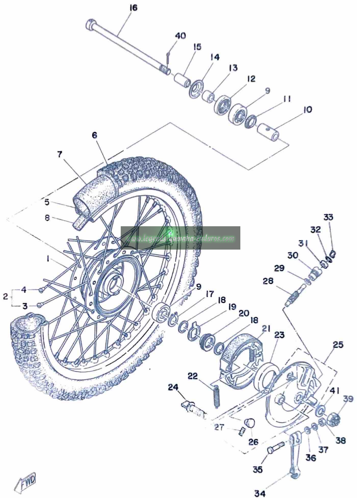
Fig. 24 FRONT WHEEL
