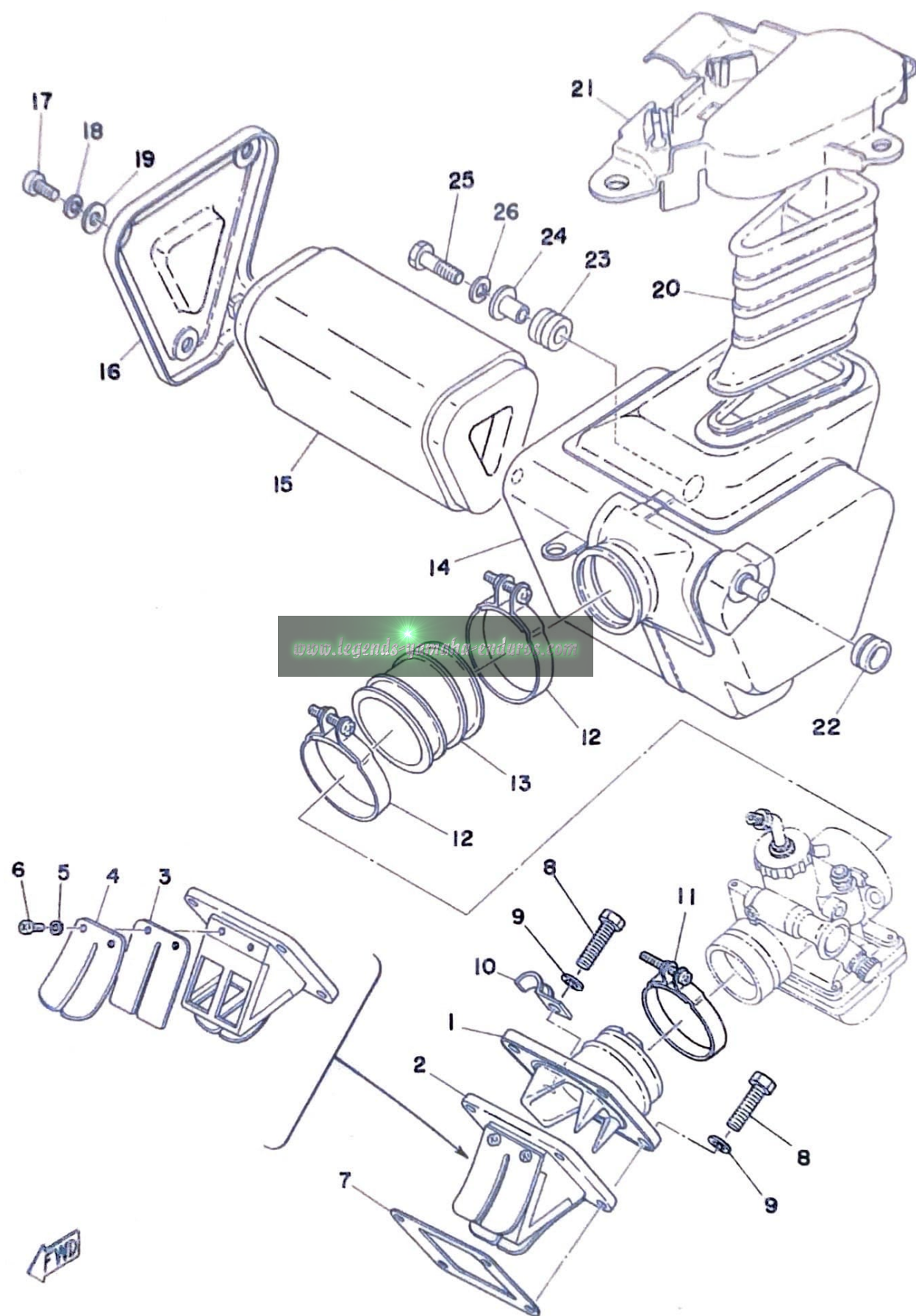
Fig. 9 INTAKE
