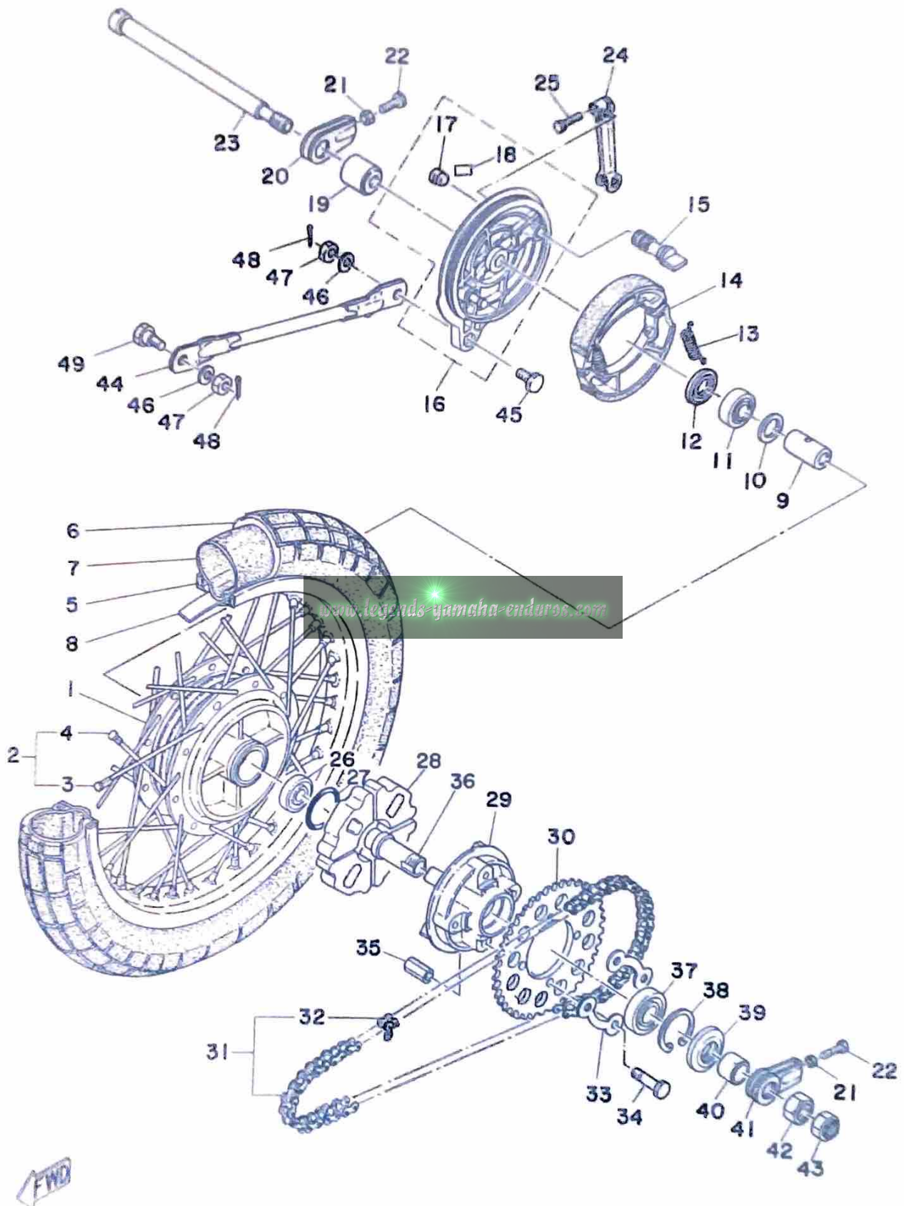
Fig. 25 REAR WHEEL
