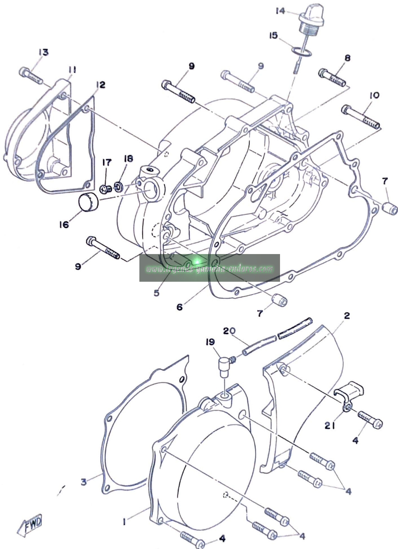
Fig. 2 CRANKCASE COVER
