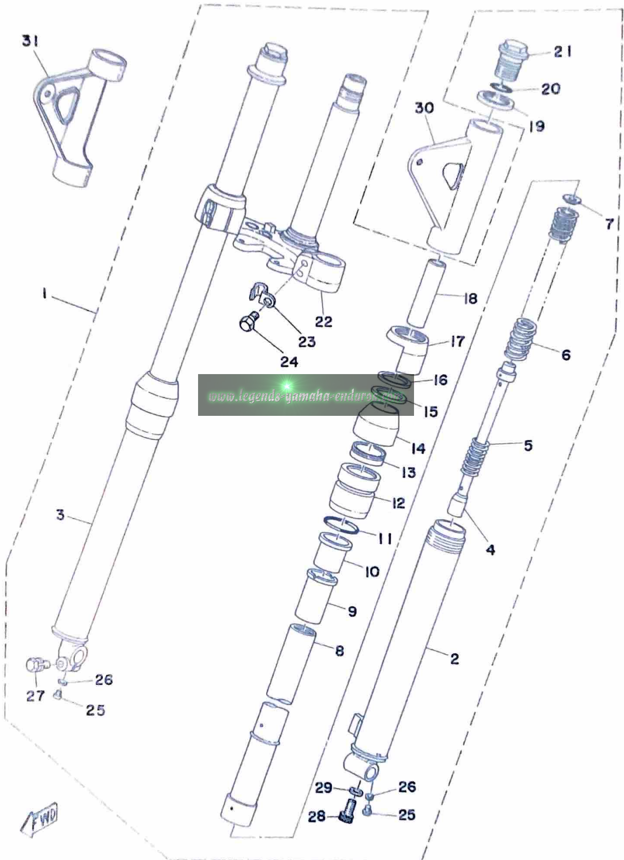
Fig. 18 FRONT FORK
