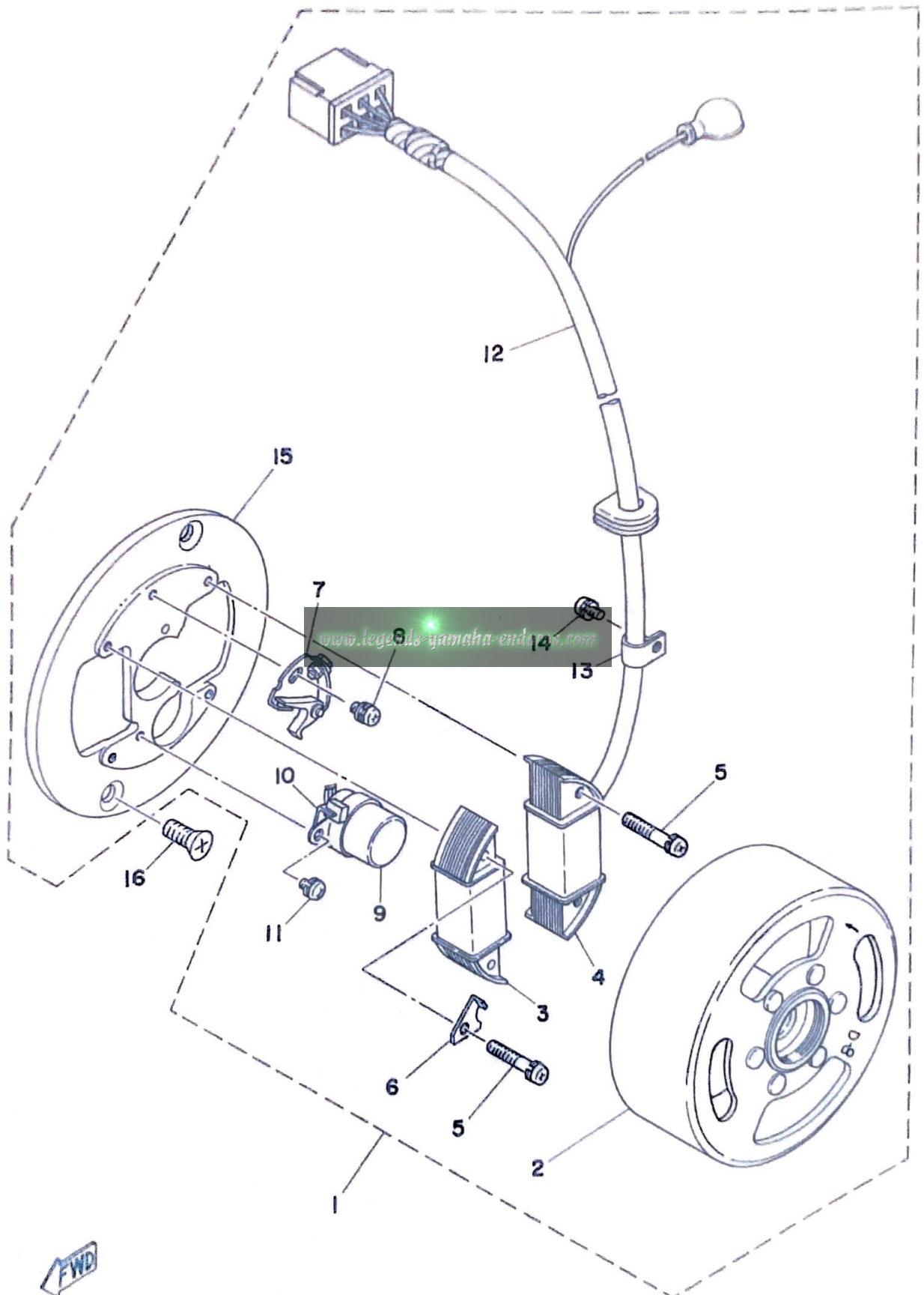
Fig. 13 FLYWHEEL MAGNETO
