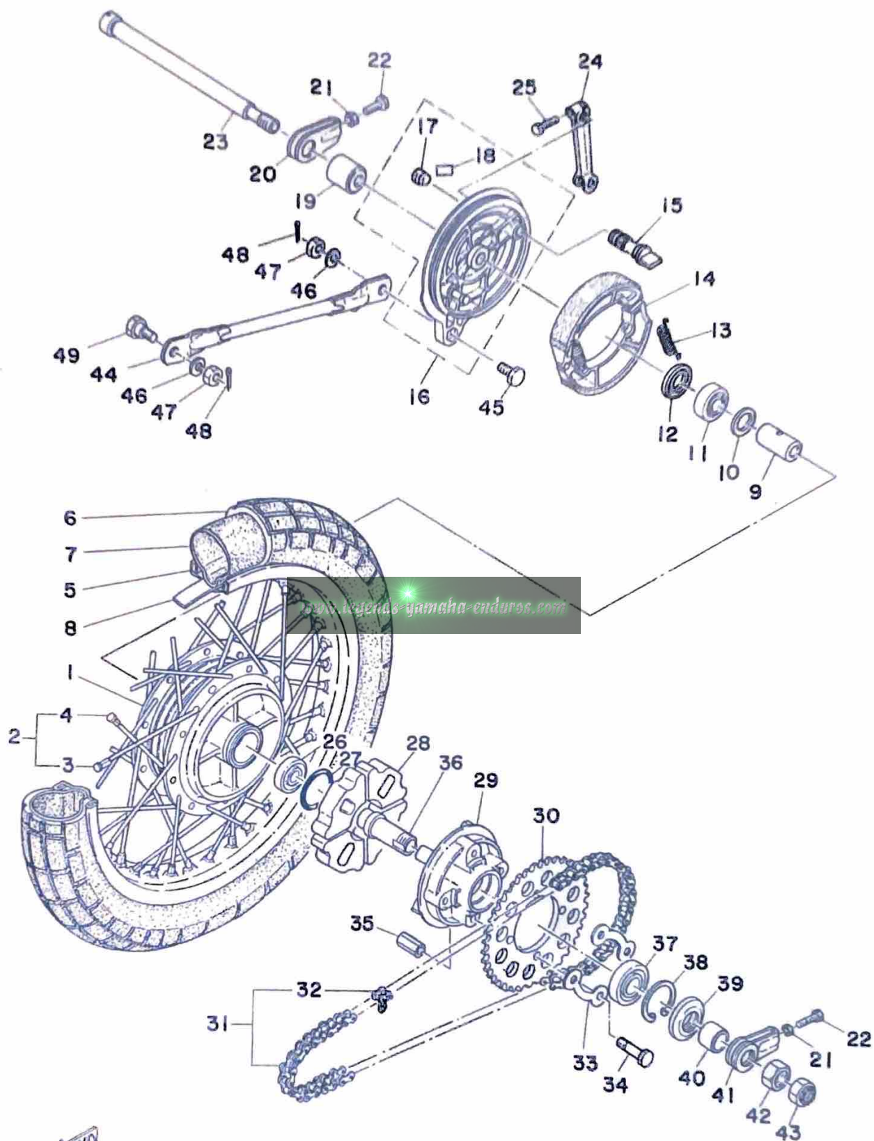
Fig. 25 REAR WHEEL
