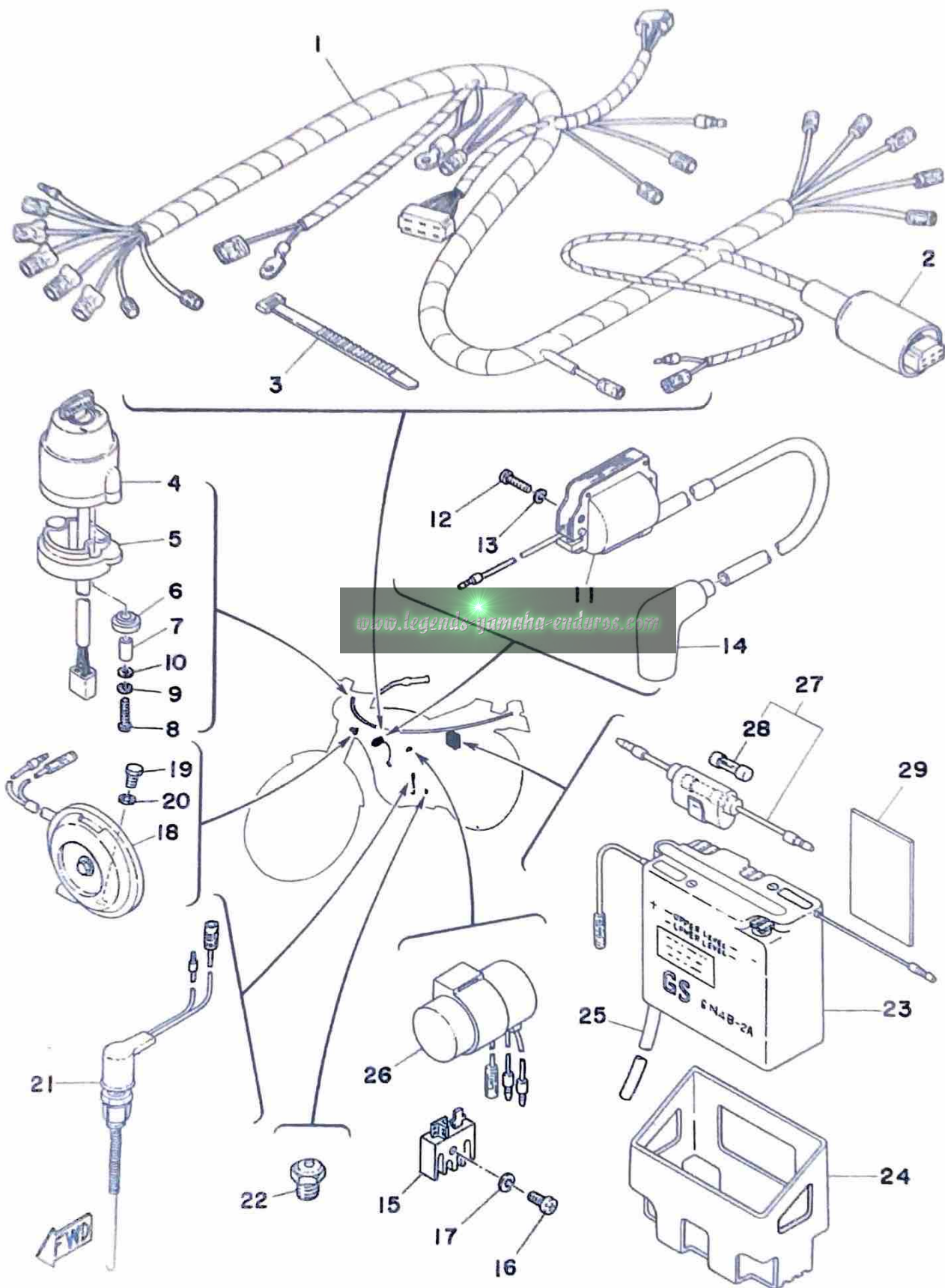
Fig. 29 ELECTRICAL
