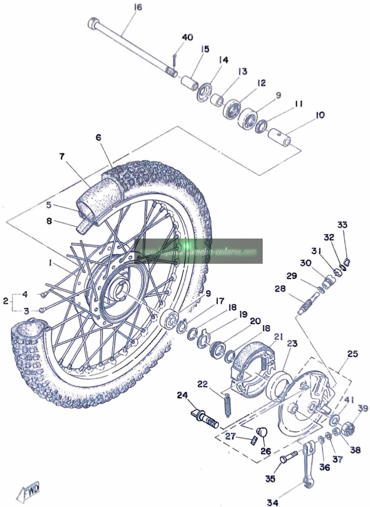
Fig. 24 FRONT WHEEL
