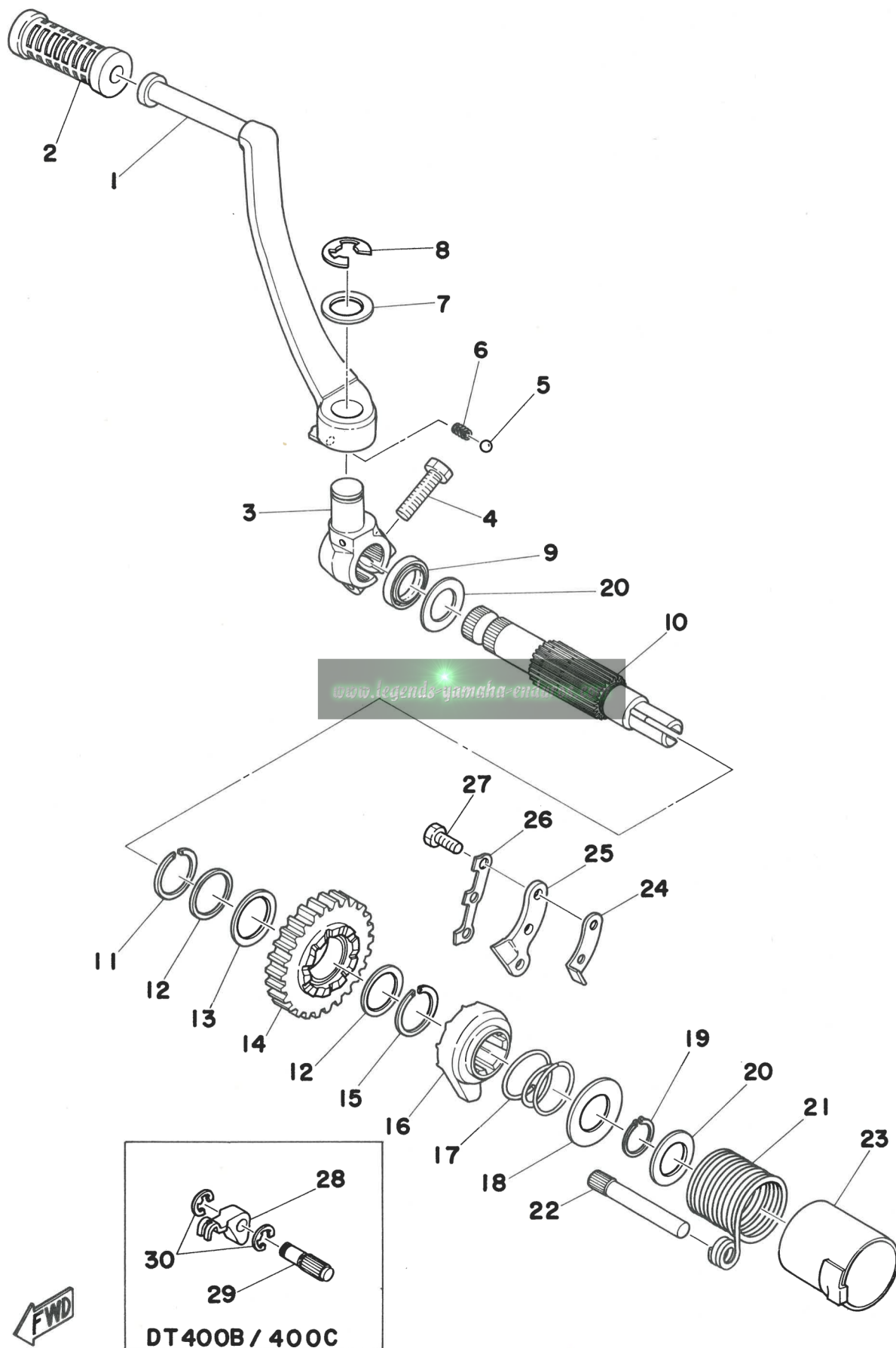
Fig. 9 KICK STARTER
