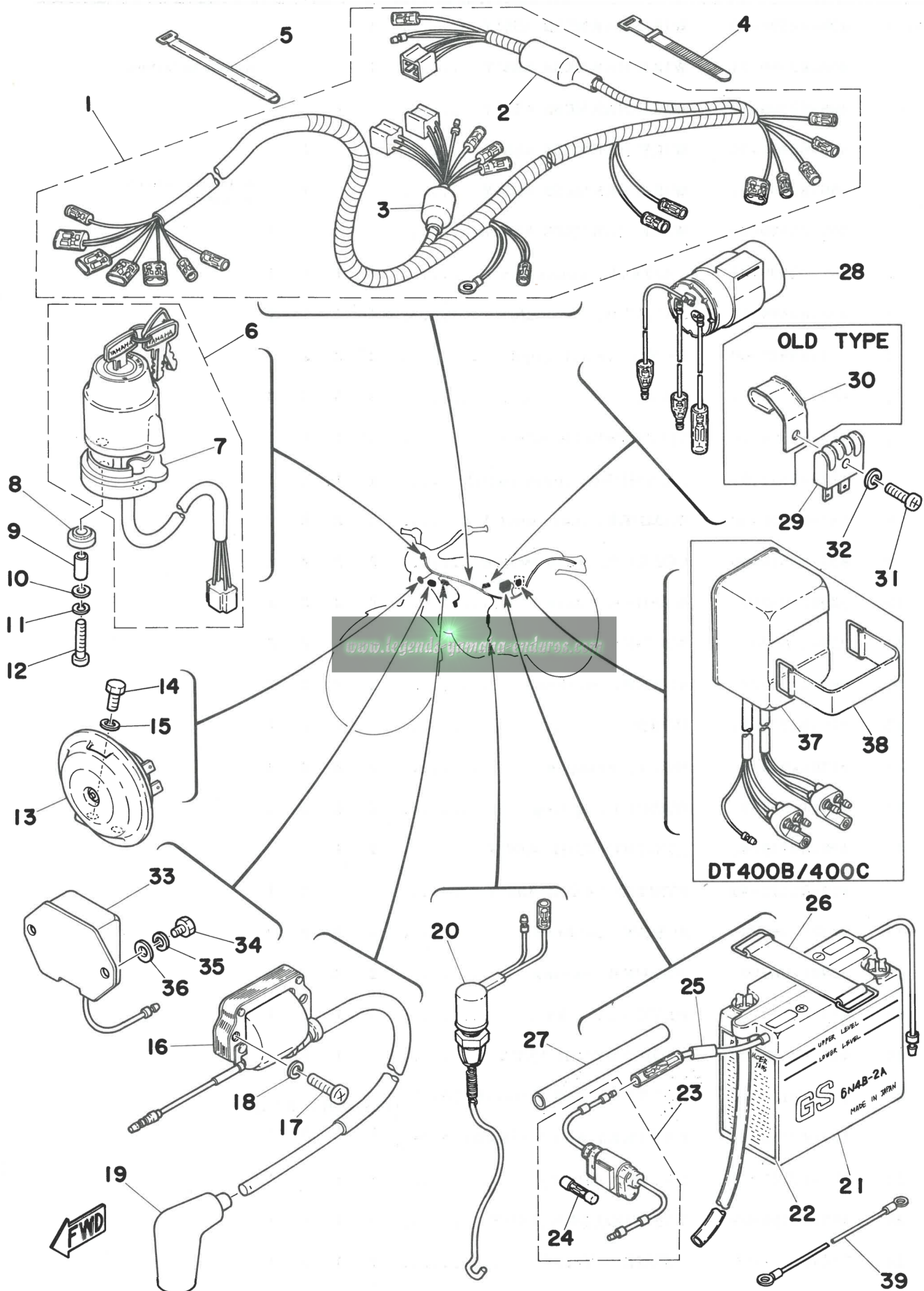
Fig. 35 ELECTRICAL
