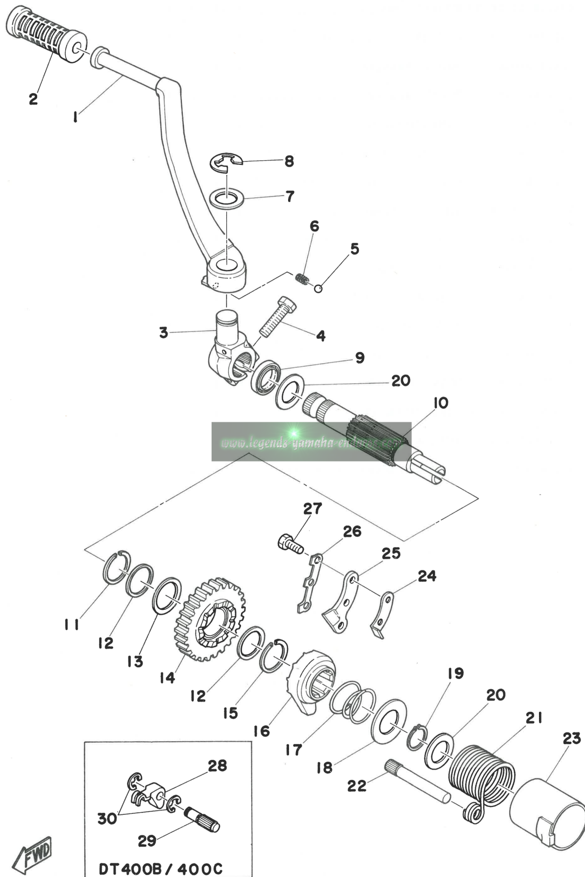
Fig. 9 KICK STARTER
