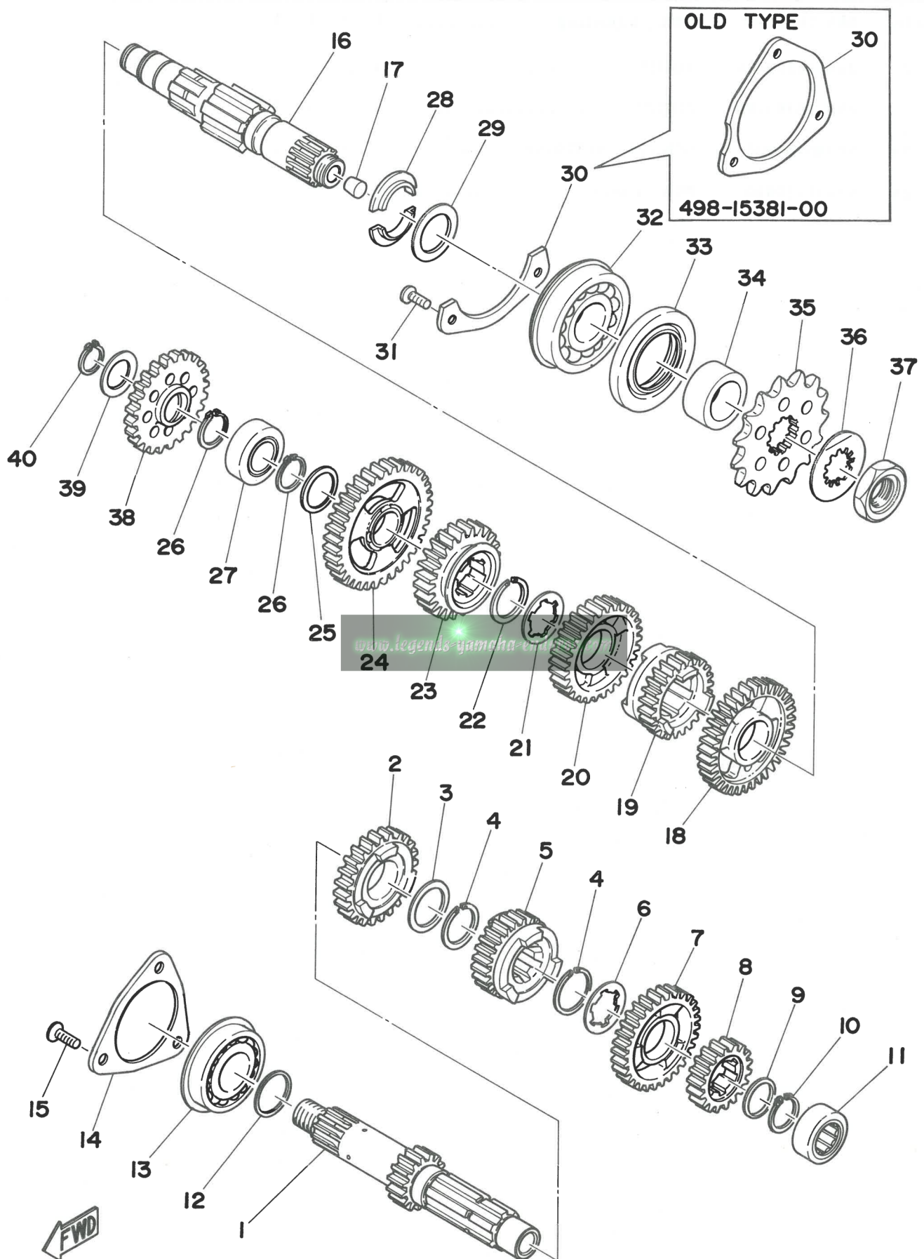
Fig. 6 TRANSMISSION
