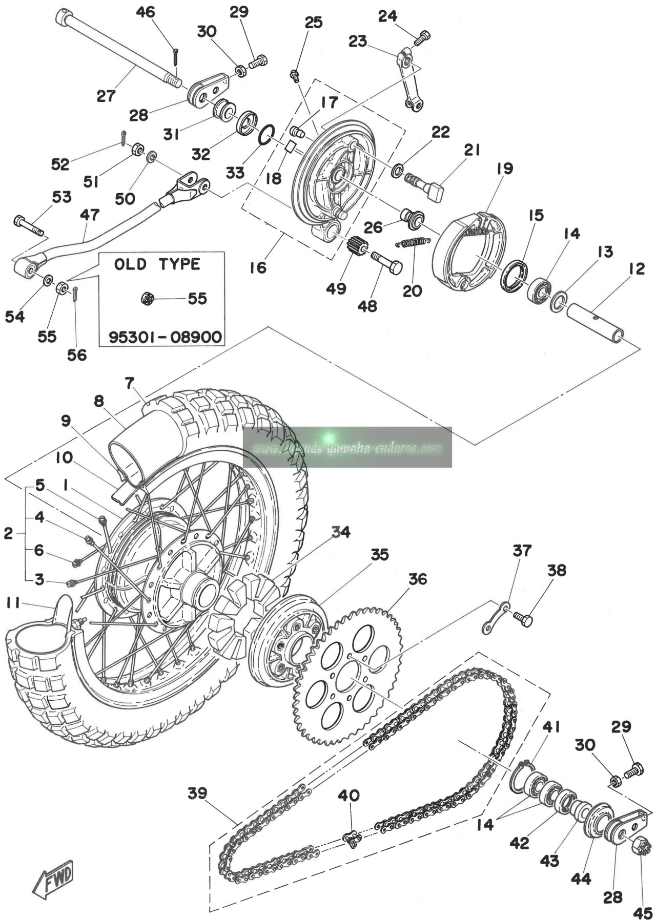
Fig. 30 REAR WHEEL
