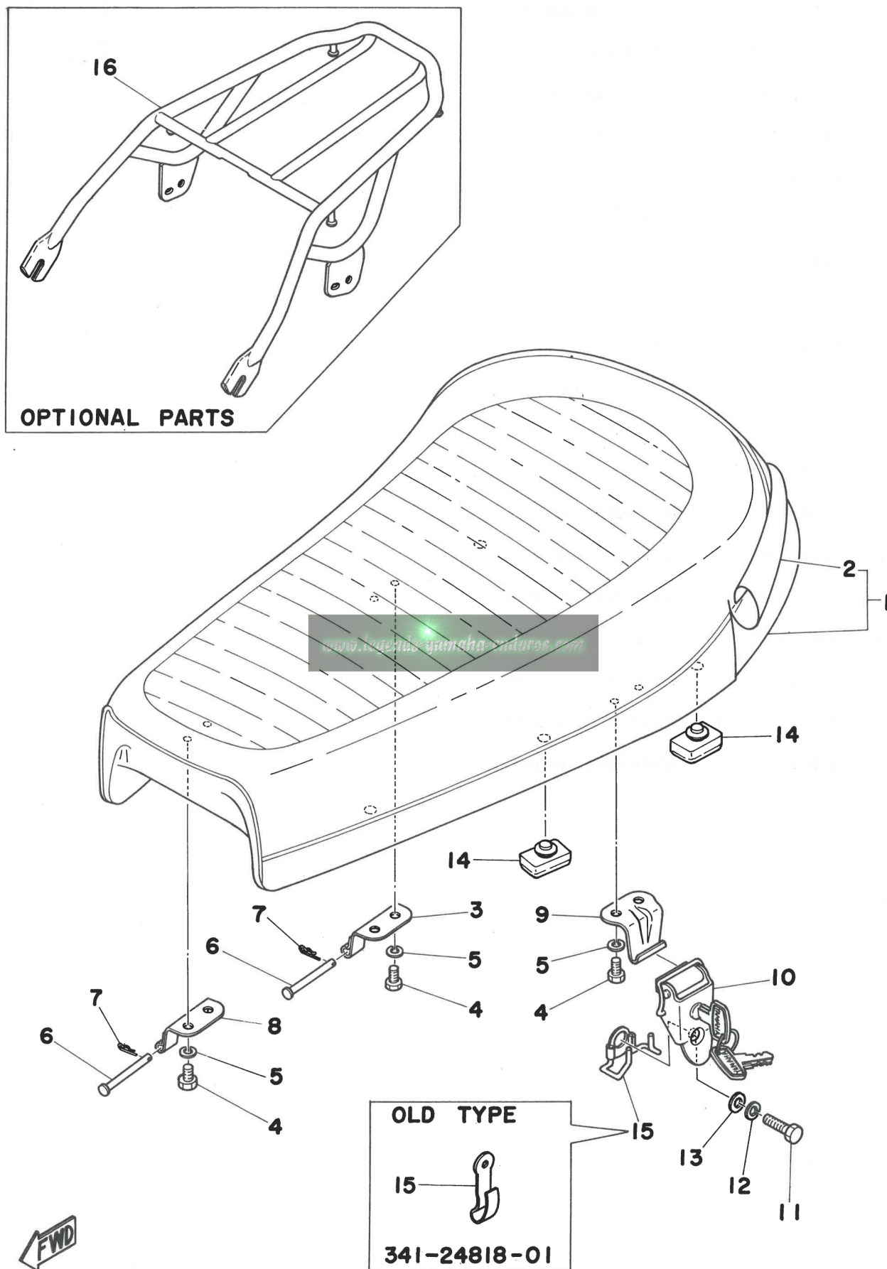
Fig. 28 SEAT
