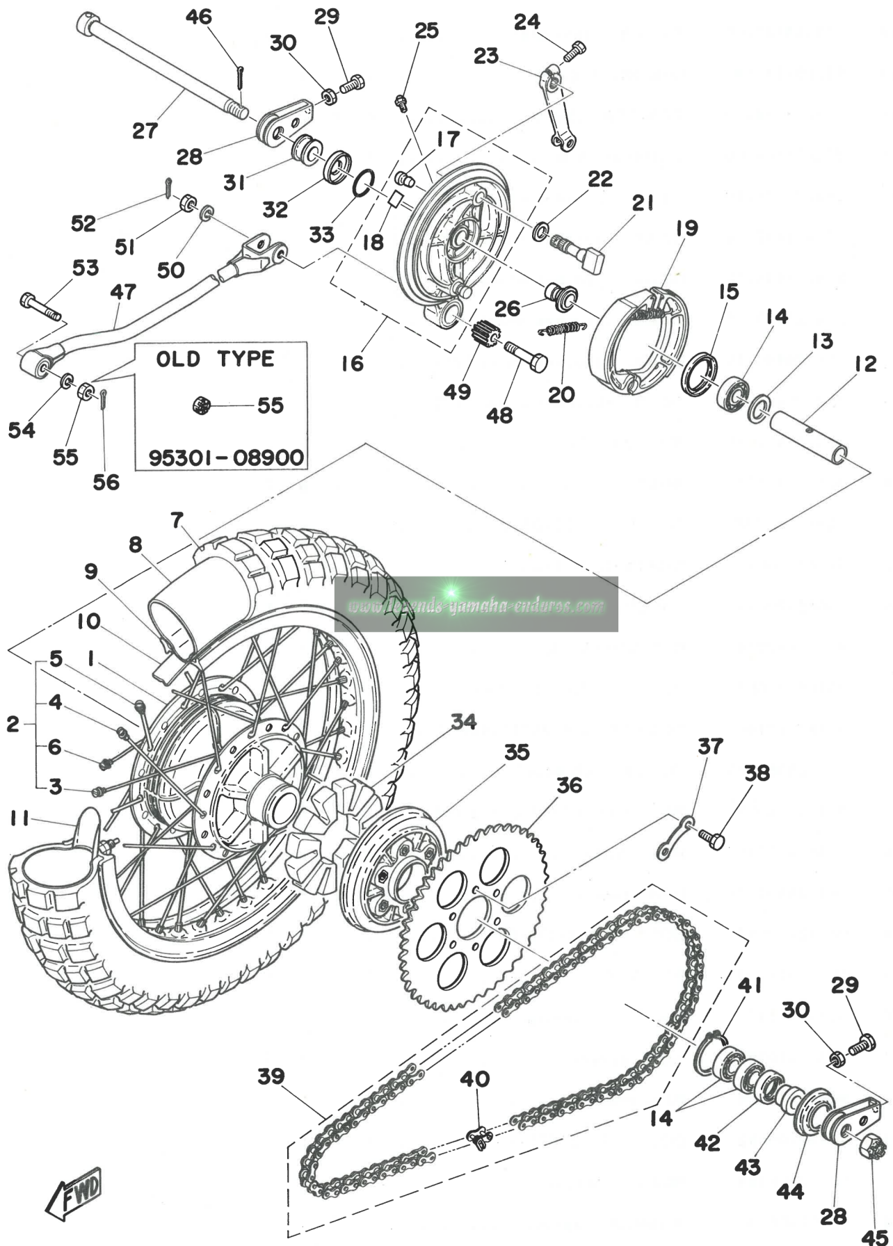
Fig. 30 REAR WHEEL
