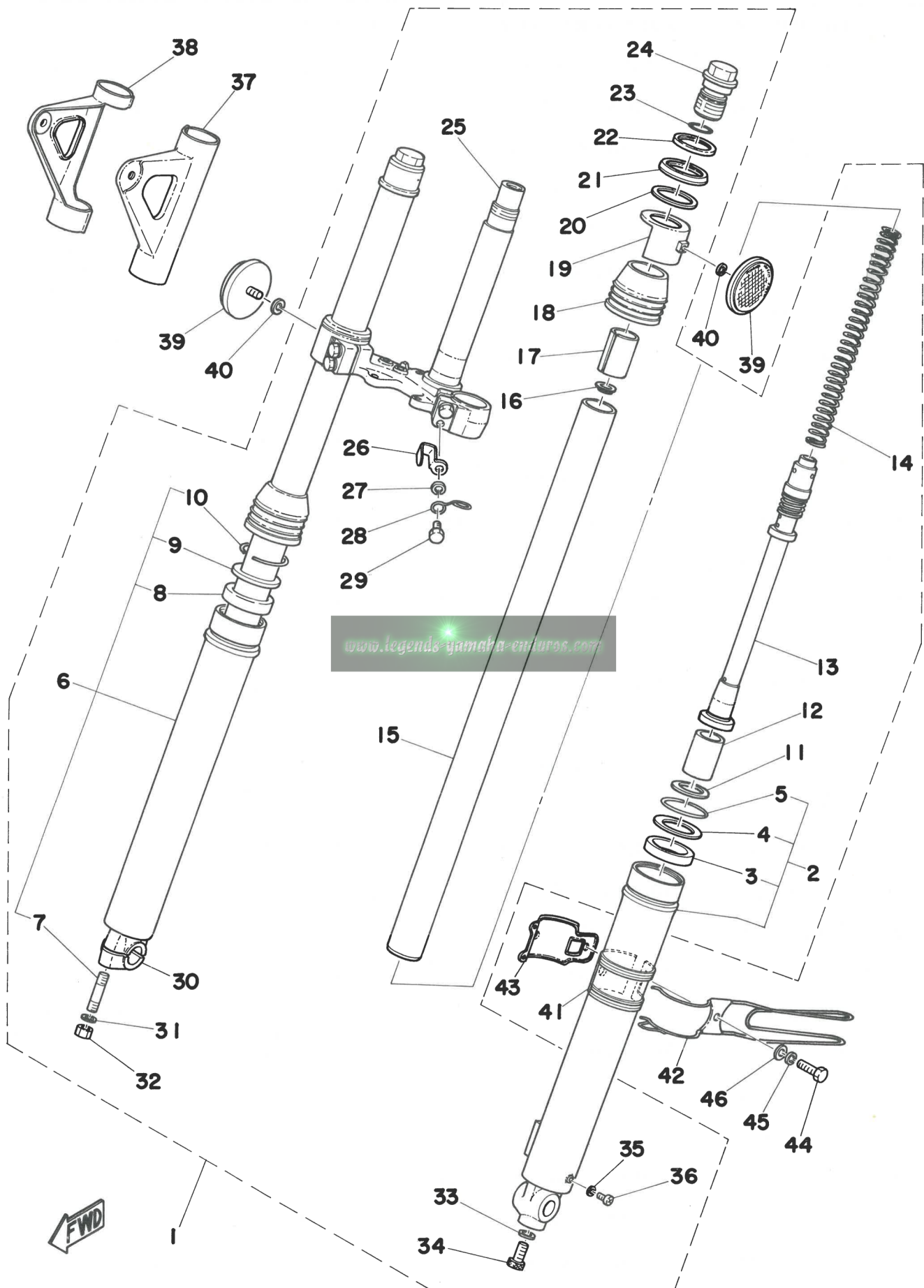
Fig. 23 FRONT FORK
