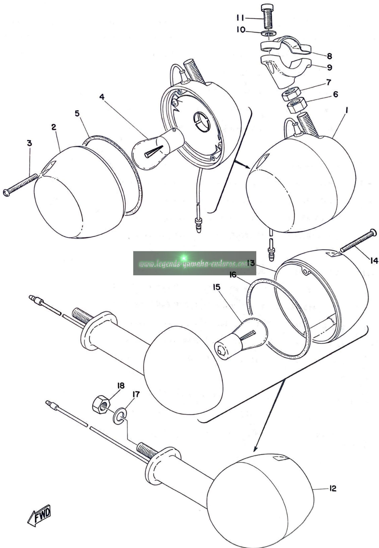
Fig. 6 FLASHER LAMP
