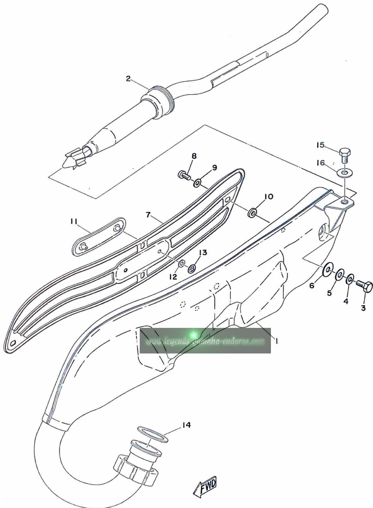
Fig. 11 EXHAUST
