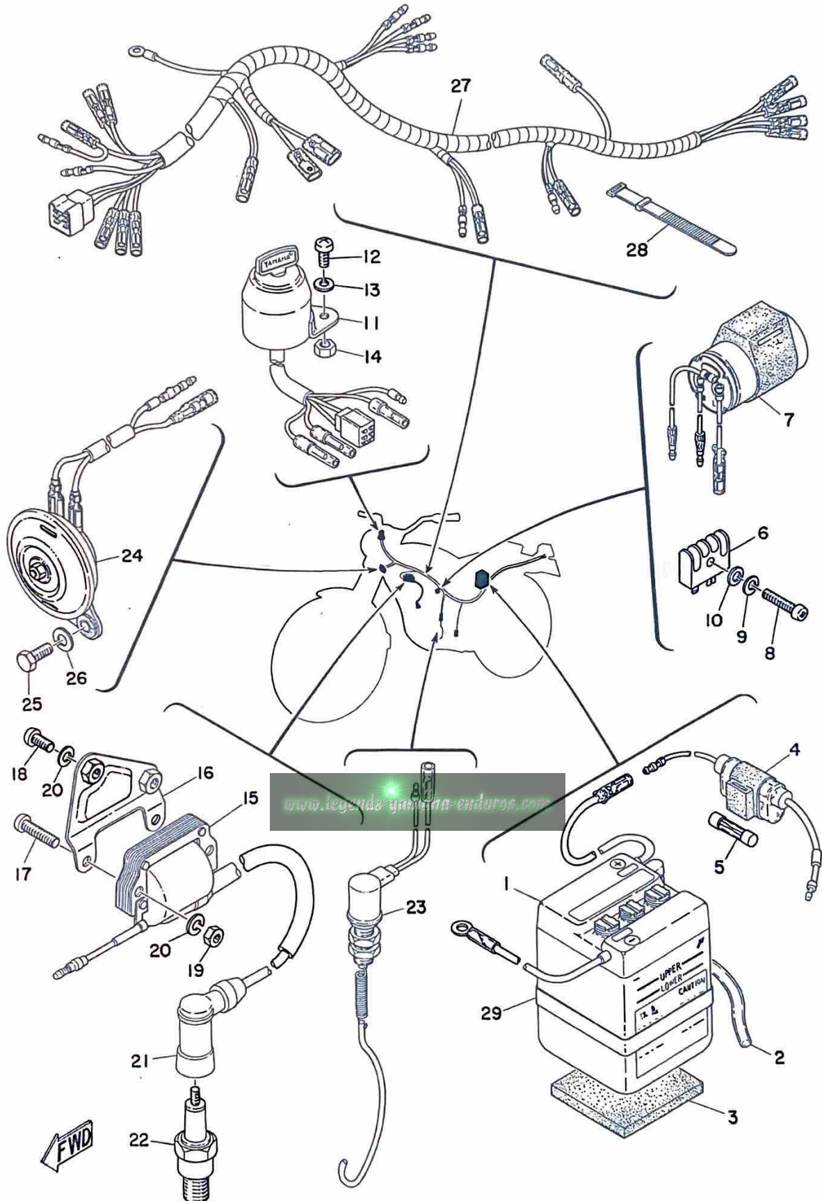
Fig. 29 ELECTRICAL
