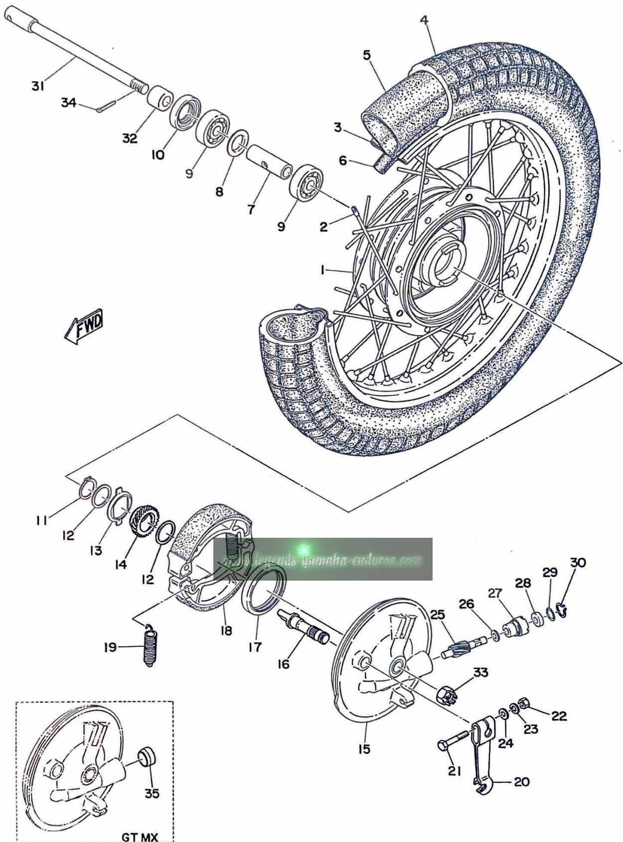
Fig. 24 FRONT WHEEL
