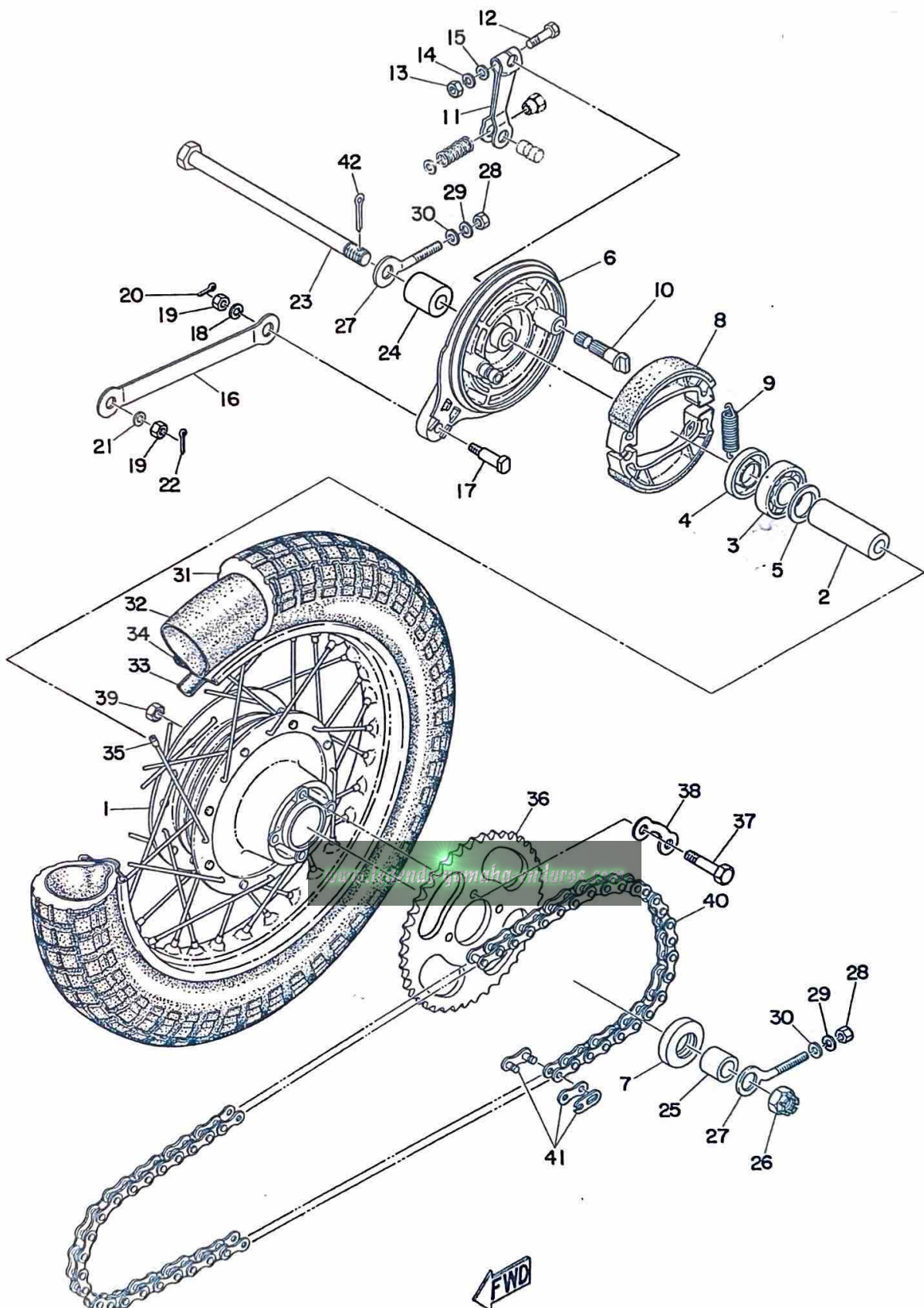
Fig. 25 REAR WHEEL
