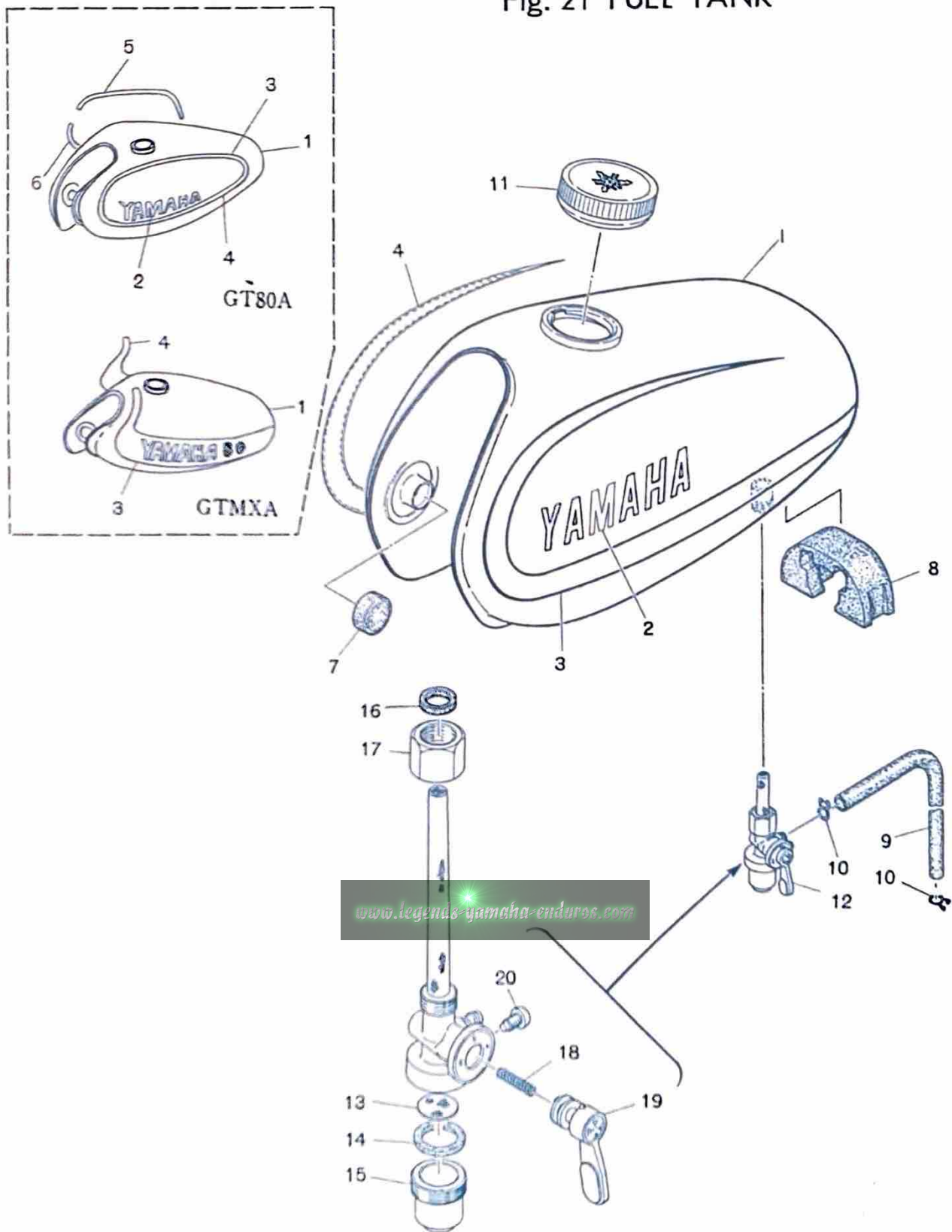
Fig. 21 FUEL TANK
