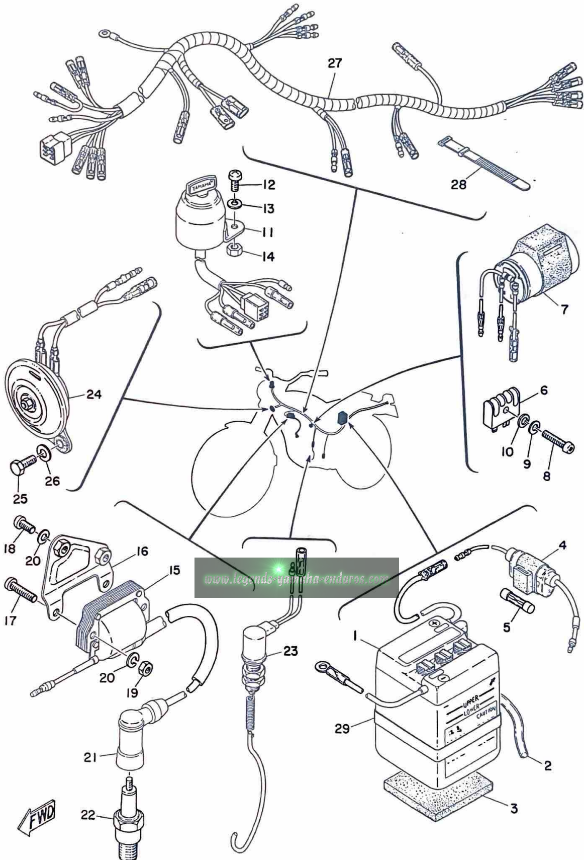
Fig. 29 ELECTRICAL
