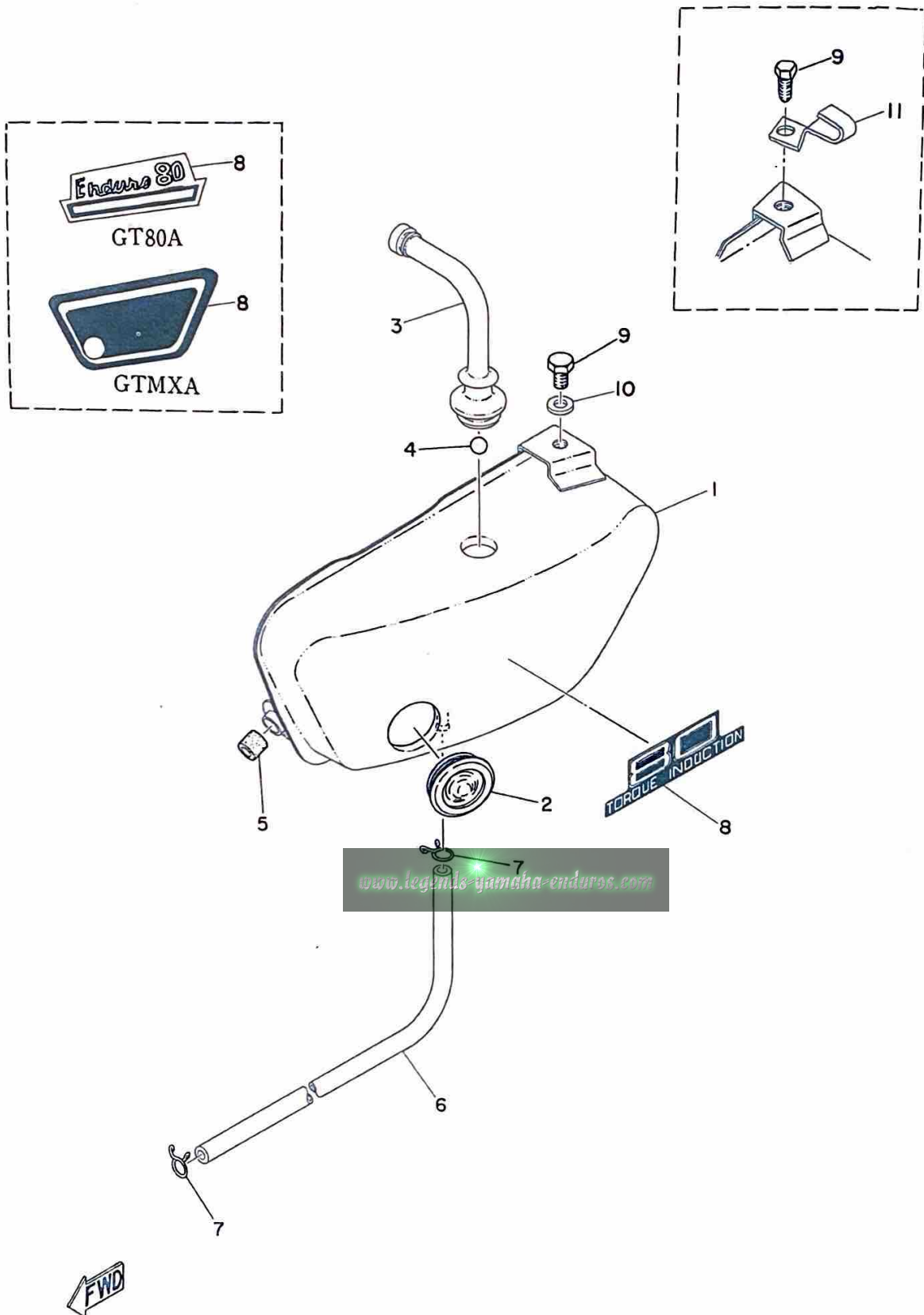
Fig. 22 OIL TANK
