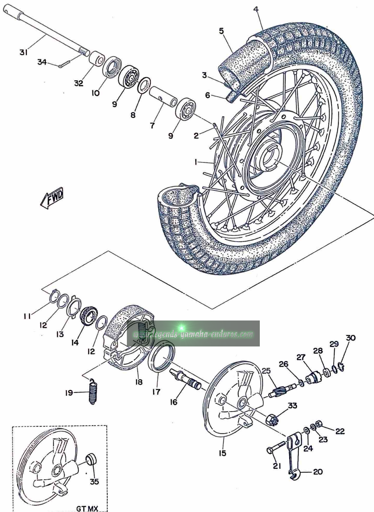
Fig. 24 FRONT WHEEL
