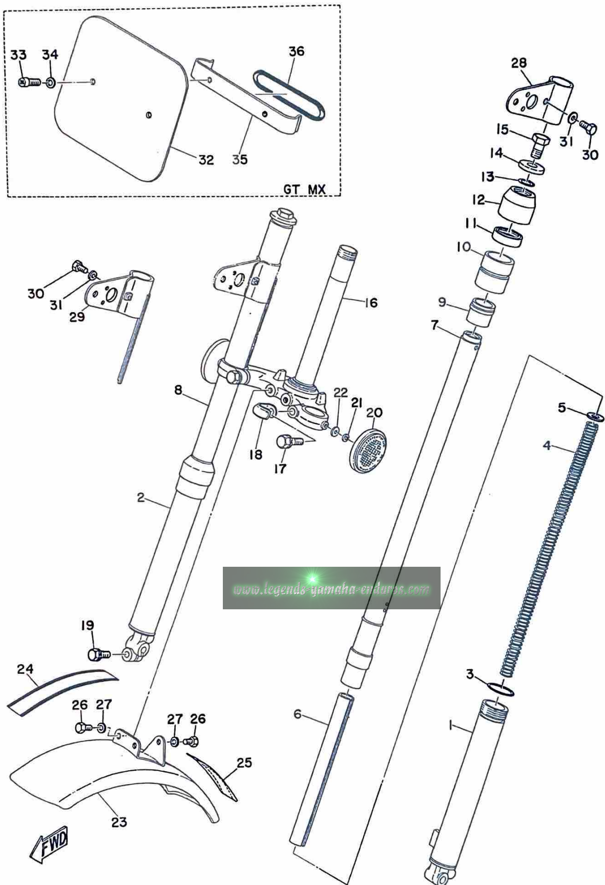
Fig. 18 FRONT FORK · FRONT FENDER
