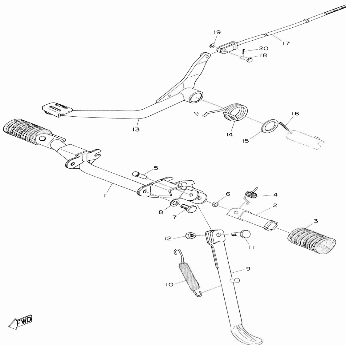
Fig. 18 STAND, FOOT REST & REAR BRAKE PEDAL
