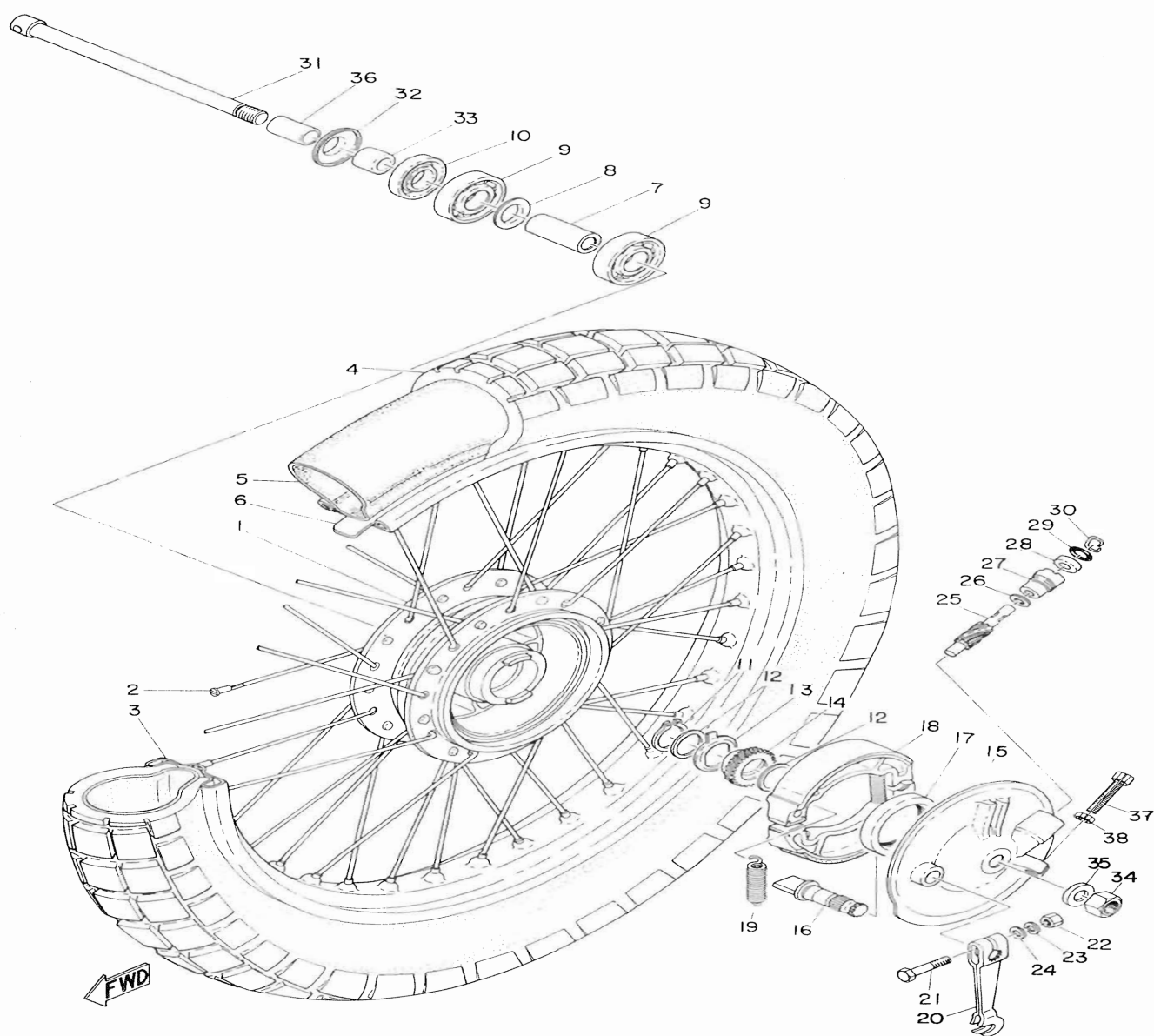
Fig. 25 FRONT WHEEL
