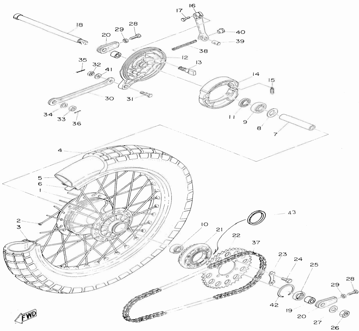
Fig. 26 REAR WHEEL
