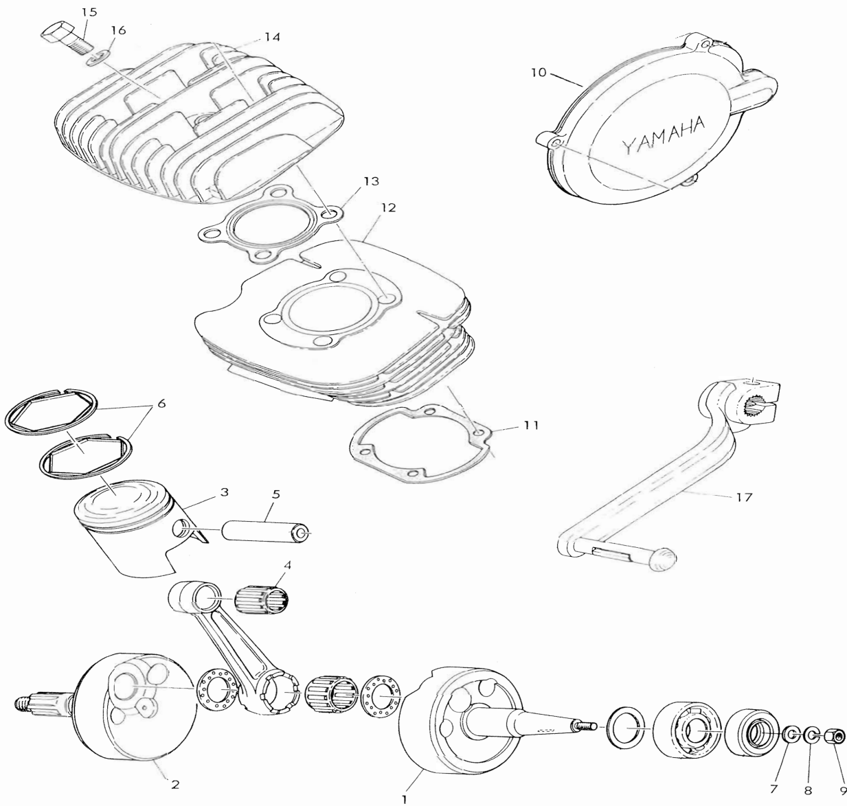
Fig. 1 ENGINE (Miscellaneous)
