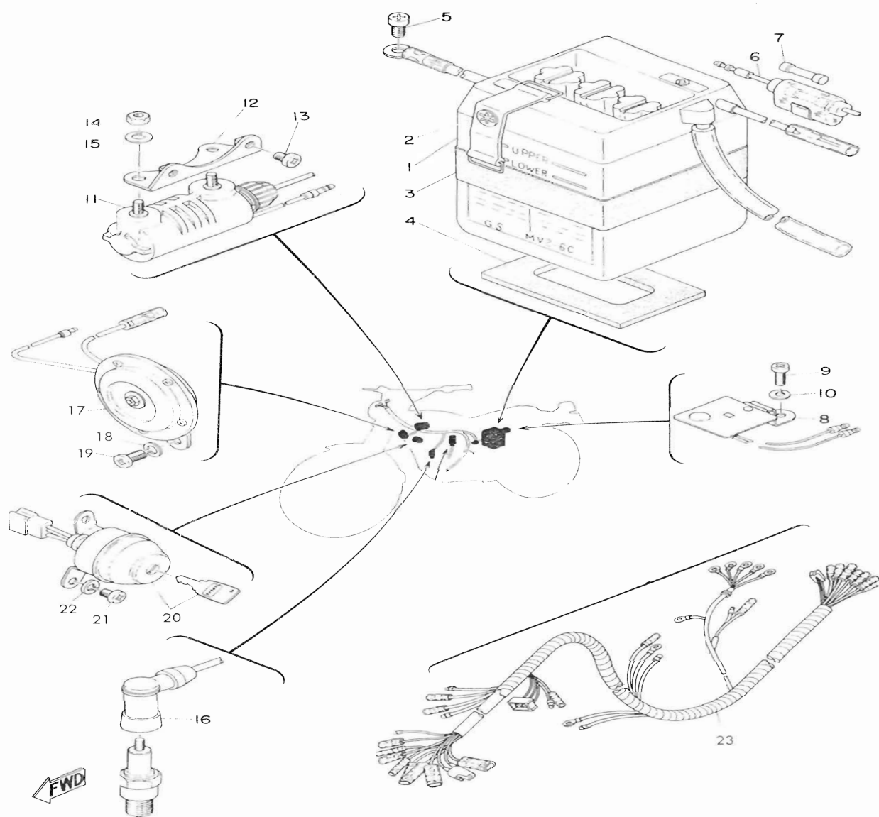
Fig. 6 ELECTRICAL
