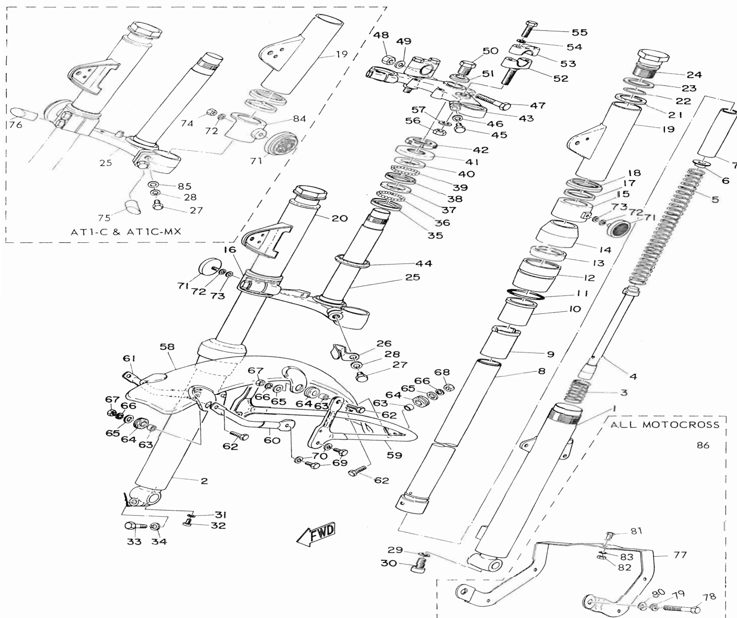
Fig. 19 FRONT FORK & FRONT FENDER
