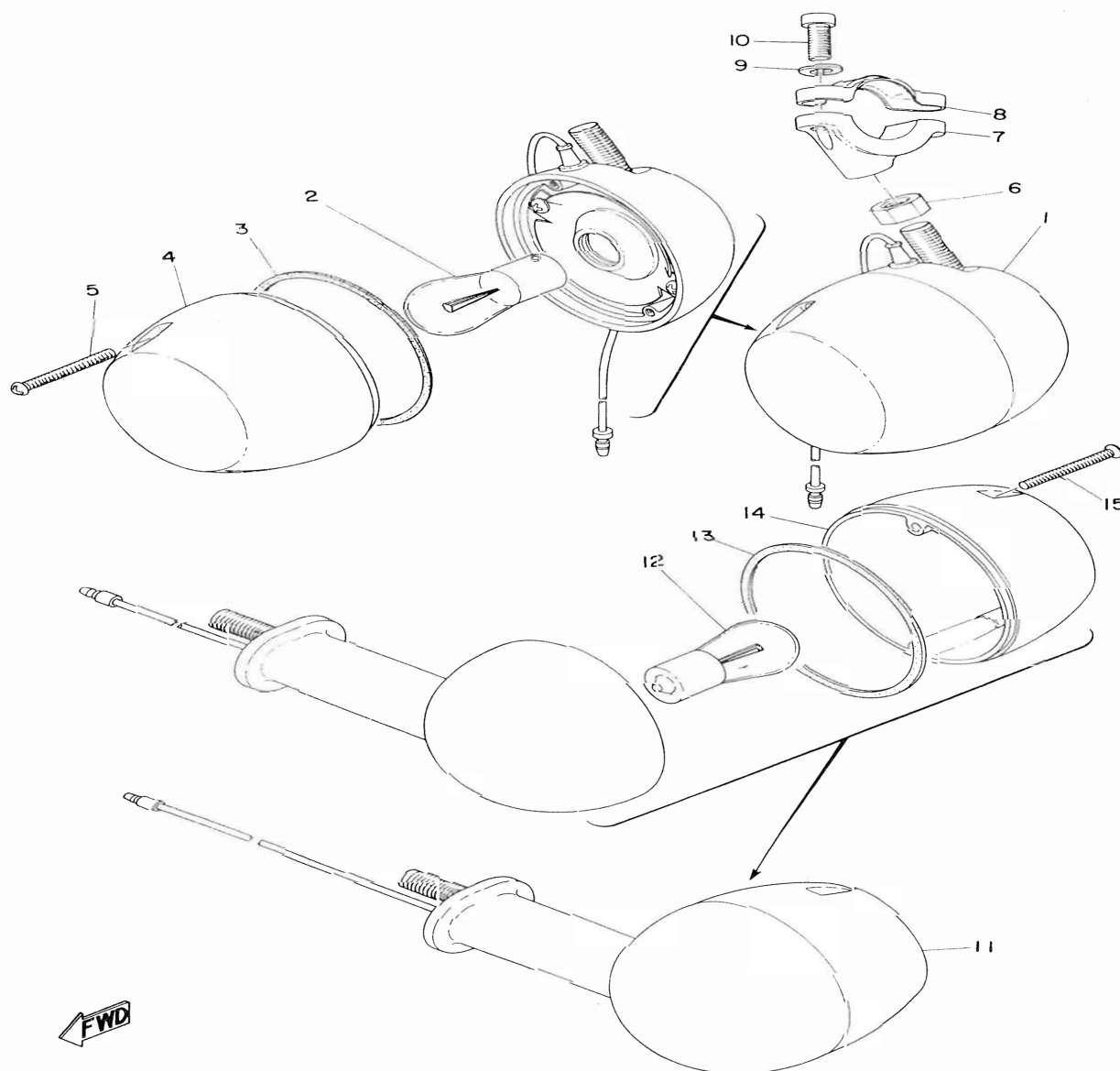
Fig.30 FLASHER LAMP (AT1C)
