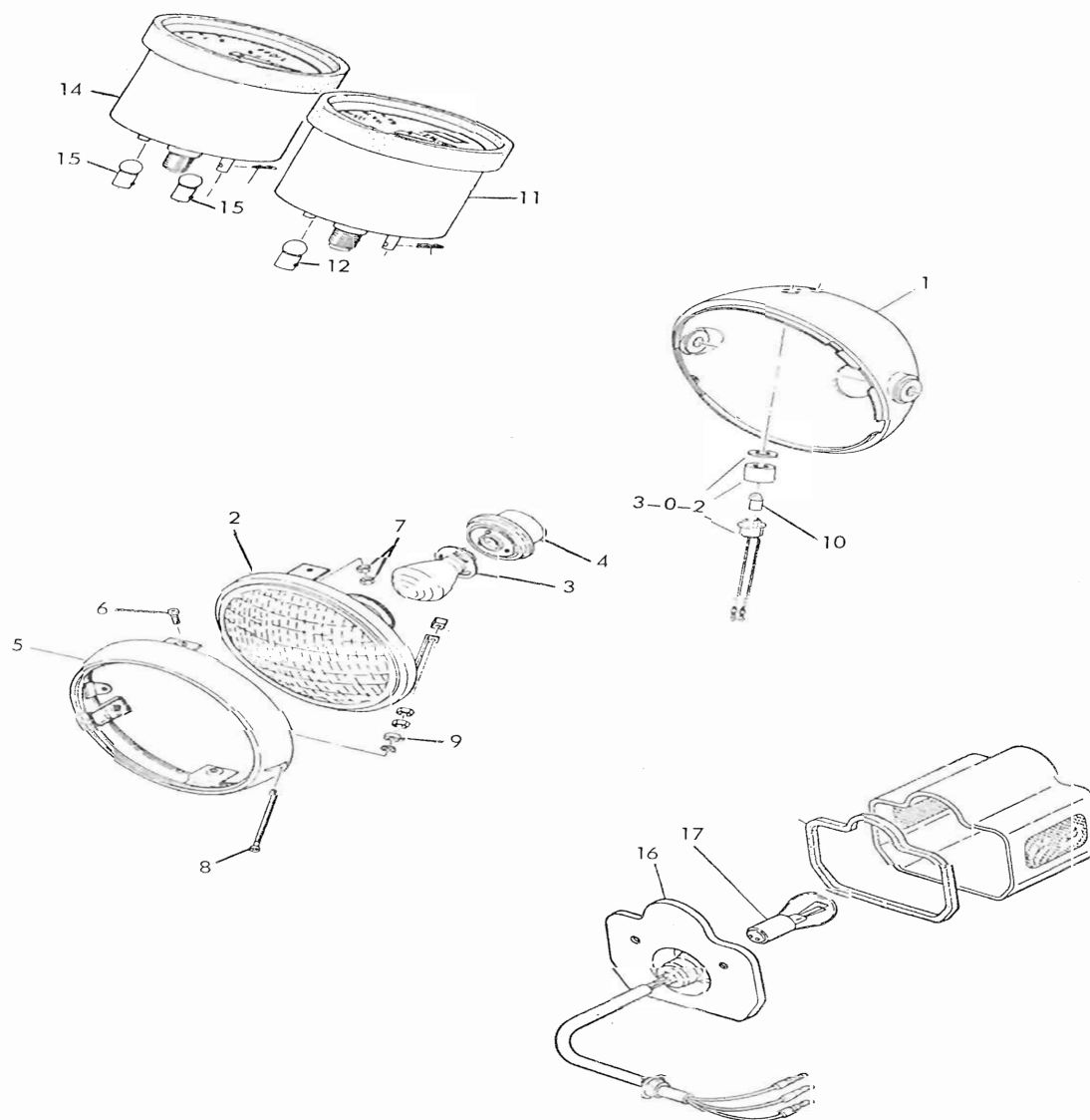
Fig. 3 HEAD & TAIL LAMPS, SPEEDOMETER & TACHOMETER (CT1A & CT1B)
