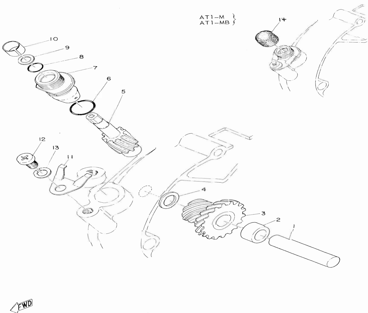
Fig. 9 TACHOMETER GEAR
