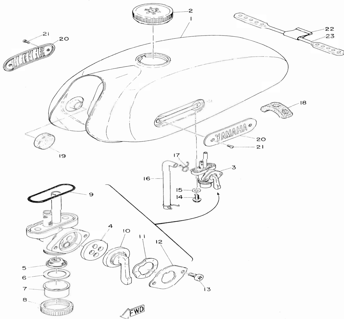
Fig. 22 FUEL TANK
