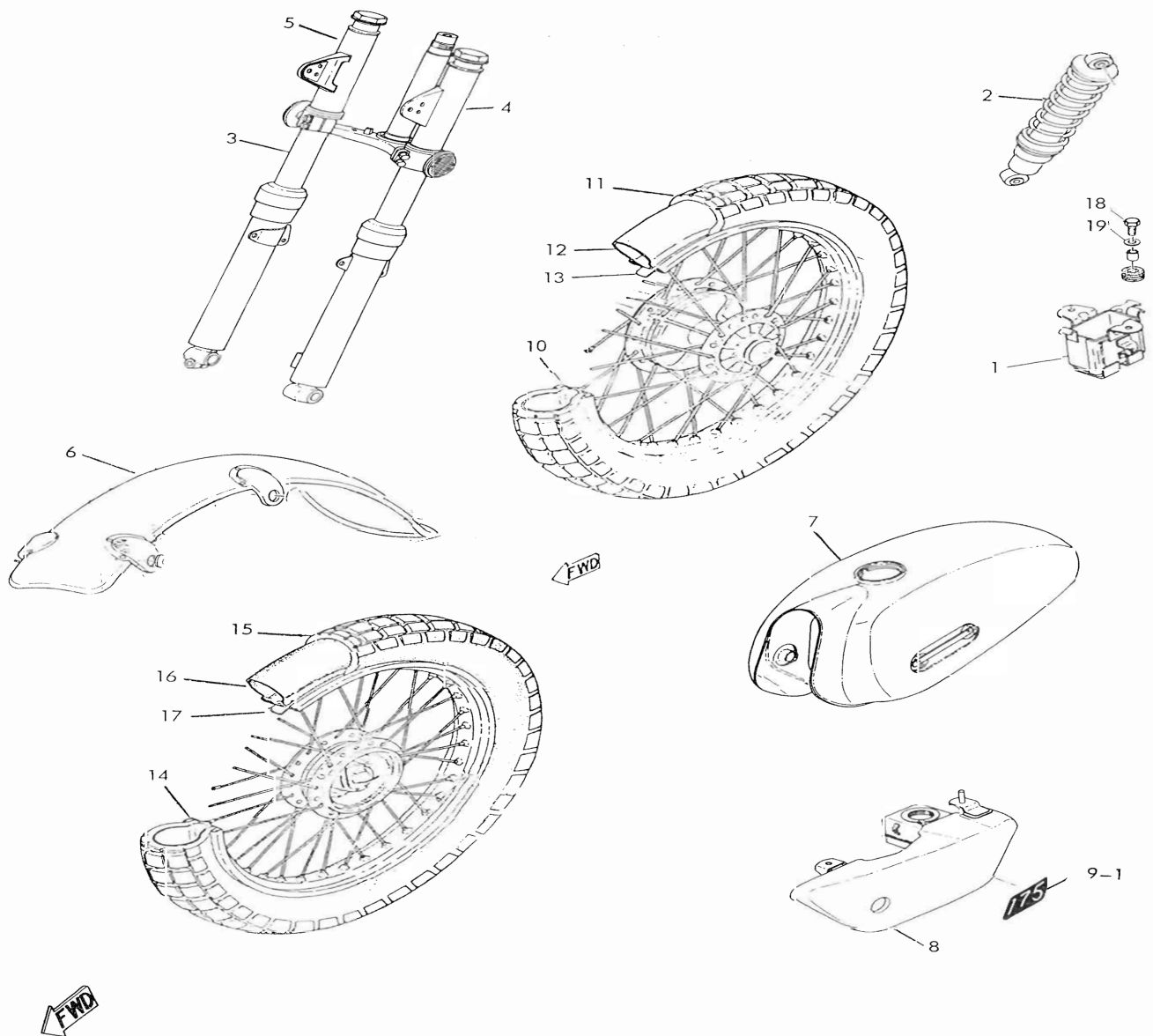
Fig. 2 CHASSIS (Miscellaneous)
