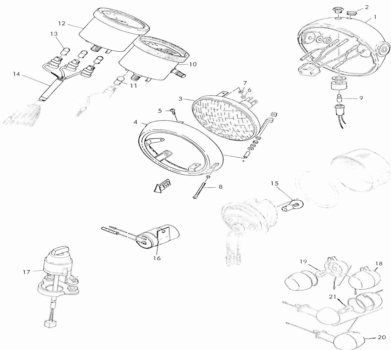
Fig. 4 SPEEDOMETER, TACHOMETER, SWITCH & LAMPS (CT1B & CT1C)
