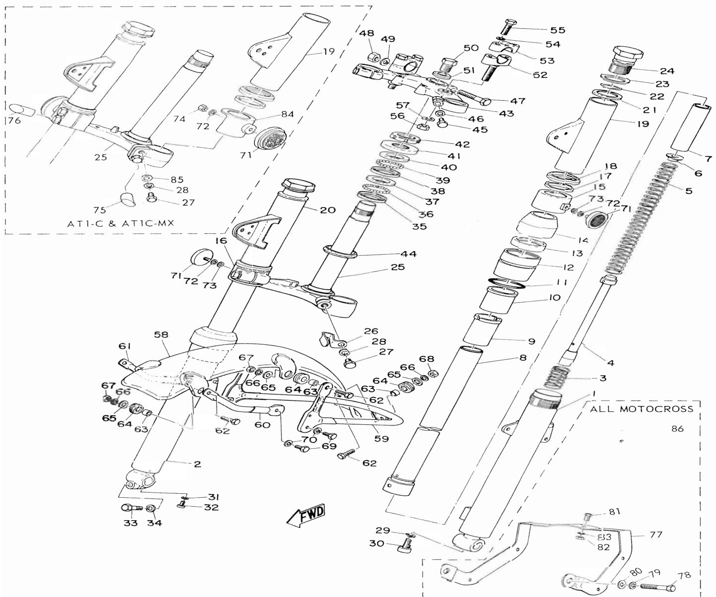
Fig. 19 FRONT FORK & FRONT FENDER
