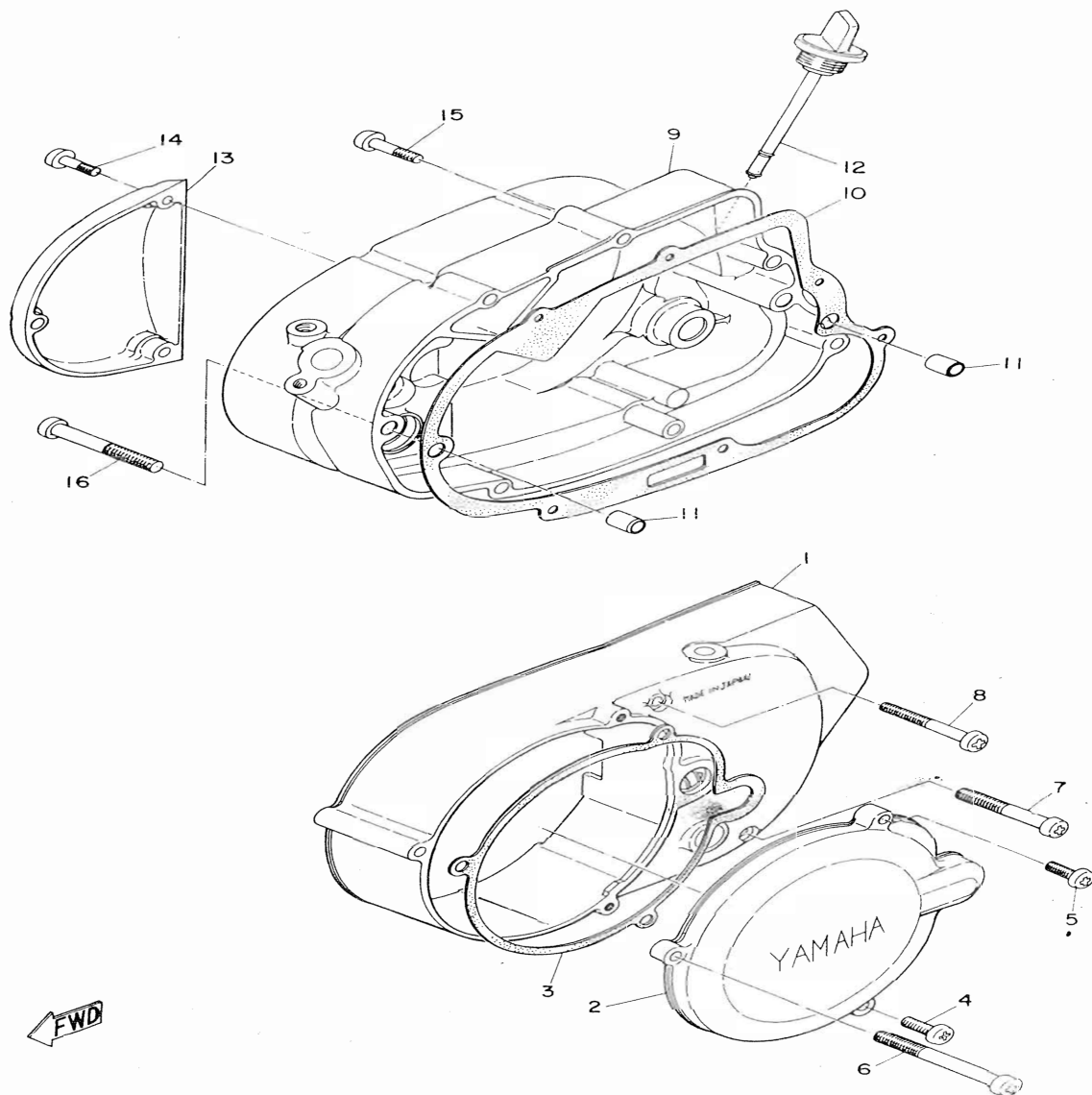
Fig. 2 CRANKCASE COVER
