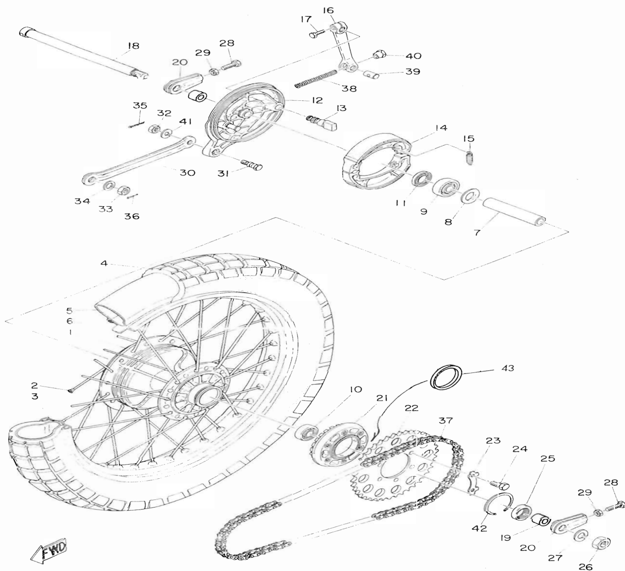
Fig. 26 REAR WHEEL
