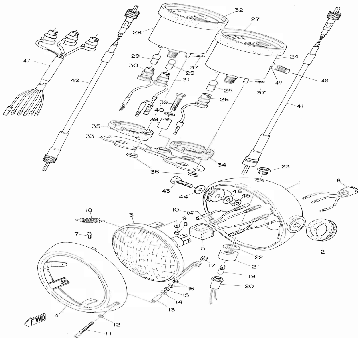
Fig. 27 HEAD LAMP , SPEEDOMETER & TACHOMETER
