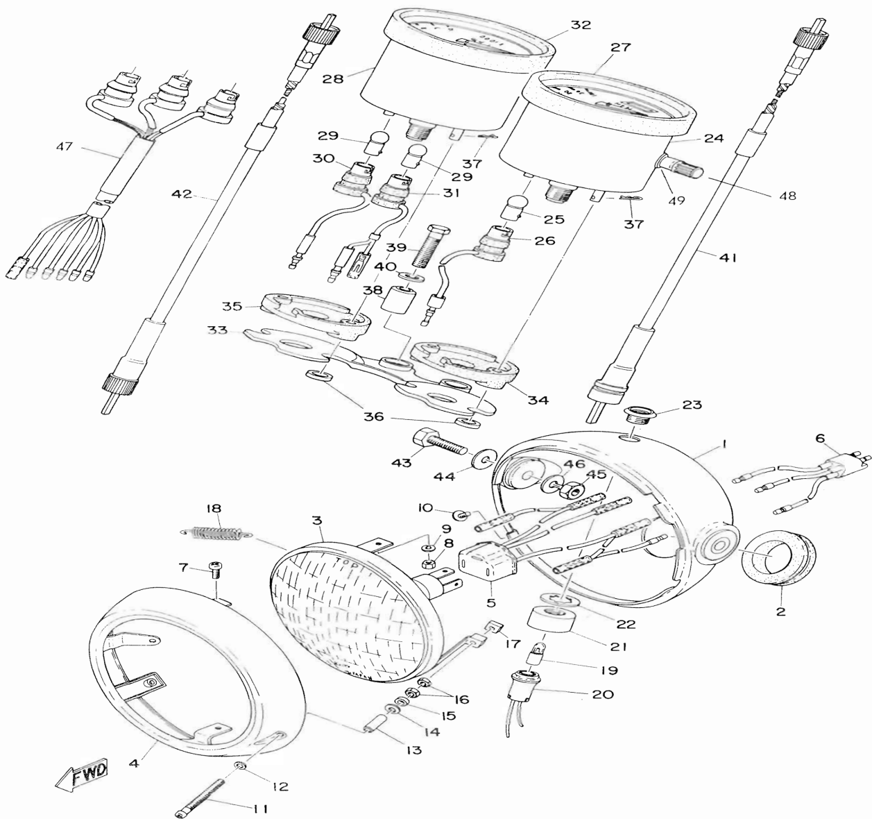
Fig. 27 HEAD LAMP , SPEEDOMETER & TACHOMETER
