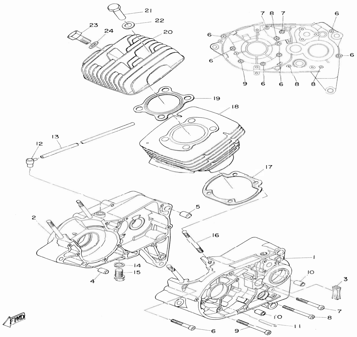
Fig. 1 CRANKCASE
