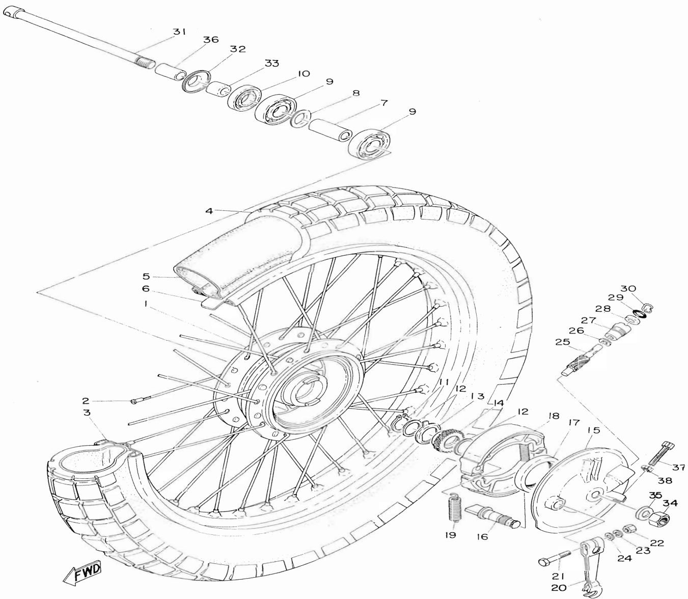
Fig. 25 FRONT WHEEL
