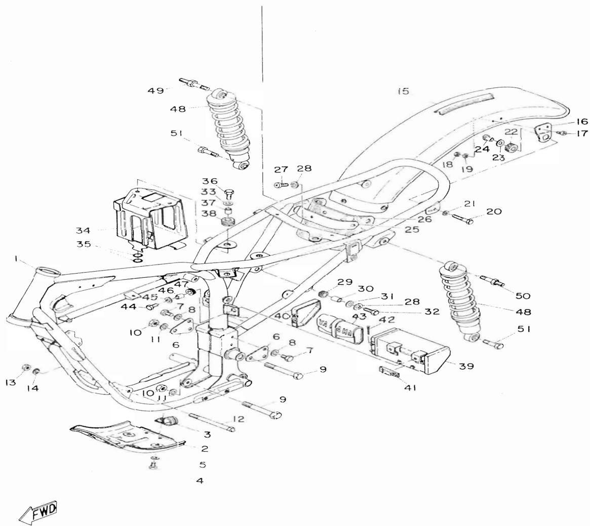
Fig. 16 FRAME & REAR FENDER
