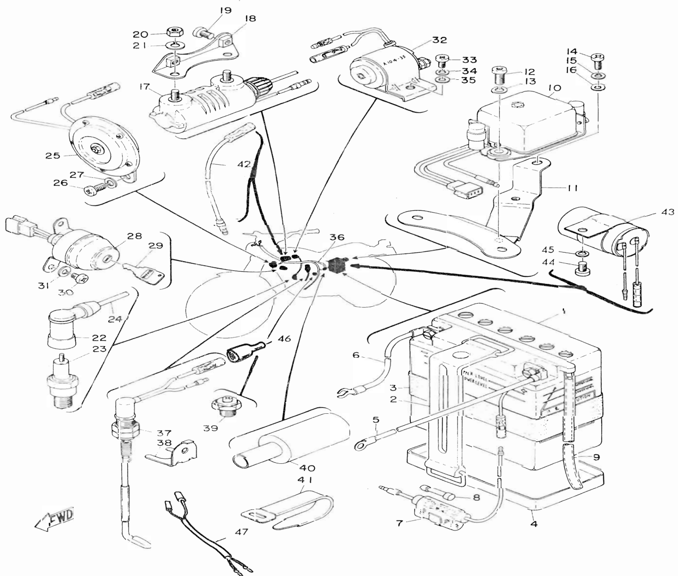
Fig. 31 ELECTRICAL
