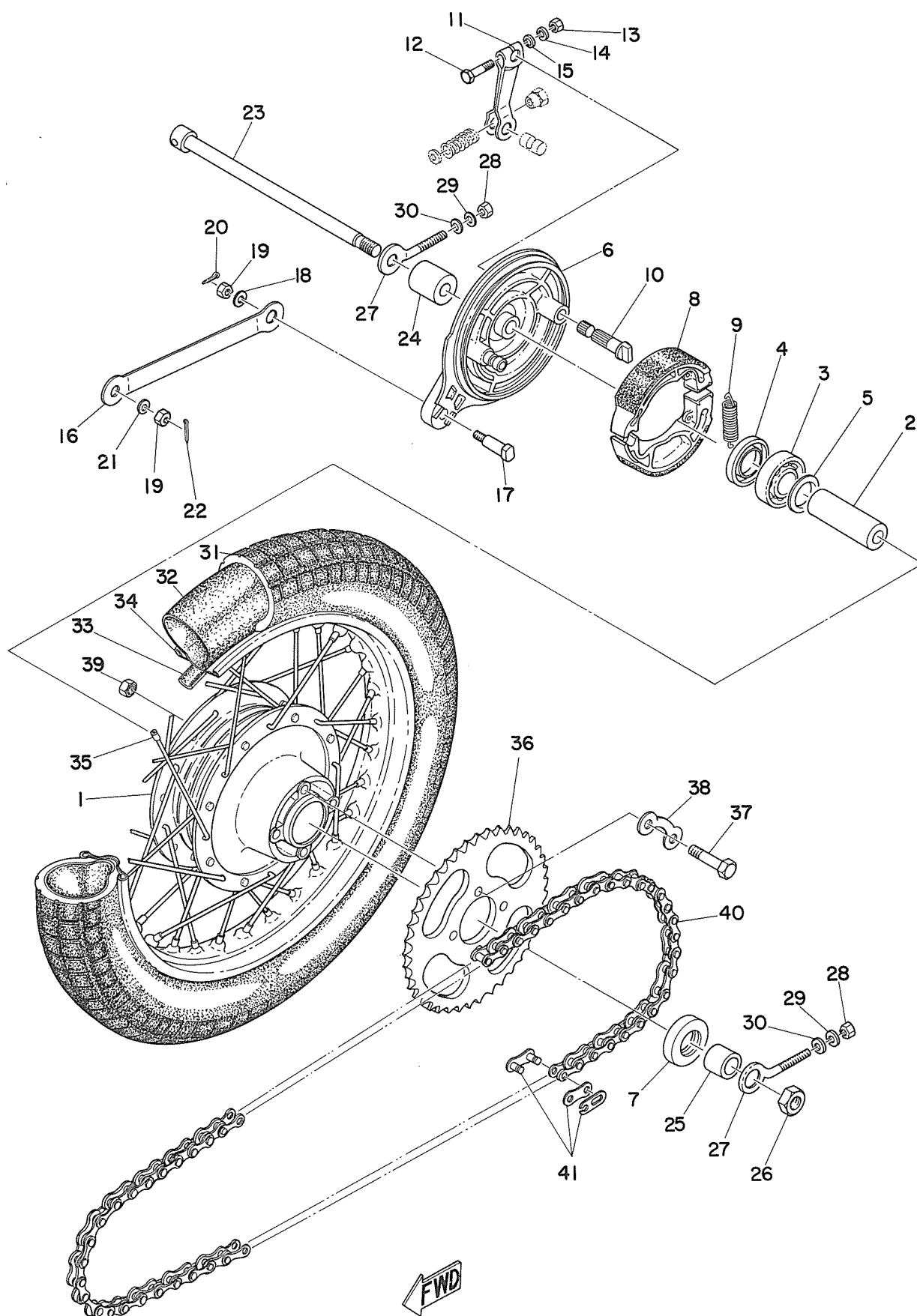
Fig. 24 REAR WHEEL
