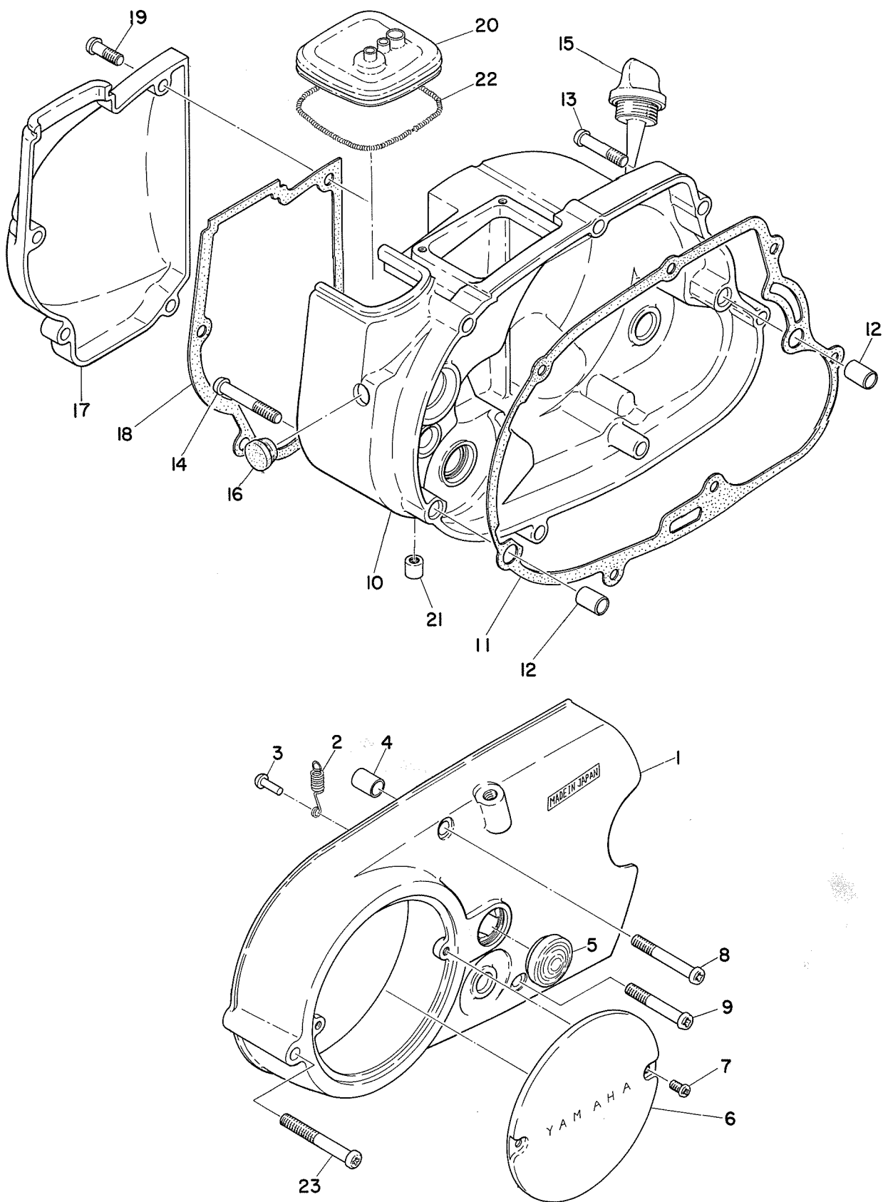
Fig. 2 CRANKCASE COVER
