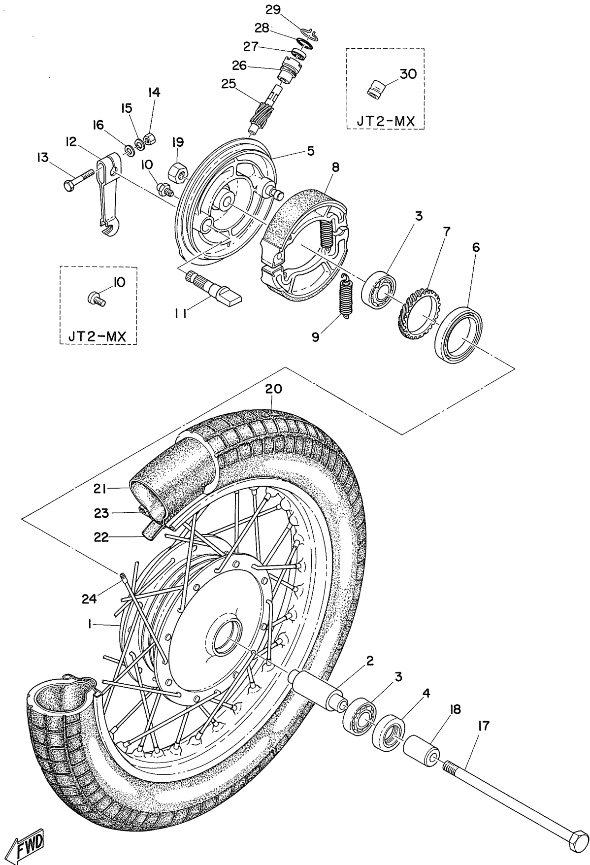
Fig. 23 FRONT WHEEL
