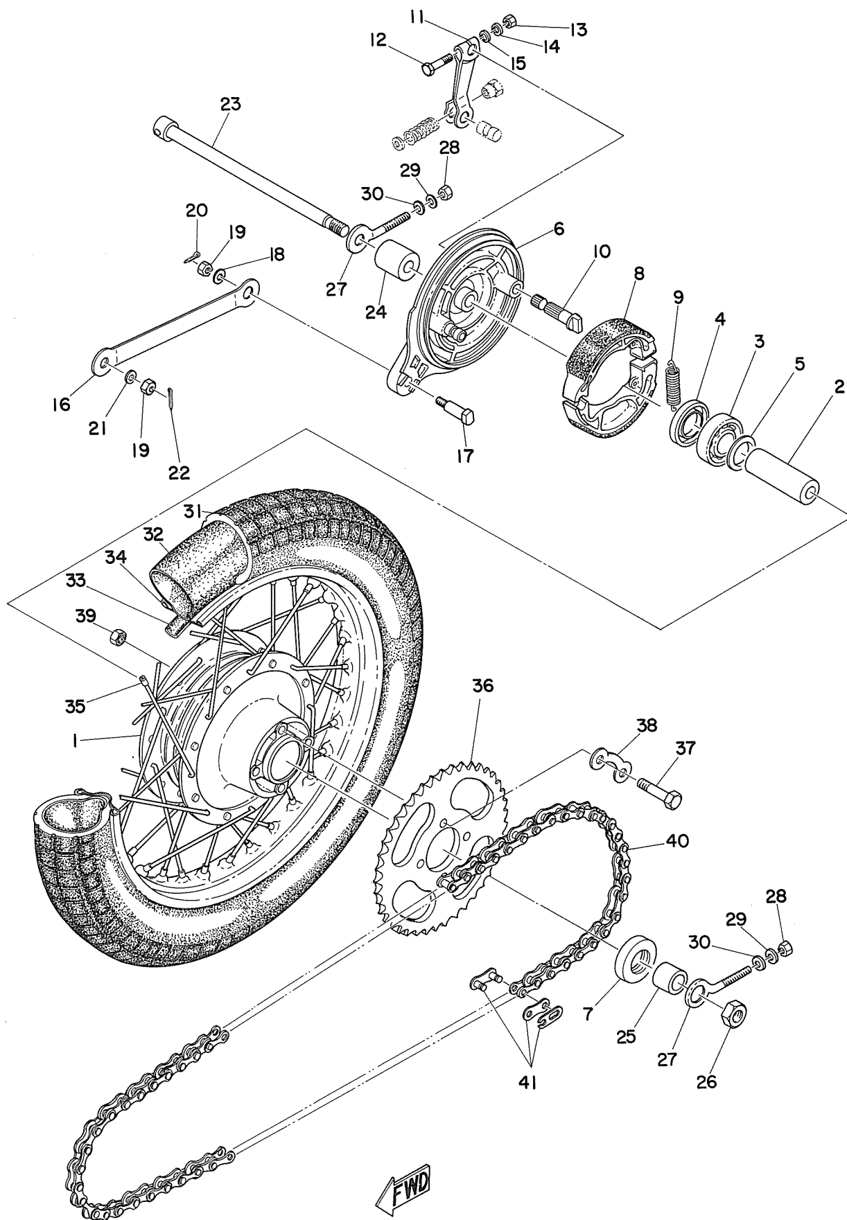
Fig. 24 REAR WHEEL
