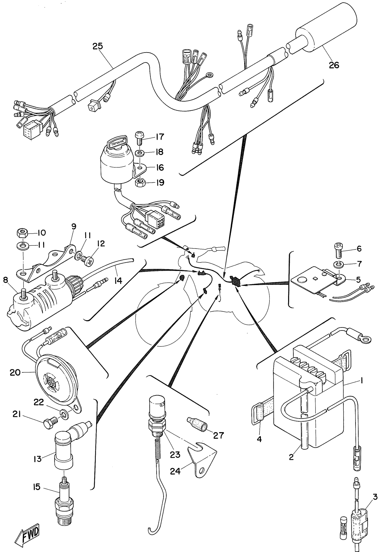
Fig. 27 ELECTRICAL
