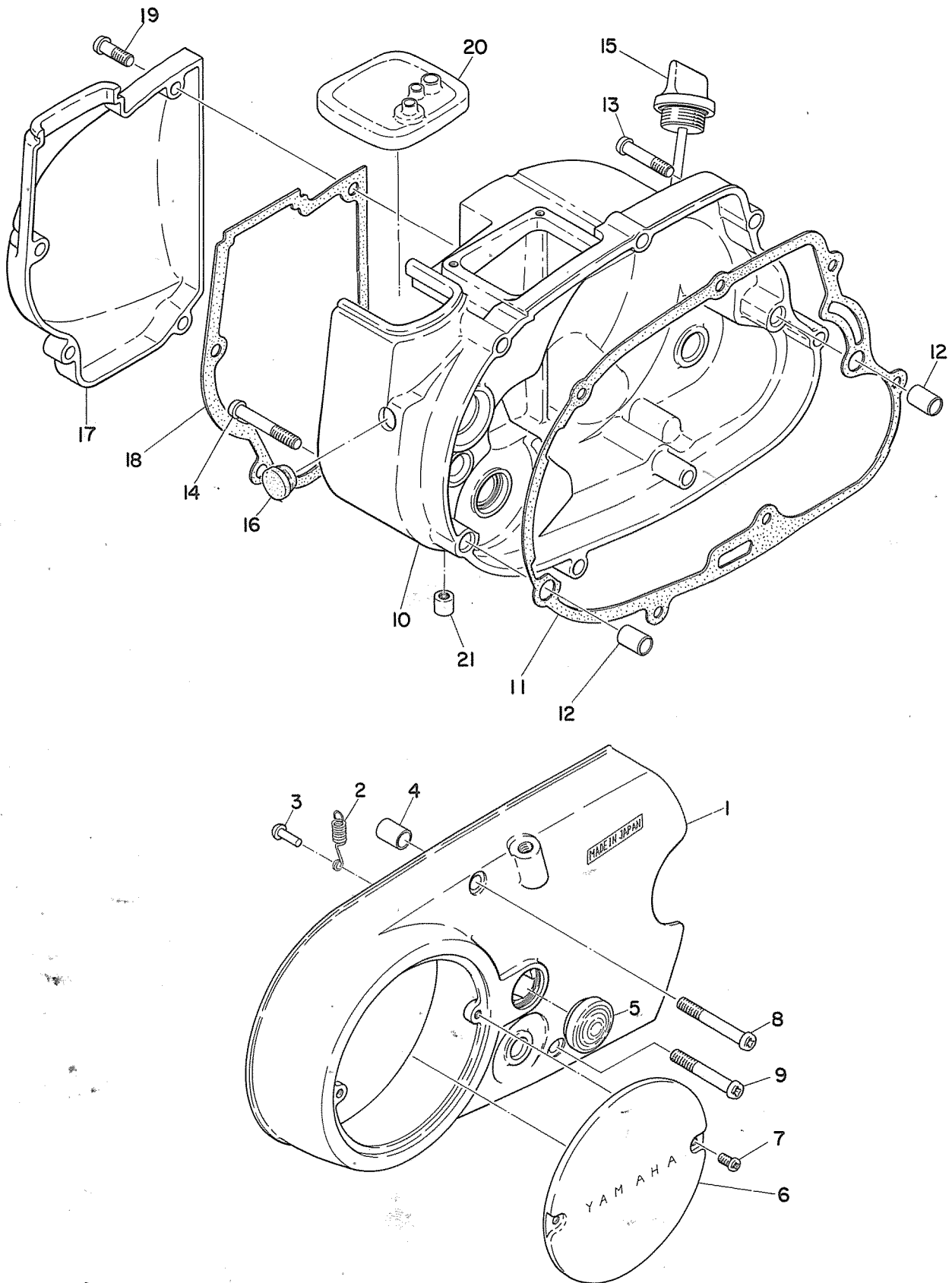
Fig. 2 CRANKCASE COVER
