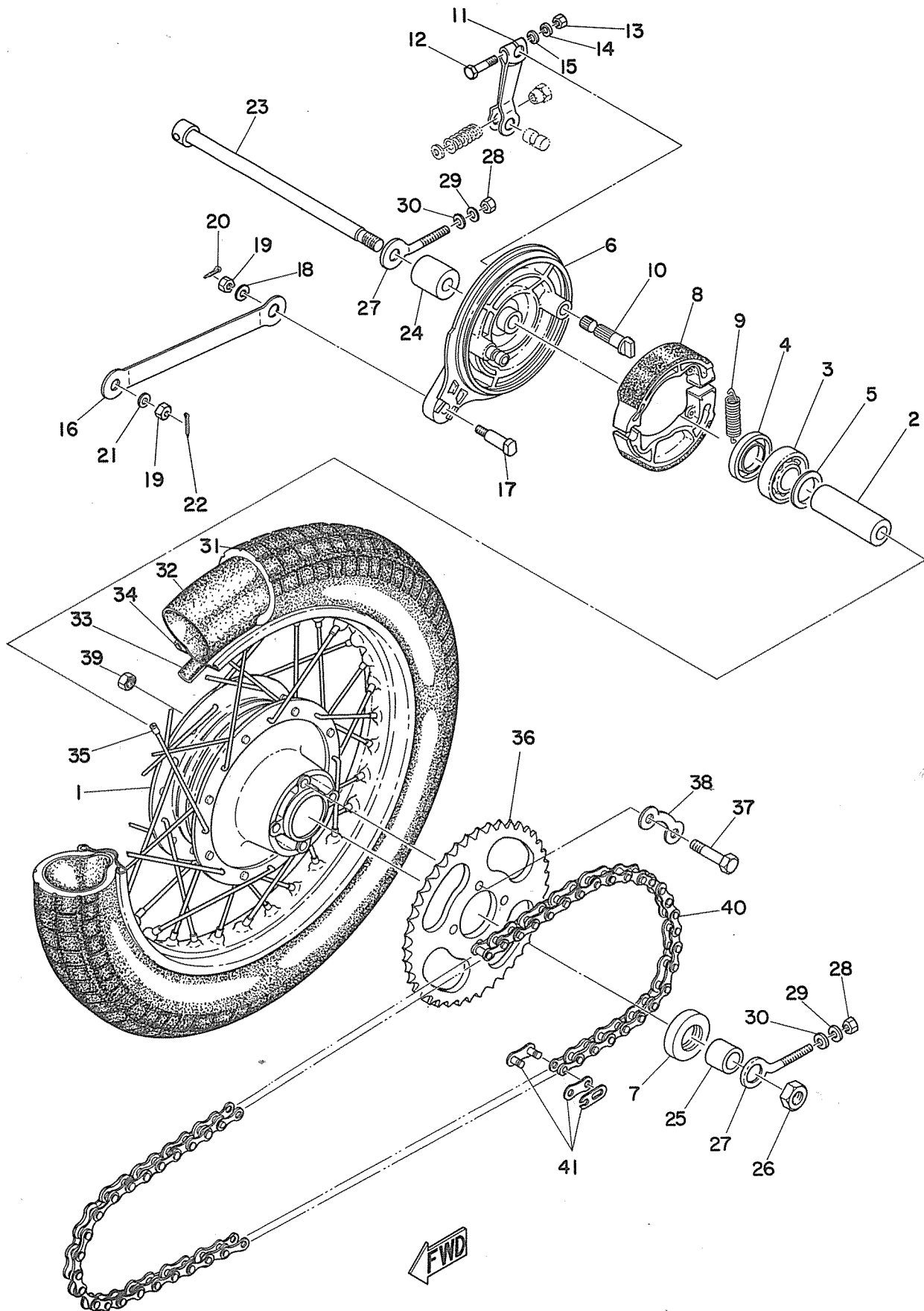
Fig. 24 REAR WHEEL
