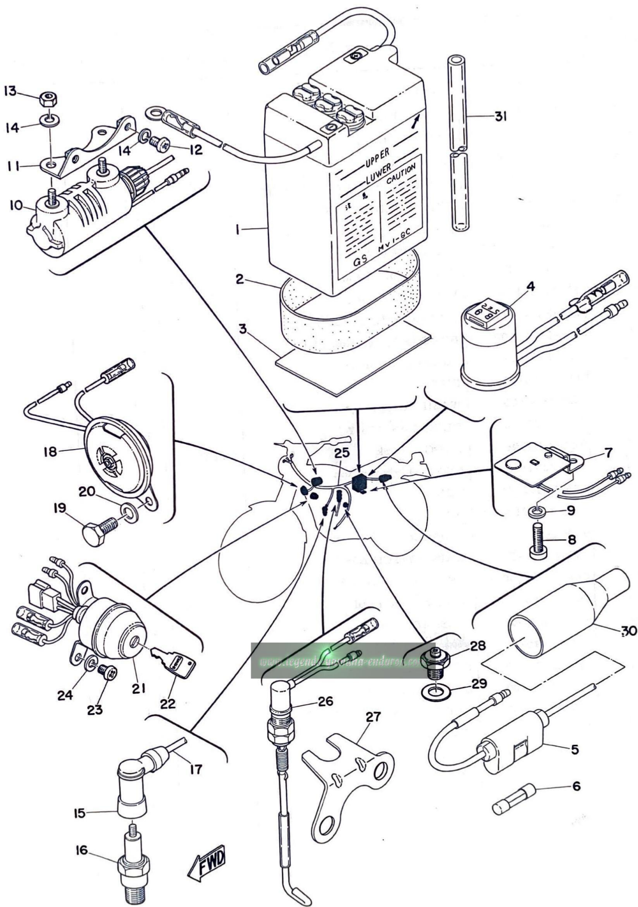
Fig. 26 ELECTRICAL
