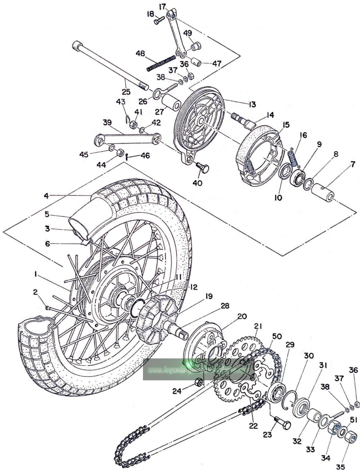
Fig. 23 REAR WHEEL
