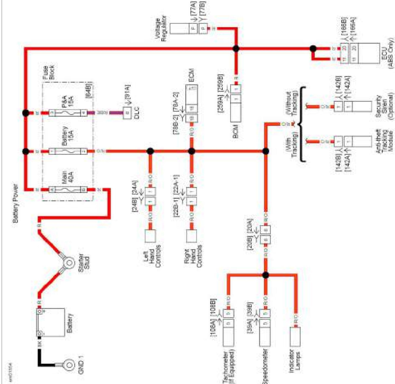
Battery Power Distribution
