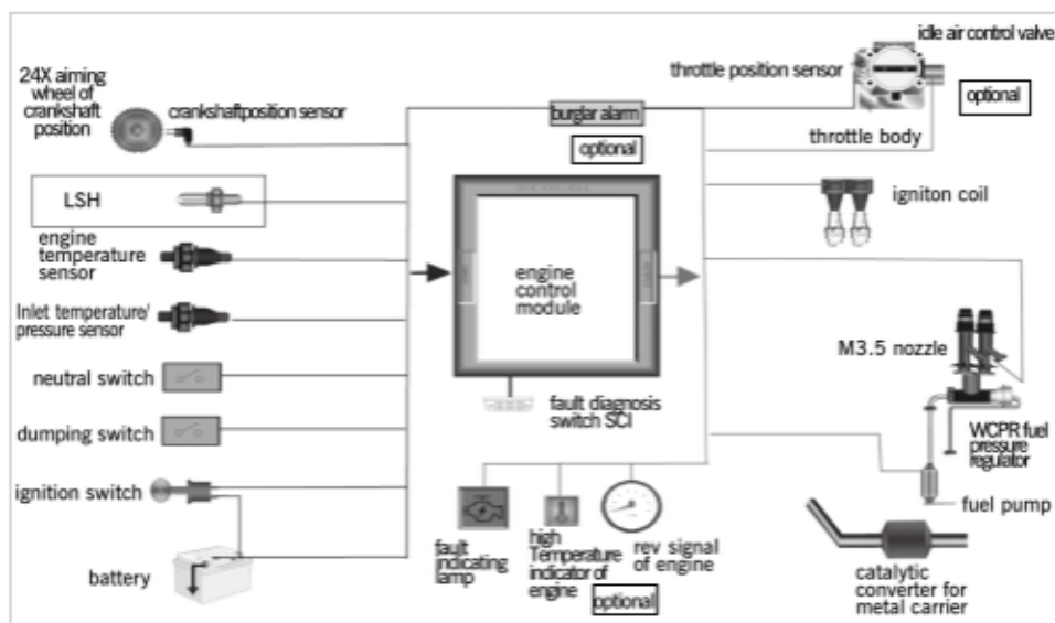
Structural drawing of EFI system
