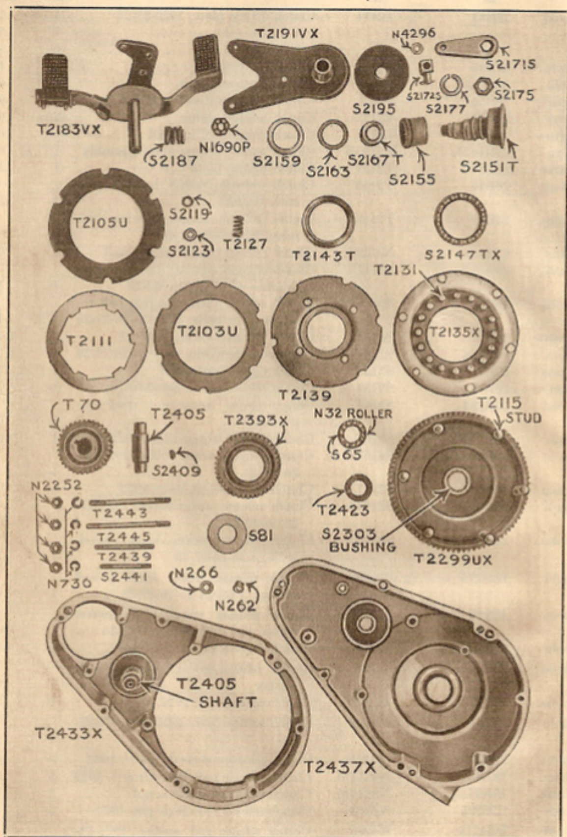
Clutch Group
