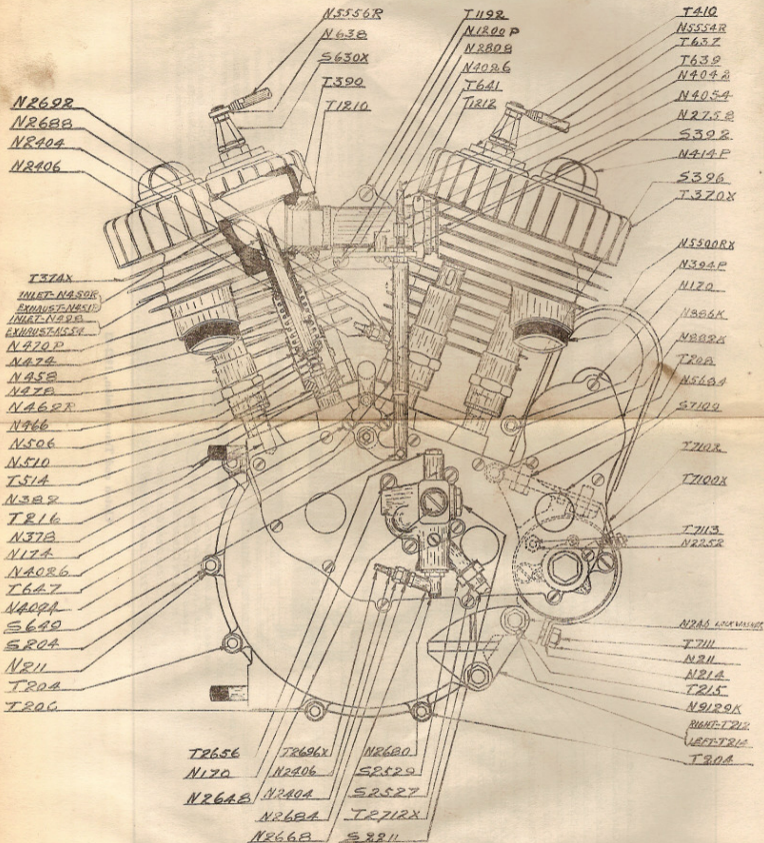
Sectional View Chief Motor, Model H
