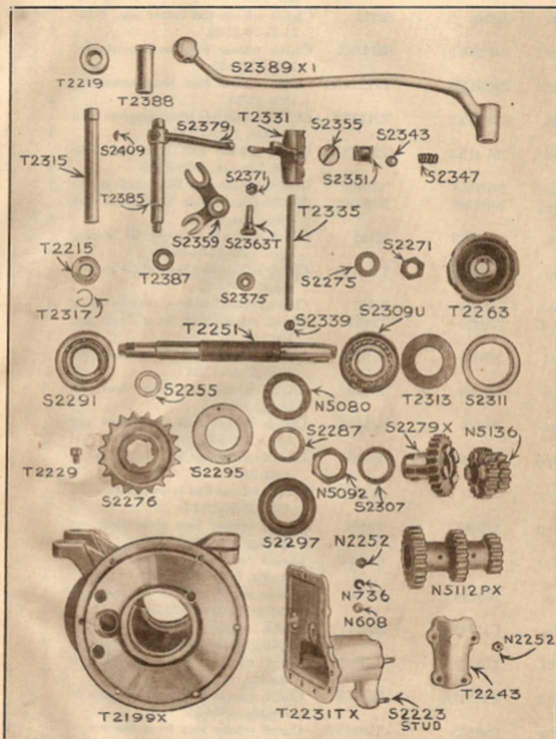
Transmission Group
