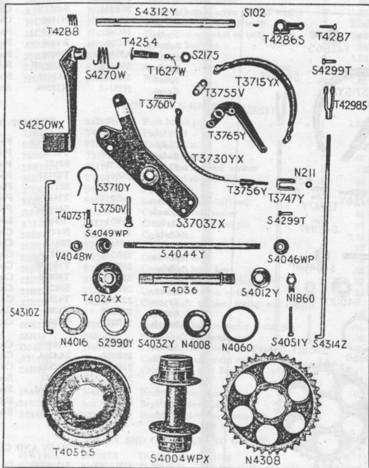
Brake Group
