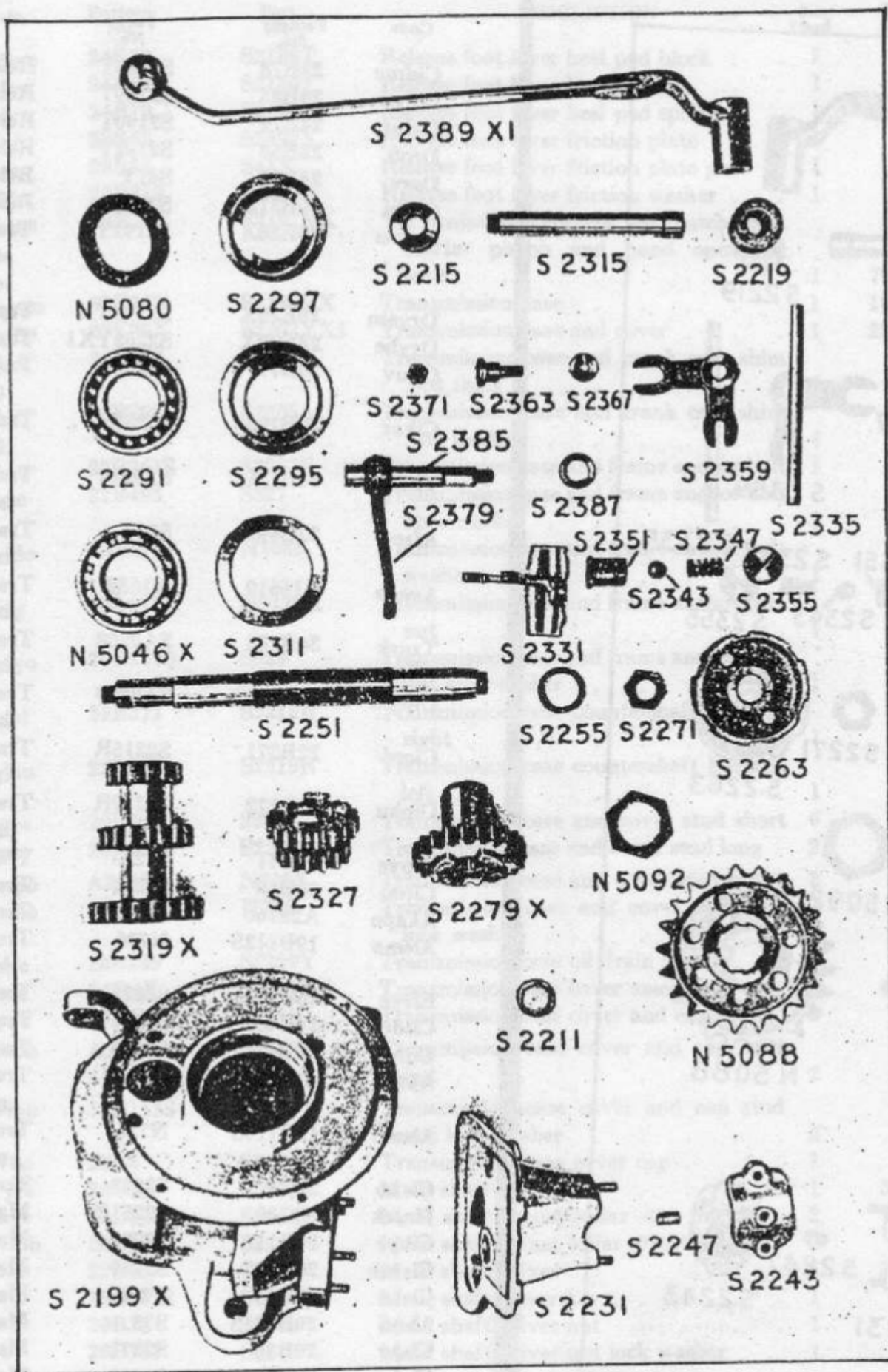
Transmission Group
