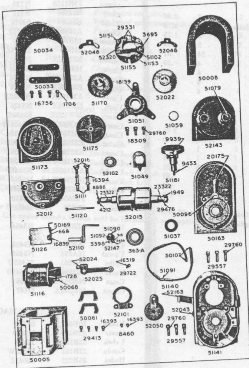
Magneto Group
