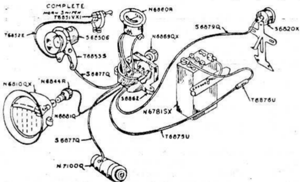
Wiring Diagram 1926
