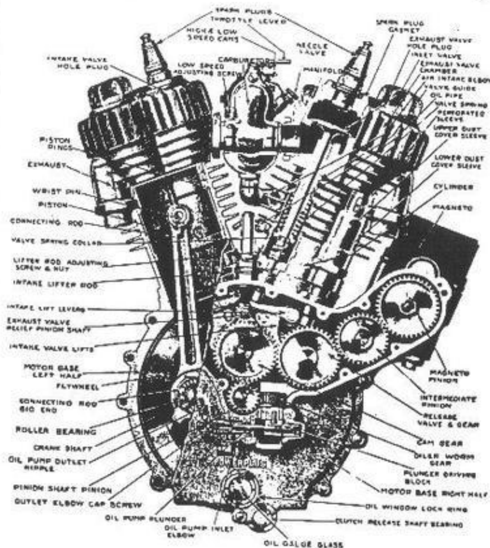
Sectional View Powerplus Motor
