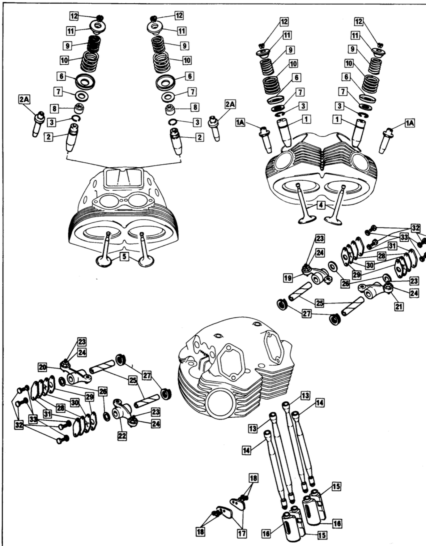
Valve Gear
