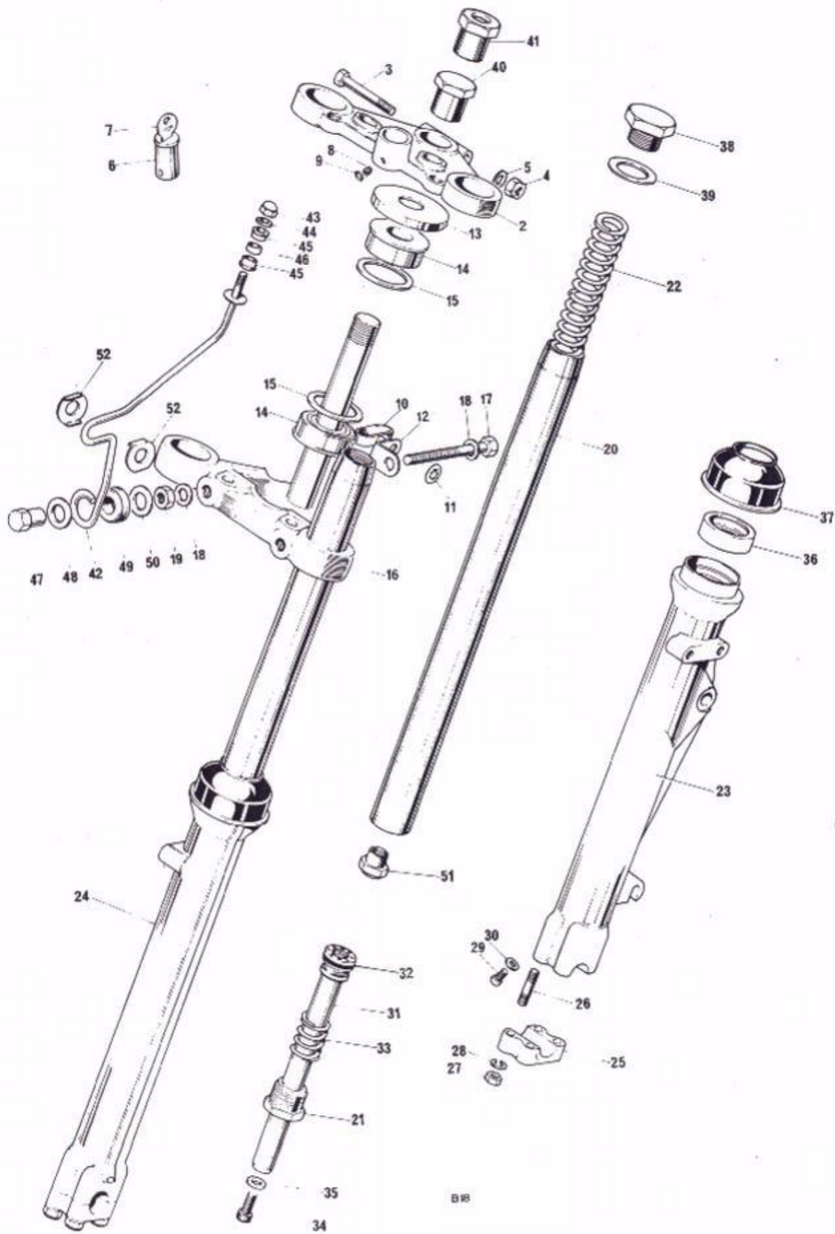
Fig. 19. TELESCOPIC FRONT FORK
