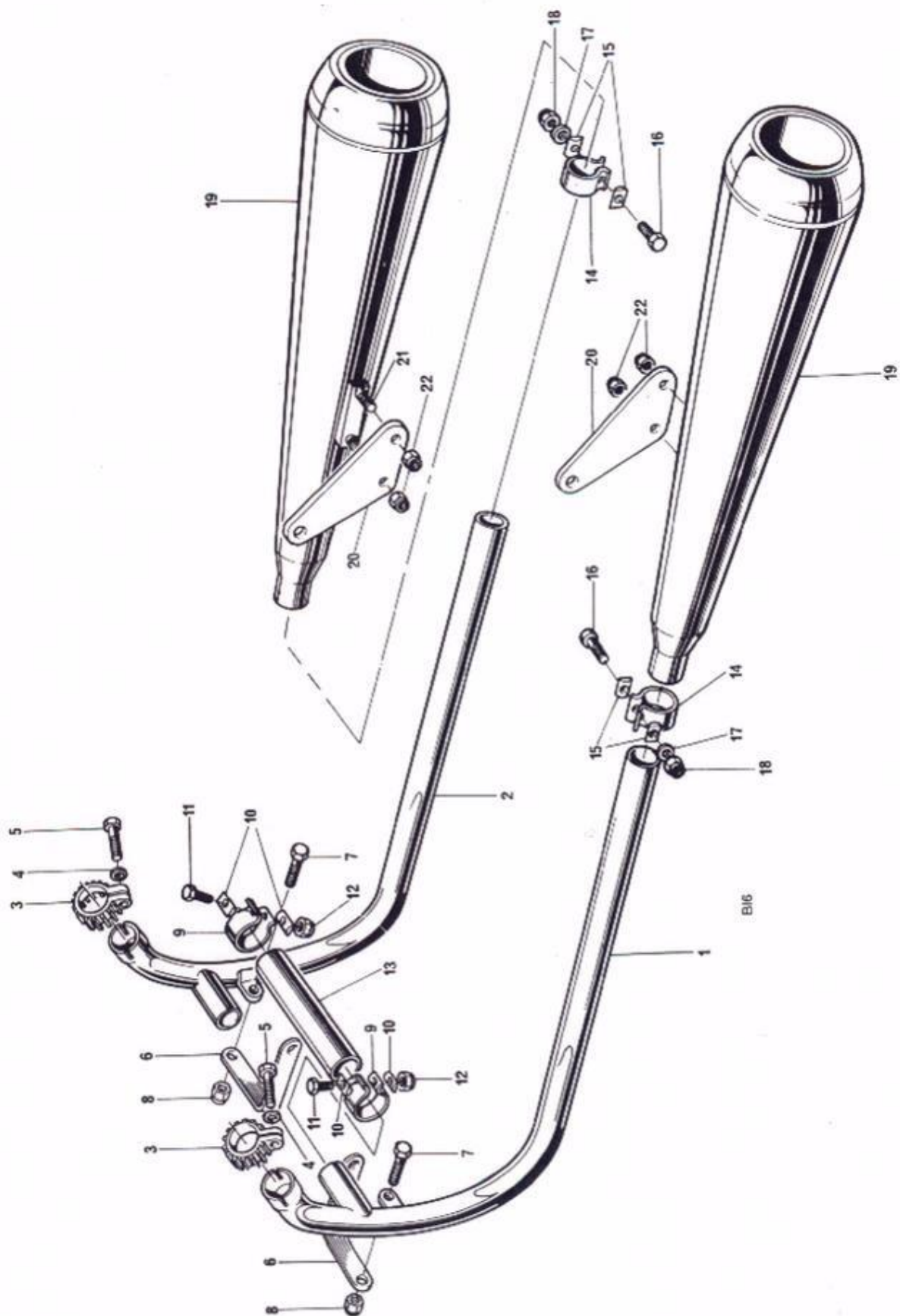
Fig. 17. EXHAUST PIPES AND MUFFLERS
