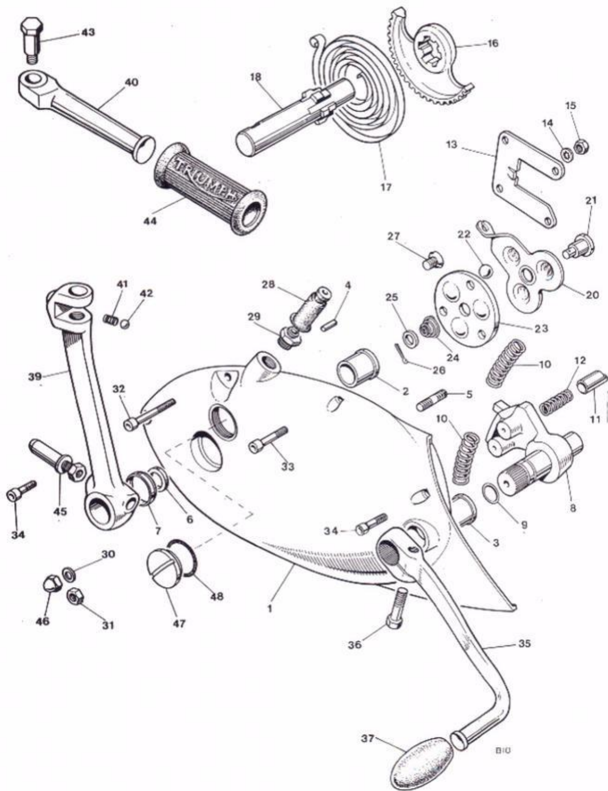
Fig 11. GEARBOX OUTER COVER
