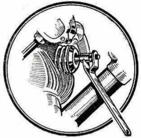
Fig. 8.—PUSH-ROD EXTRACTOR.
