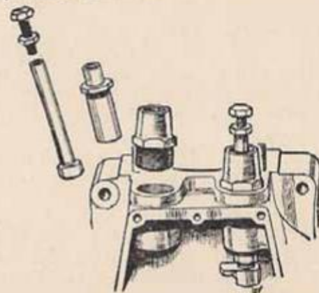
FIG. 53.—NEW OILTIGHT TAPPET GUIDES MADE IN TWO PARTS
