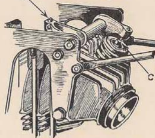
FIG. 34. SHOWING VALVE CLEARANCE ADJUSTMENT
