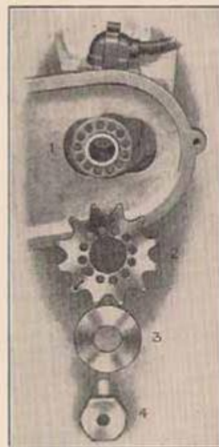
FIG. 44. THE VERNIER TIMING ADJUSTMENT
