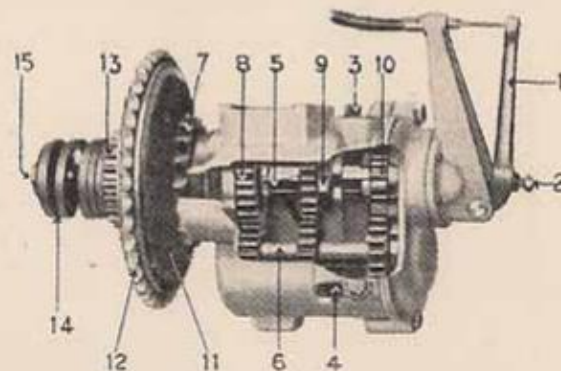
FIG. 31. THE A.J.S. GEAR-BOX
