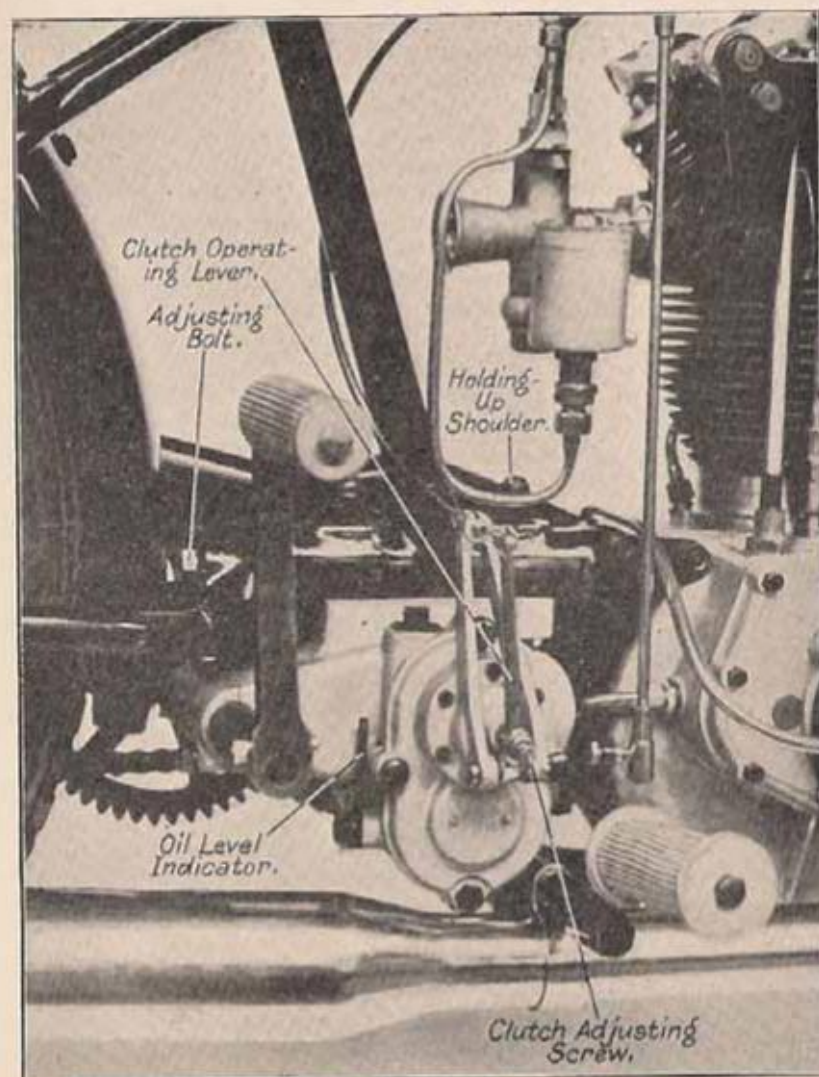
FIG. 48. SHOWING GEAR-BOX AND CLUTCH OPERATION This shows the 3-49 h.p. O.H.V. Model, but is identical on all other models
