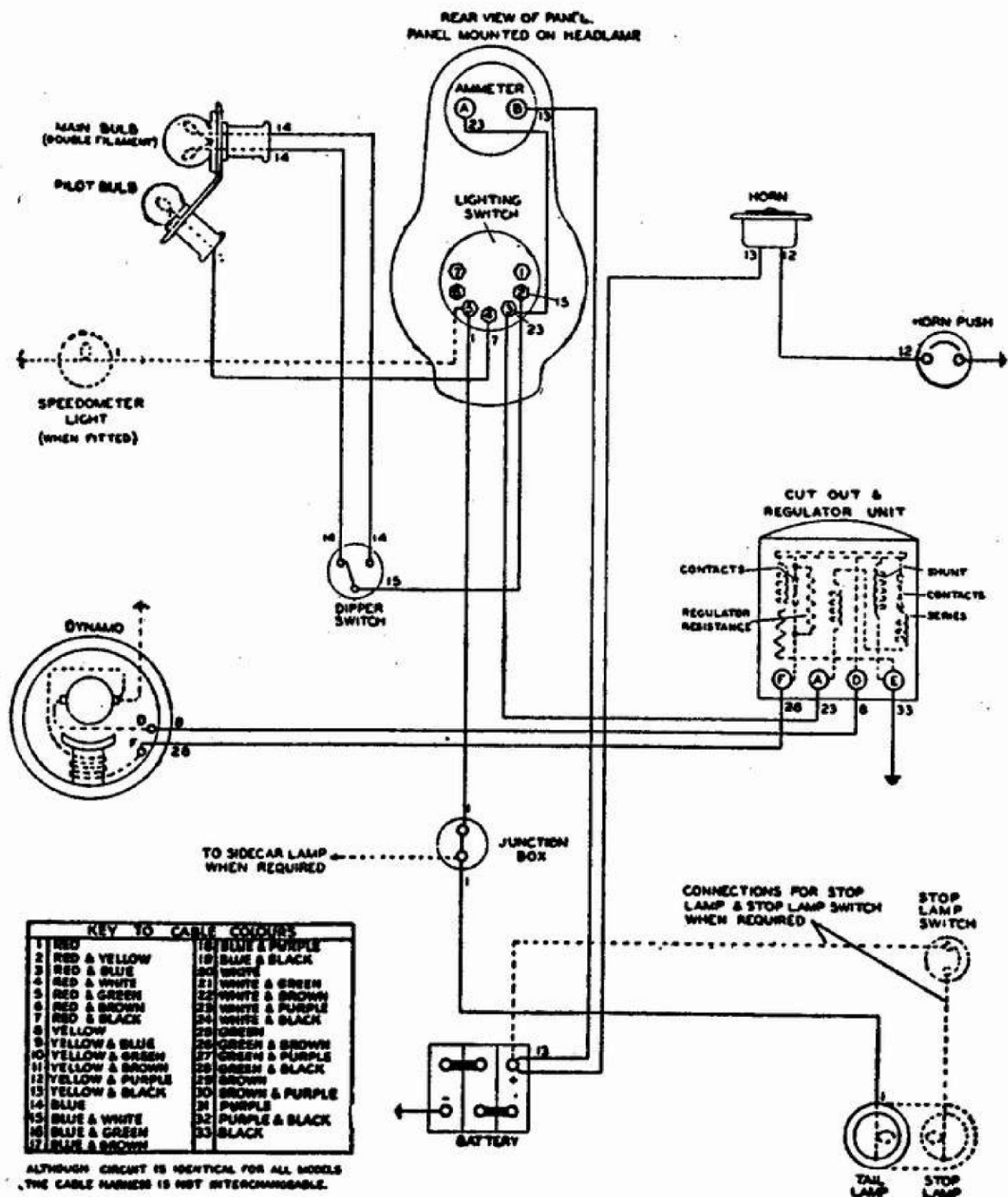
FIG. 55.—LUCAS MAGDYNO COMPENSATED VOLTAGE CONTROL EQUIPMENT AS FITTED TO ARIEL MOTOR CYCLES, 1937-50, EXCEPT TO THE 1949-1950 1000-C.C. MODELS WITH COIL IGNITION.
