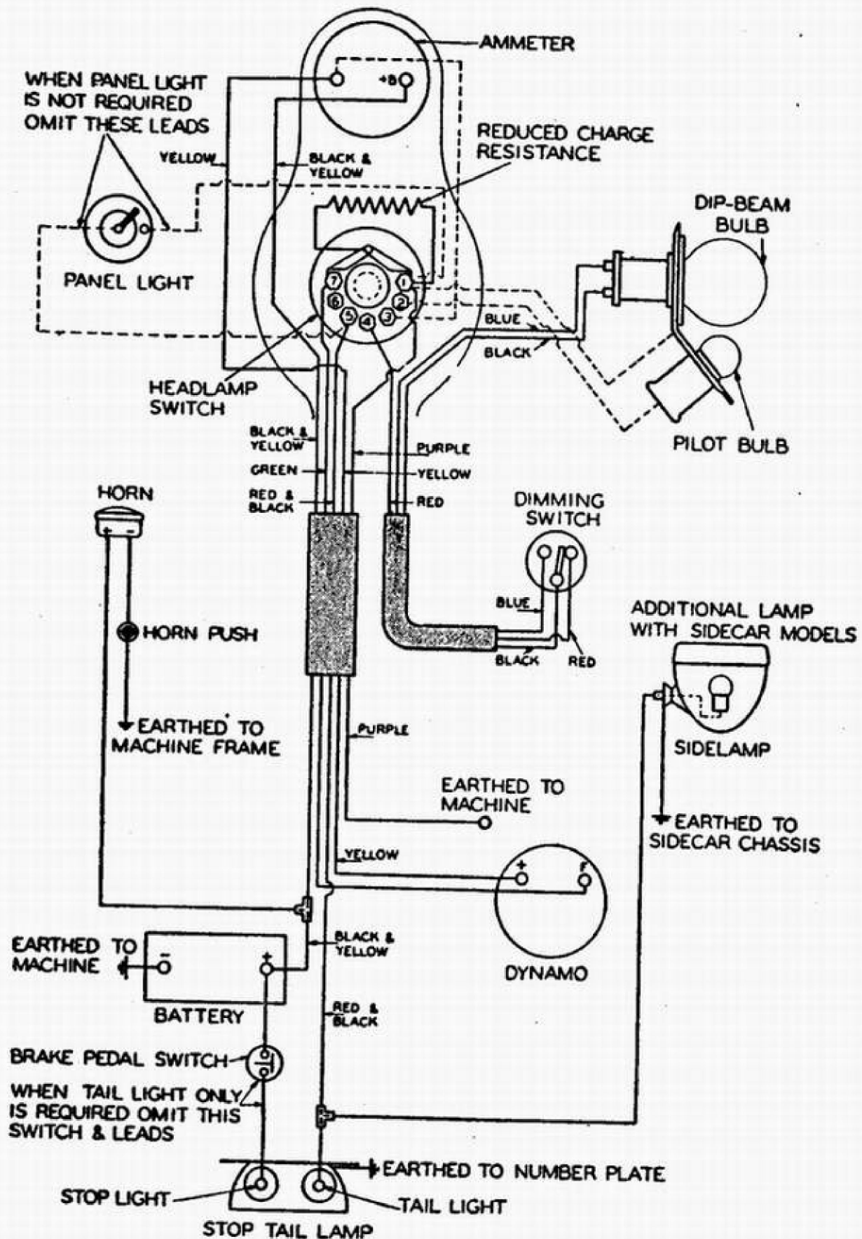
FIG. 52.—WIRING DIAGRAM FOR LUCAS MAGDYNO LIGHTING EQUIPMENT AS FITTED TO ARIEL MOTOR CYCLES, 1933-1936.
