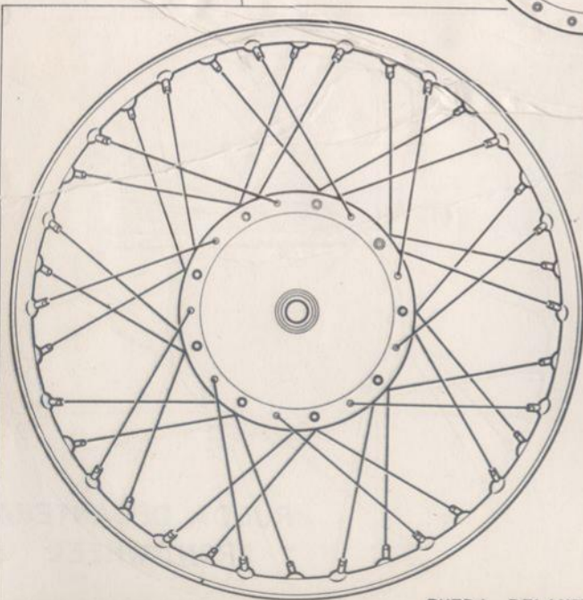
RUEDA DELANTERA FRONT WHEEL
