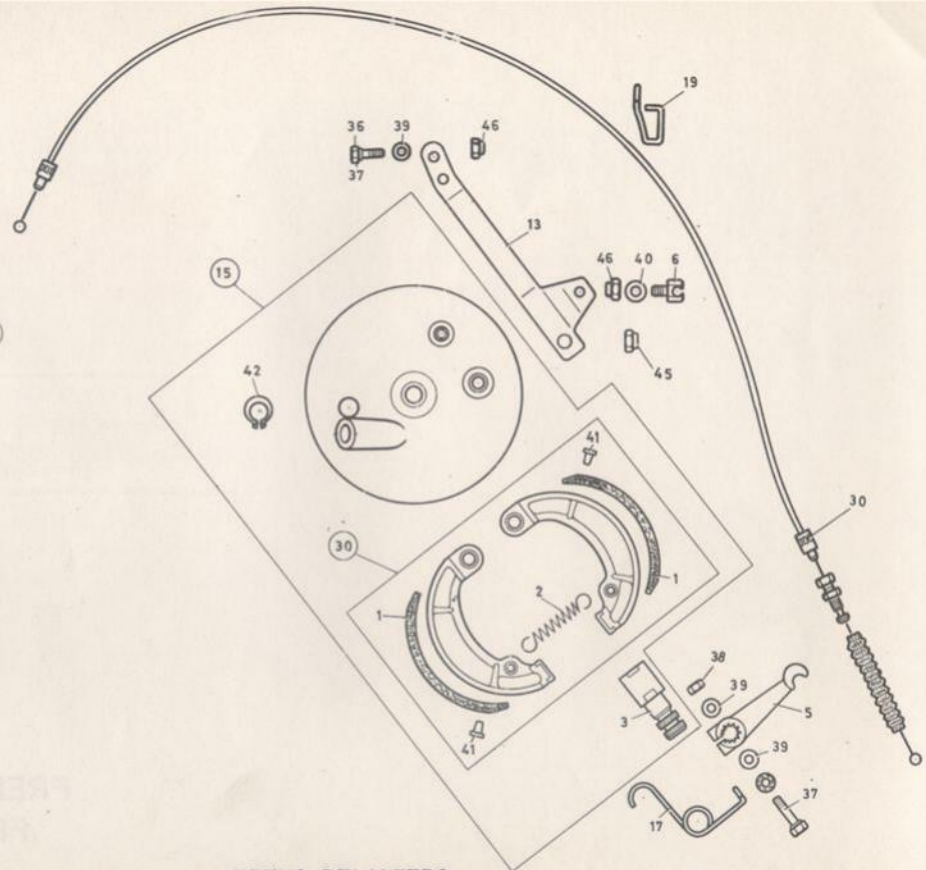
FRENO DELANTERO FRONT BRAKE
