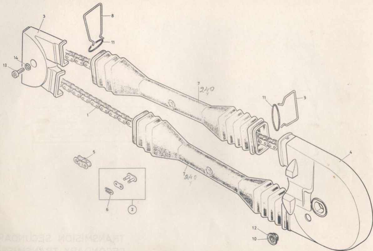
TRANSMISION SECUNDARIA SECONDARY TRANSMISSION
