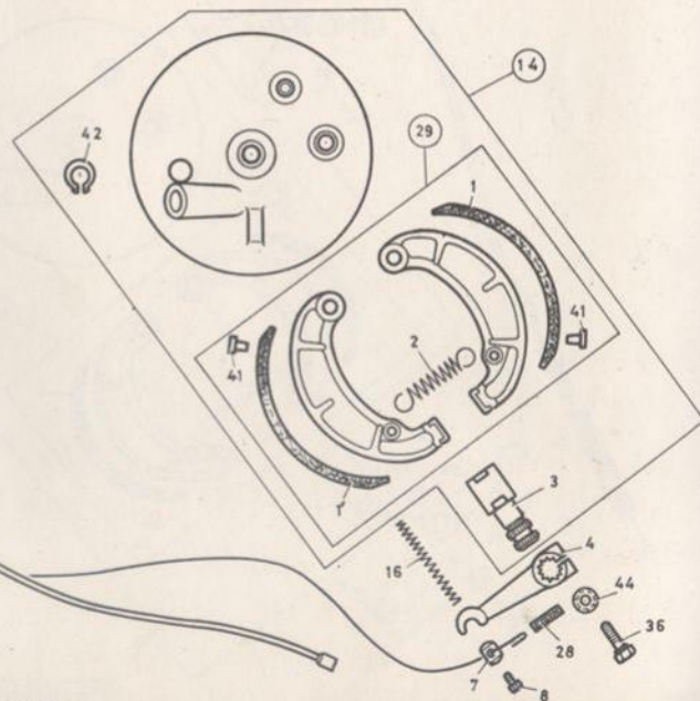
FRENO DELANTERO FRONT BRAKE
