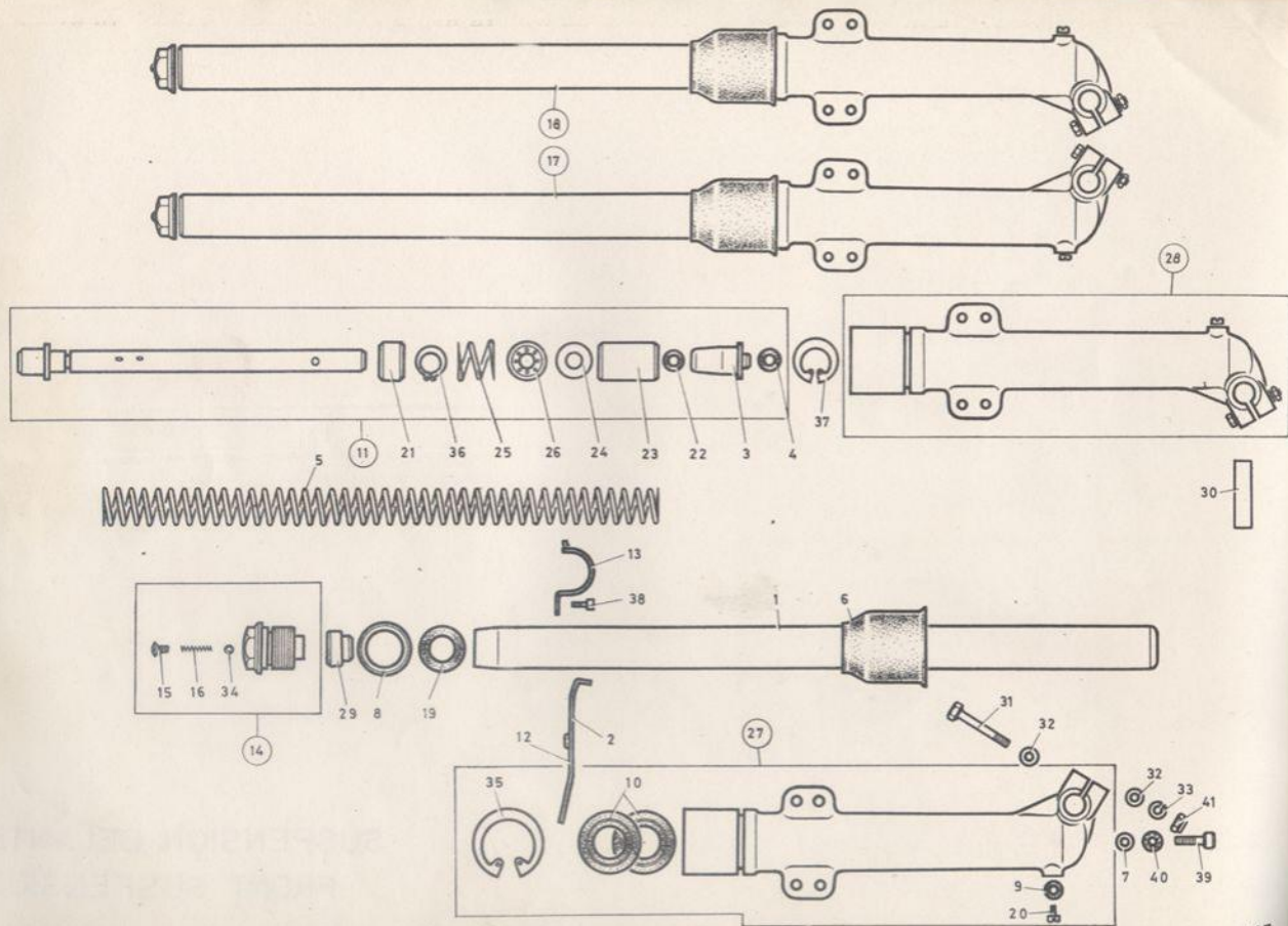
SUSPENSION DELANTERA FRONT SUSPENSION
