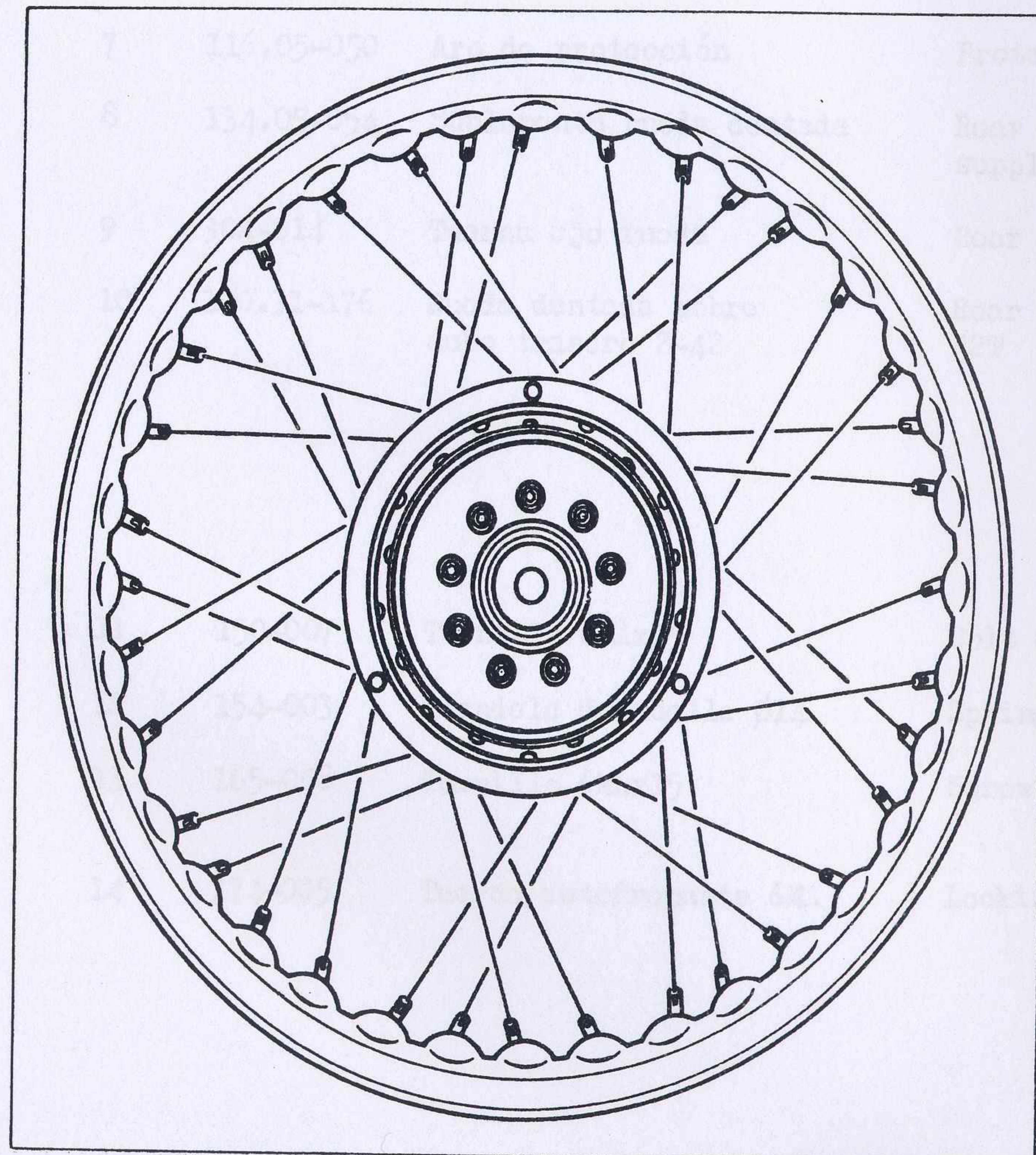
RUEDA TRASERA REAR WHEEL
