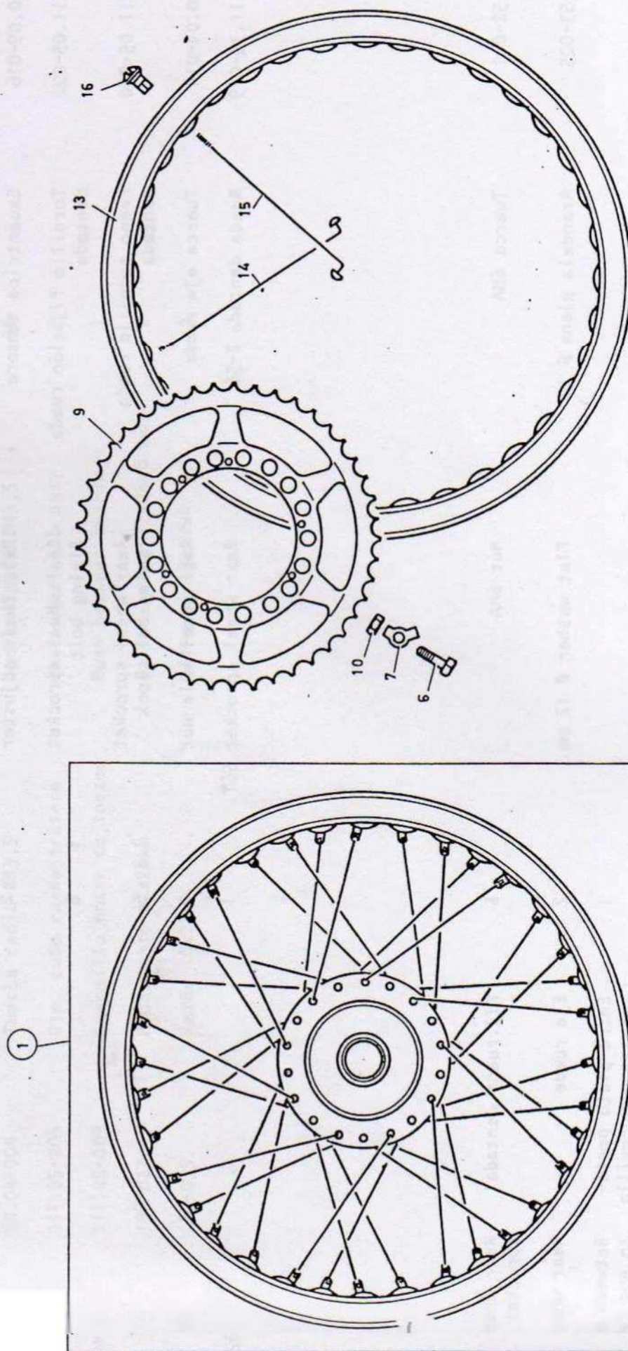
RUEDA TRASERA REAR WHEEL
