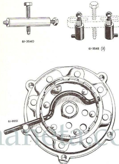
Fig. Z6. Flywheel Removal Tools.
