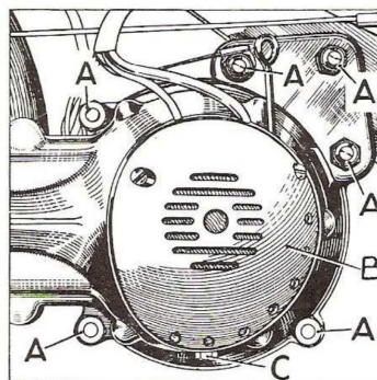
Fig. Z2. Removing Engine.
