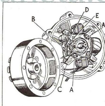
Fig. Z3. Generator (Wico)
