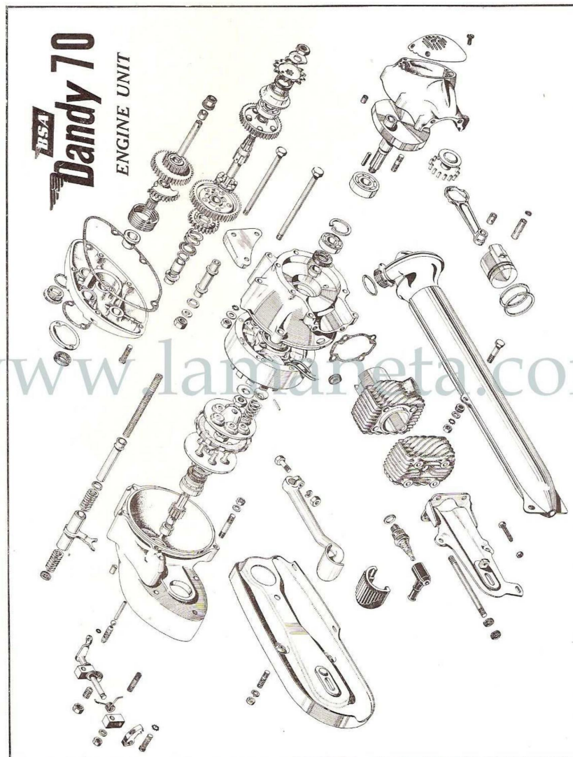
The DANDY Engine and Gearbox (Exploded View)
