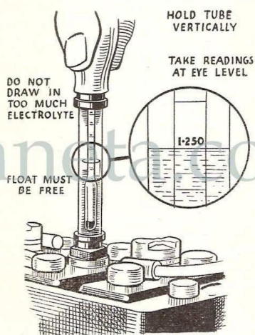
Fig Y20. Taking hydrometer readings
