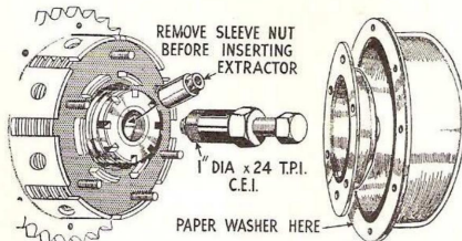
61-1912 Clutch Extractor Tool
