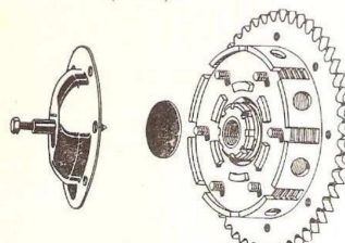
61-3055 Clutch Testing Tool
