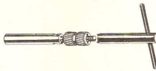
61-3284 Mainshaft Bush Reamer 61-3285 Pilot for Jigs 61-3275 61-3286 Pilot for Jigs 61-3281 61-3287 Shell Reamer Holder 61-3288 Tommy Bar for 61-3287
