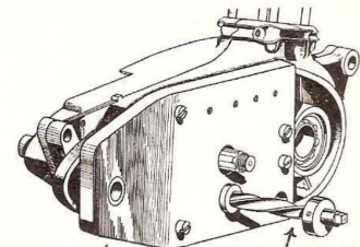
Service Tool 61-3199. 61-3308 Reamer for 61-3199 Line Reaming the Gearbox Bushes
