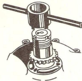
61-3220 Cush Drive Nut Tube Spanner (used with 61-699)
