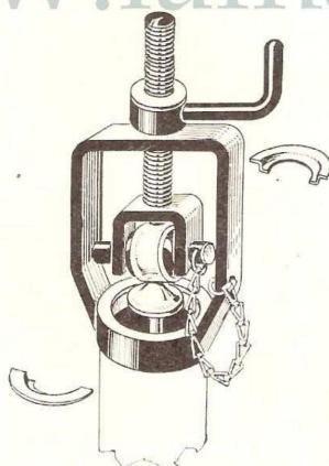
61-3503 Rear Suspension Dismantling Tool
