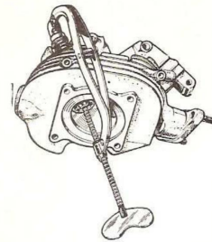
61-3340 Valve Spring Compressor with Adaptor Models M33 "B" Group, "A" Group, and Sunbeam
