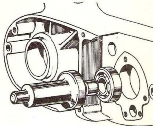
61-3214 Ballrace Pilot (gearbox pinion bearing)
