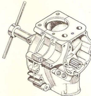
61-1932 Reamer and Holder complete (mainshaft bush) 61-1922 Reamer for 61-1932
