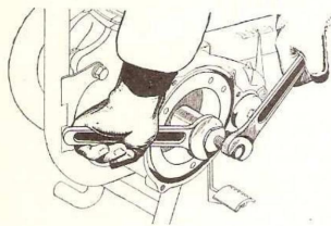
61-3188 Generator Flywheel Removal Tool (Wico Paco) 90-297 Generator Flywheel Removal Tool (Lucas)
