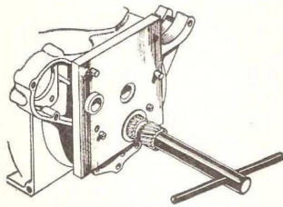
61-3281 Reaming Jig (mainshaft and timing gear bushes) 61-3275 Reaming Jig (mainshaft and timing gear bushes) 61-3162 Reaming Jig (timing gear bushes only)
