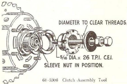
61-3306 Clutch Assembly Tool
