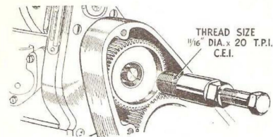
61-1903 Magdyno Driving Pinion Extractor Tool complete.
