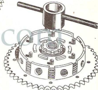
61-1915 Clutch Spring Nut Tube Spanner.
