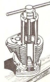
61-1937 Tool for inserting and removing Barrel Liners
