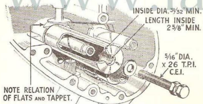
61-691 Cam Pinion Post Extractor
