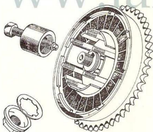
61-3362 Clutch Extractor Tool
