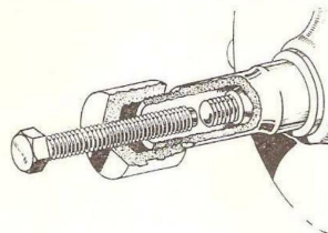
61-3365 Cush Drive Extractor
