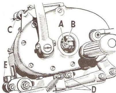
Fig. M32 (a). Clutch Adjustment.
