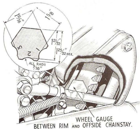
Fig. M35. Wheel alignment gauge.
