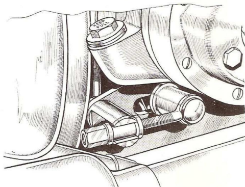
Fig. M33. Front chain adjuster.
