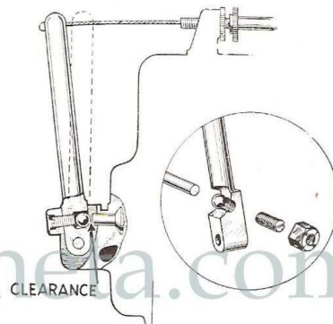
Fig. M32. Clutch control adjustment.
