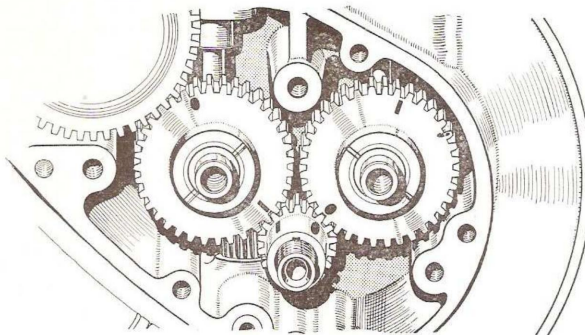
Fig. M23. Valve timing marks.
