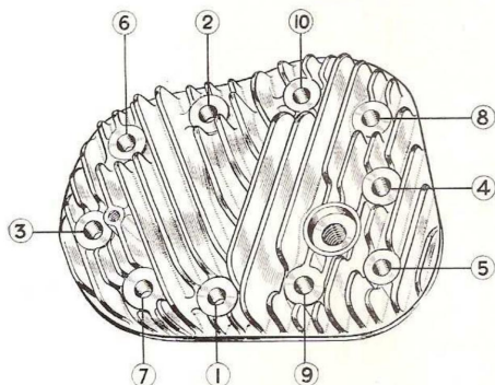
Fig. M24. Cylinder head bolts.
