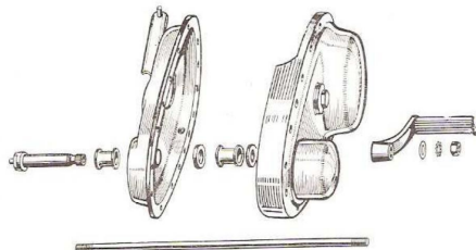
Fig. M25. Assembly of chaincase and footrest.
