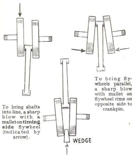
To bring flywheels parallel when sides opposite crankpin are converging insert wedge as shown and deal sharp blow with mallet.
