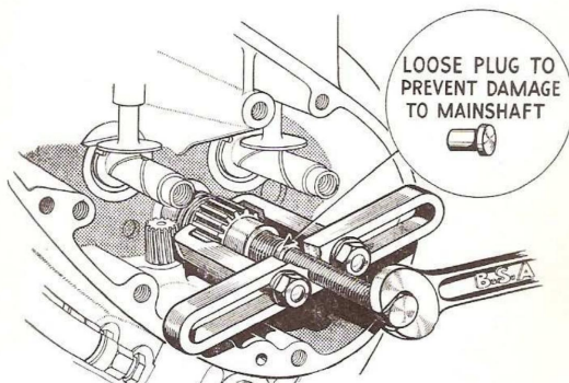
Fig. M16 Engine shaft pinion extractor 61-1735.
