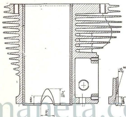
Two scoops diametrically opposite, ground after liner is pressed in.
