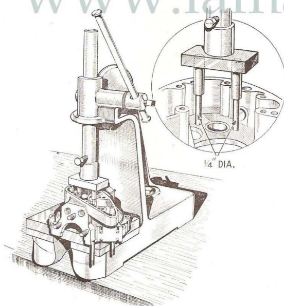
Fig. M18. Ballrace extraction (gearside).
