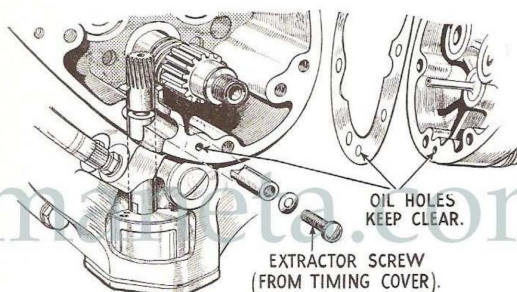
Fig. M17. Oil pump spindle locking plunger.
