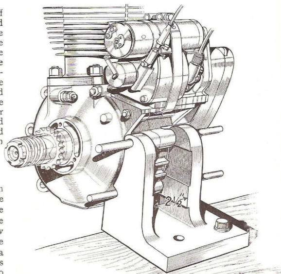
Fig. M15. Angle bracket for mounting engine.
