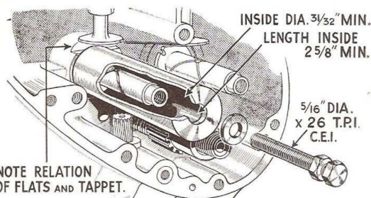
Fig. M20. Cam pinion spindle extractor 61-691.
