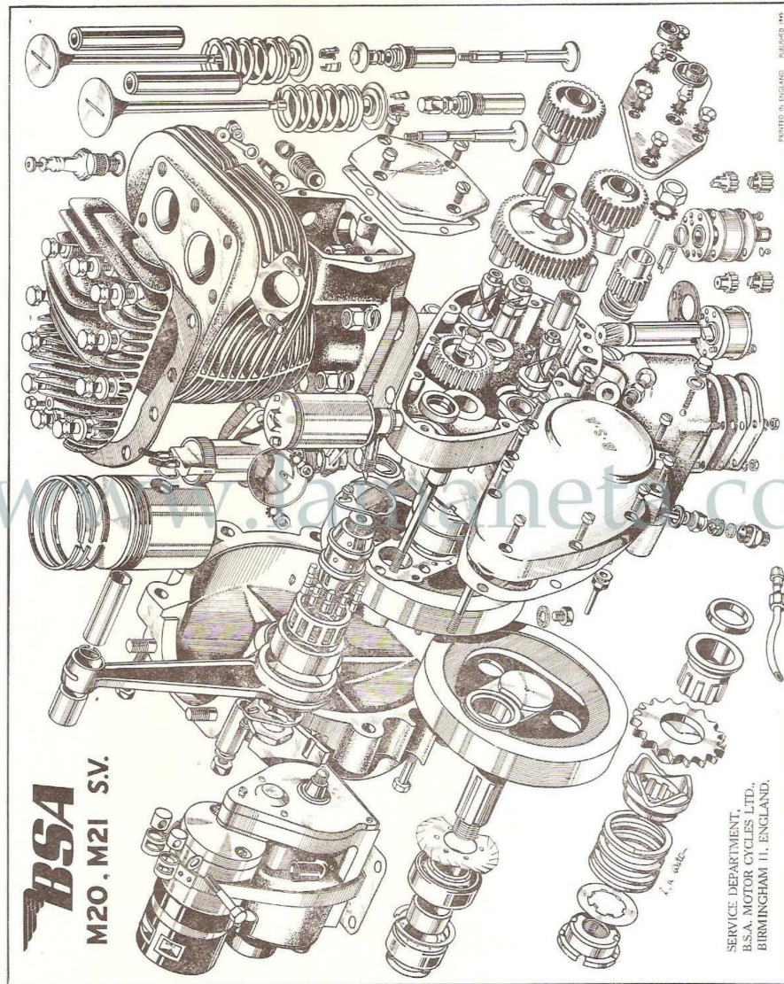
Fig. M1. M20—M21 Engine (Exploded View)
