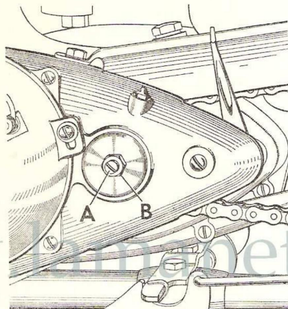
Fig. D 21.—Clutch control adjustment
